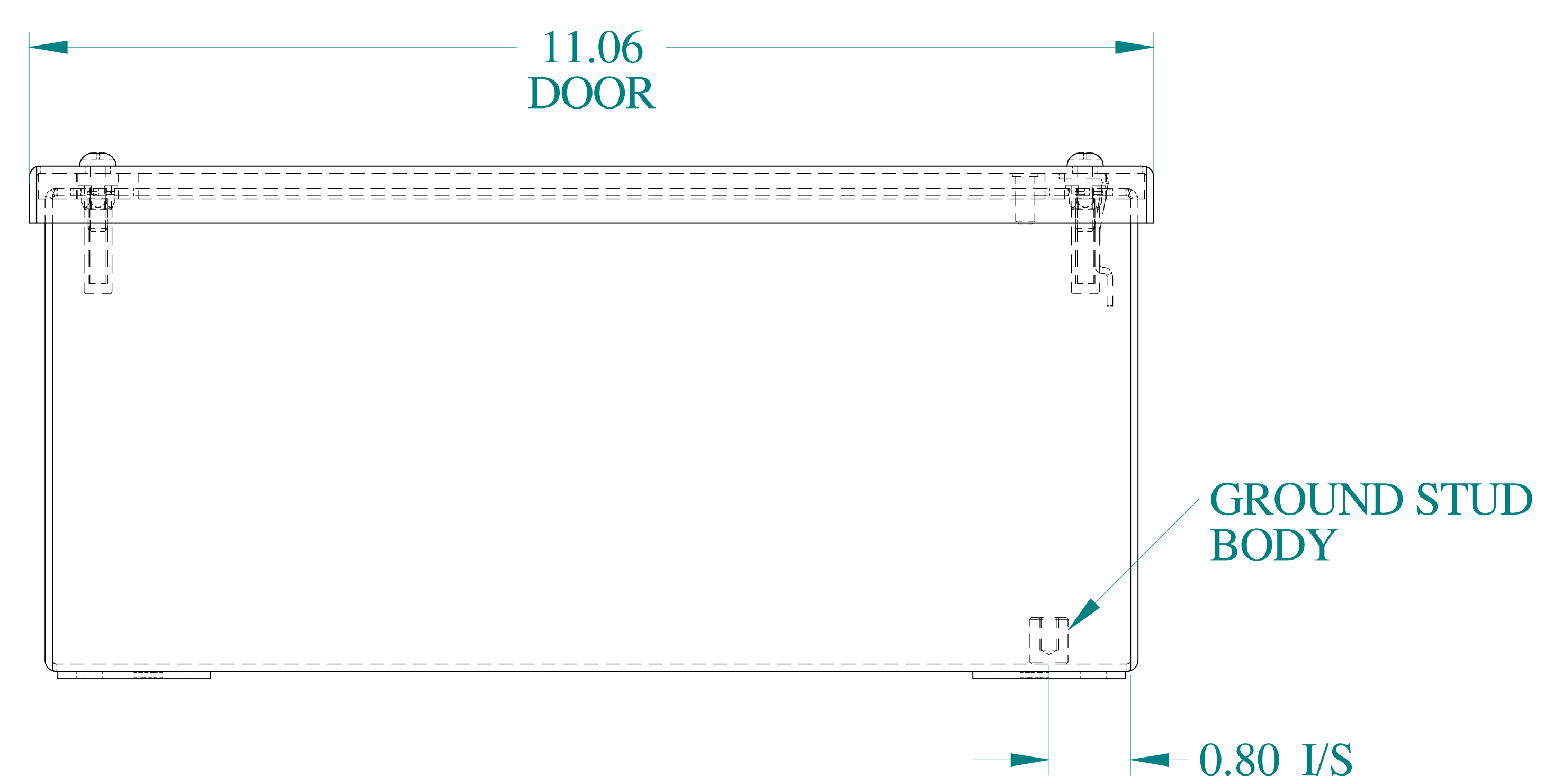
BOTTOM VIEW
