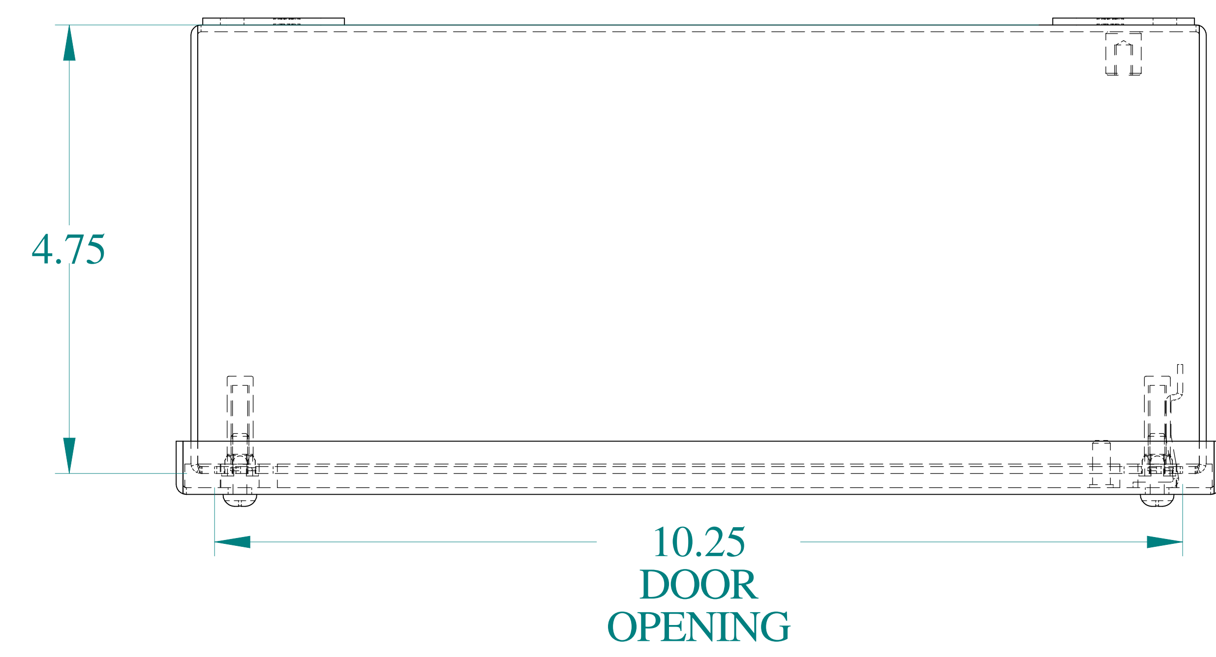
TOP VIEW
