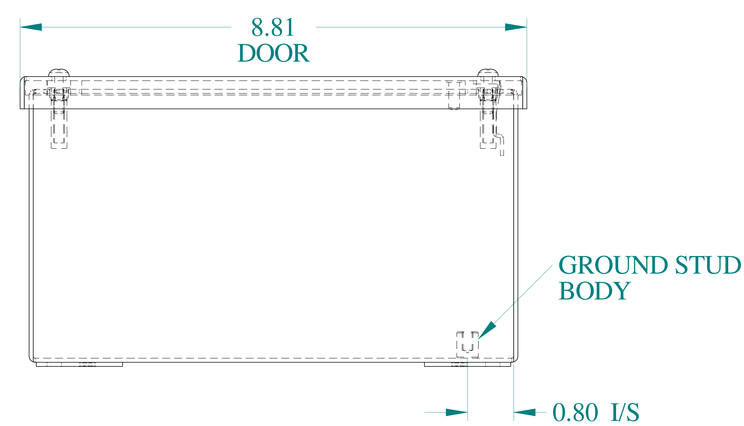
BOTTOM VIEW
