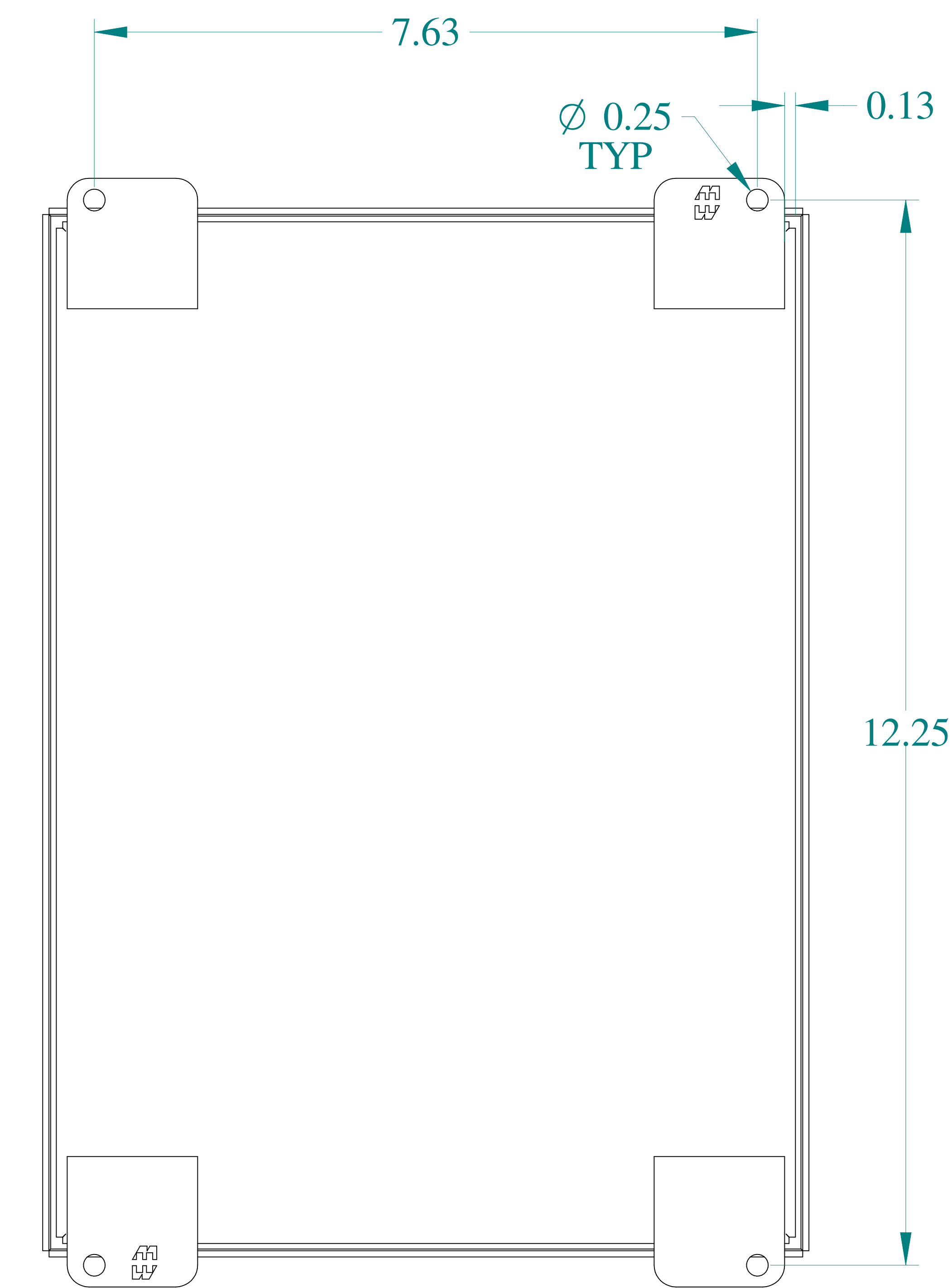
BACK VIEW
