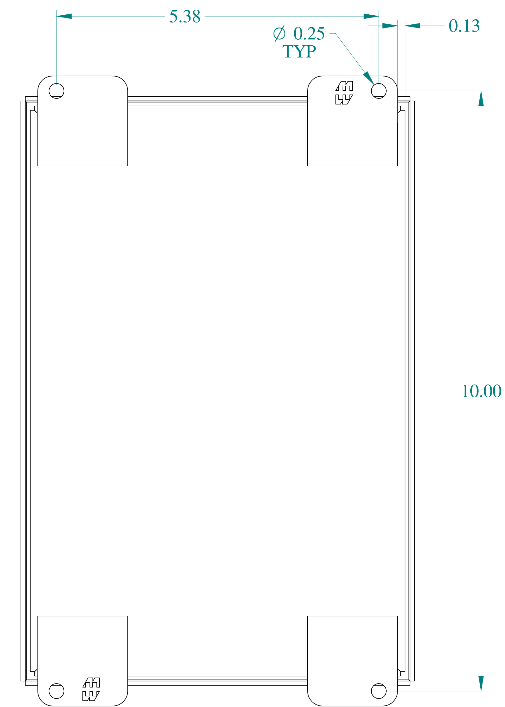
BACK VIEW
