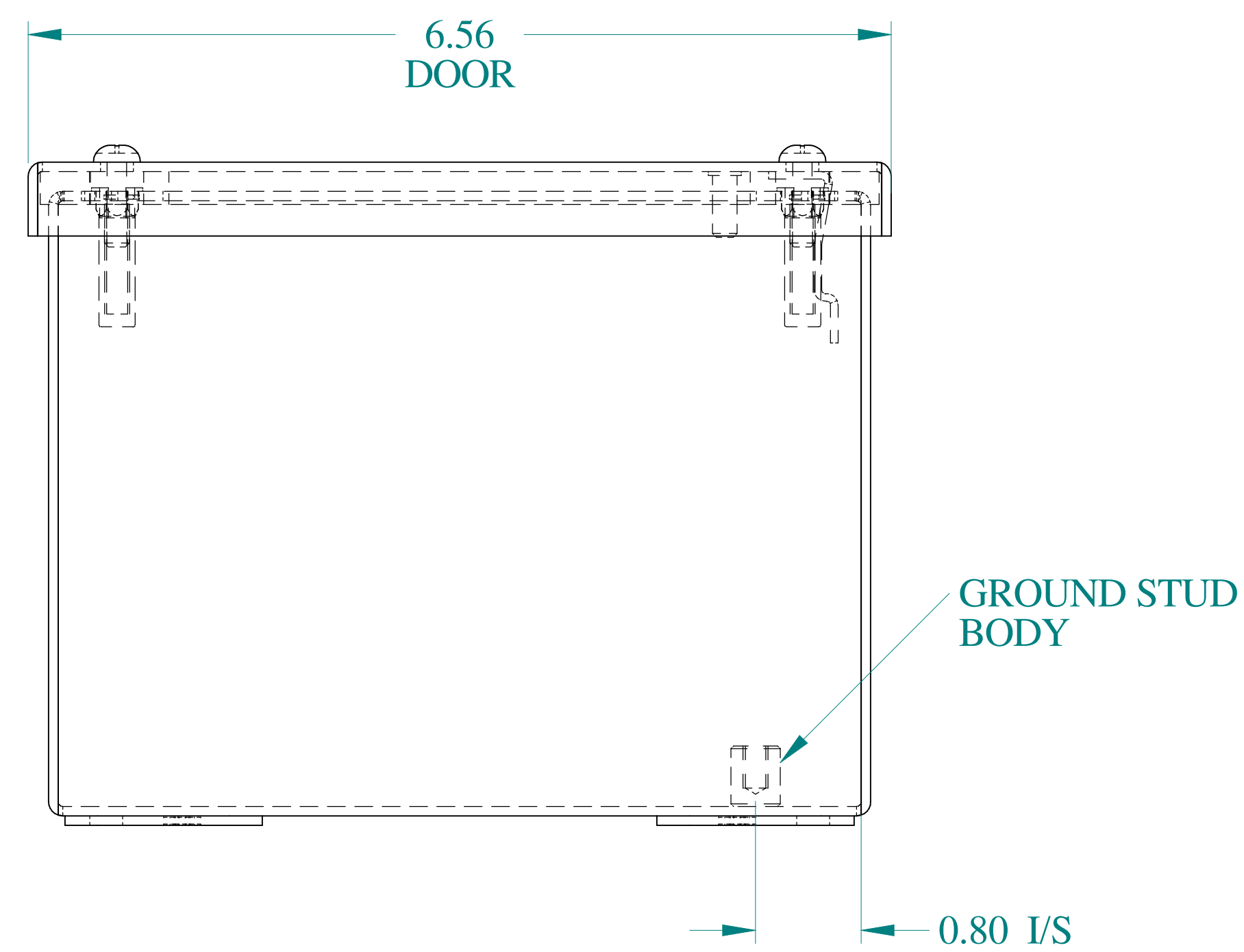
BOTTOM VIEW
