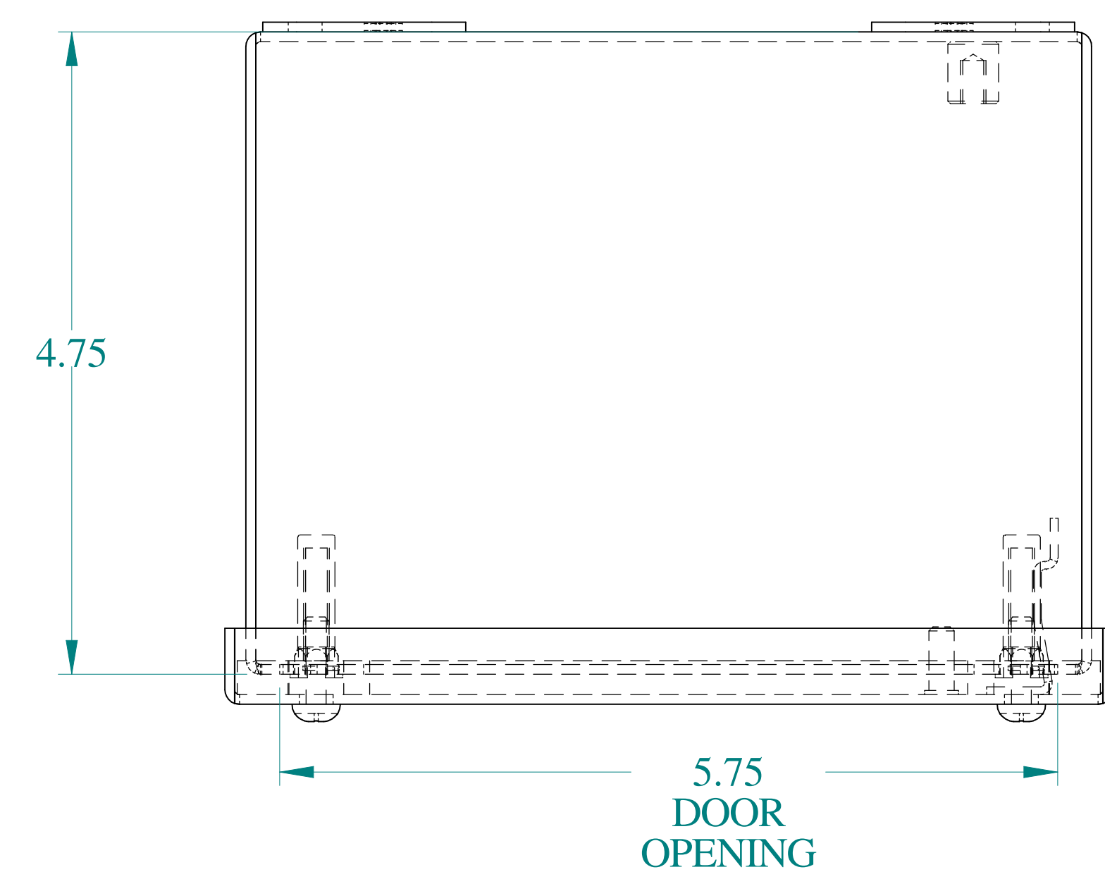
TOP VIEW
