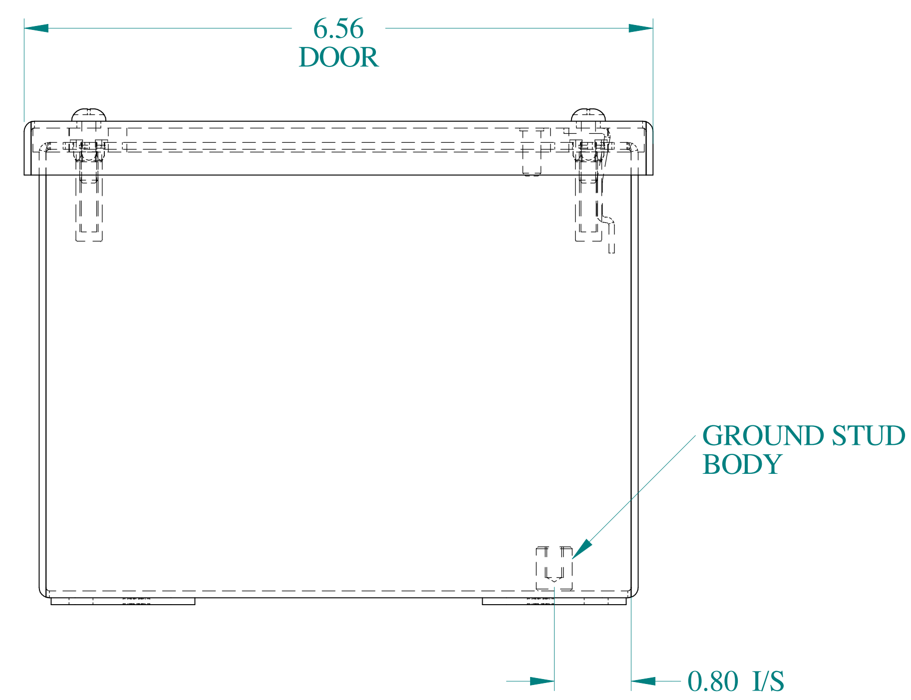
BOTTOM VIEW
