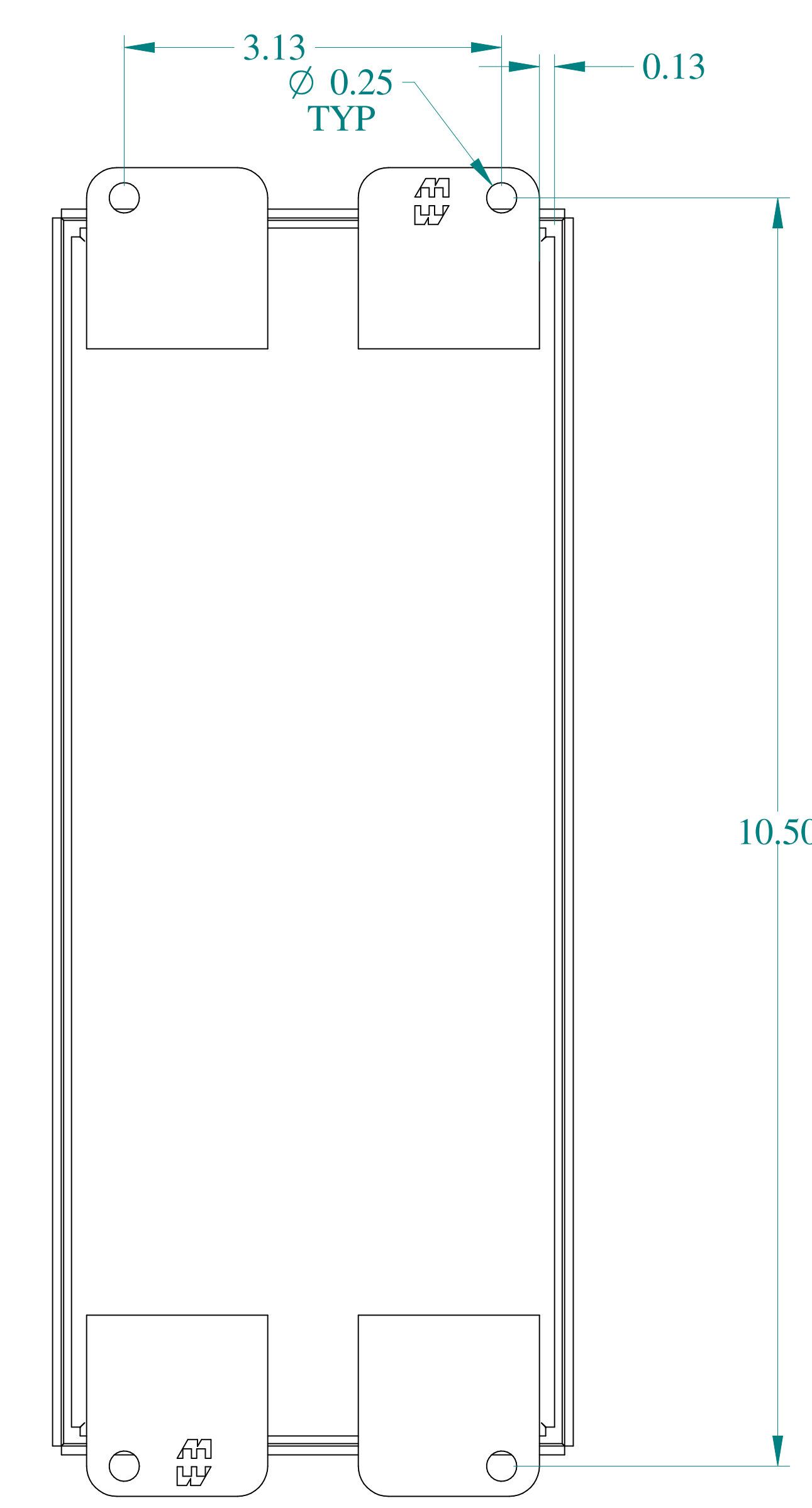
BACK VIEW
