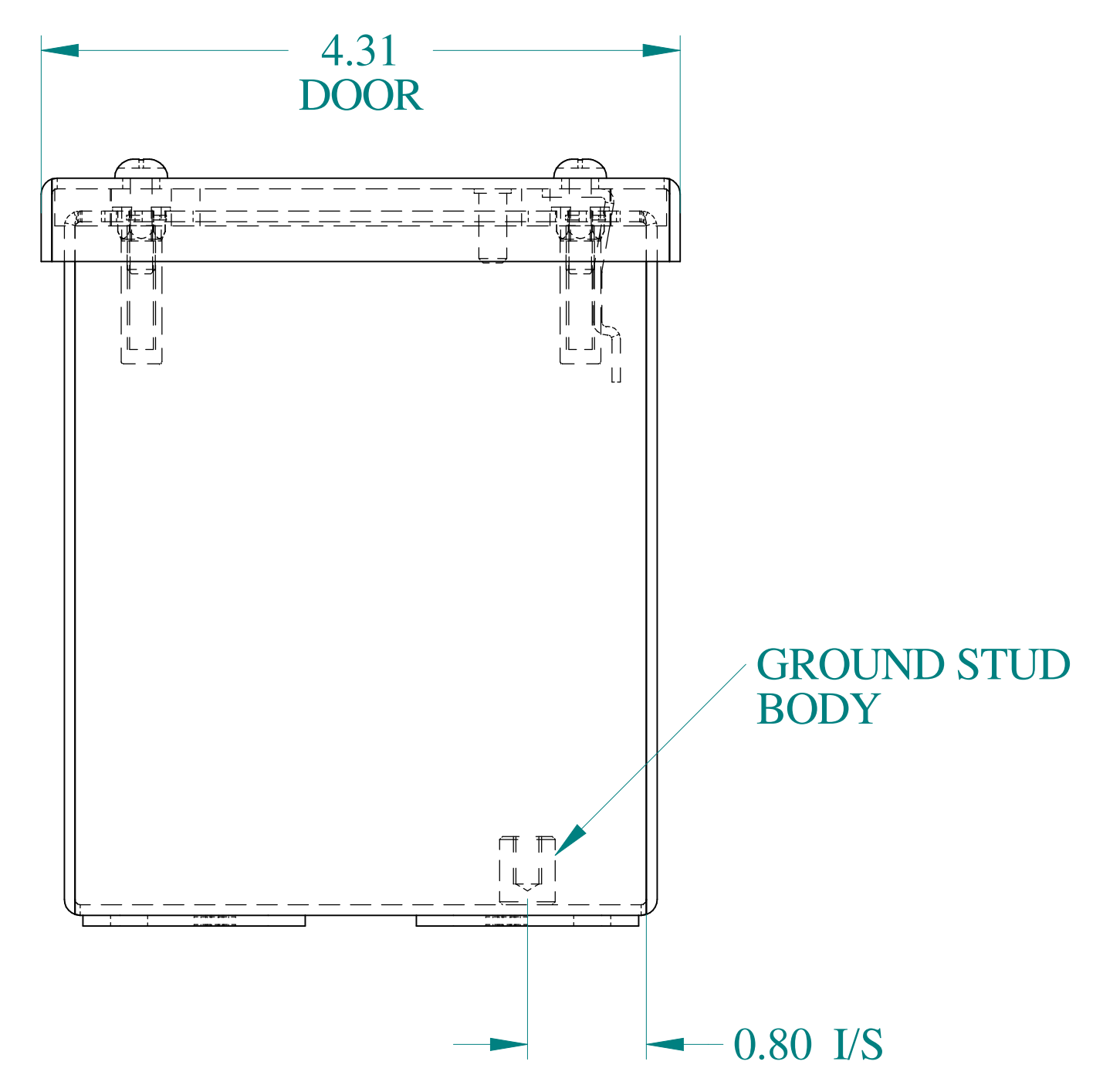
BOTTOM VIEW
