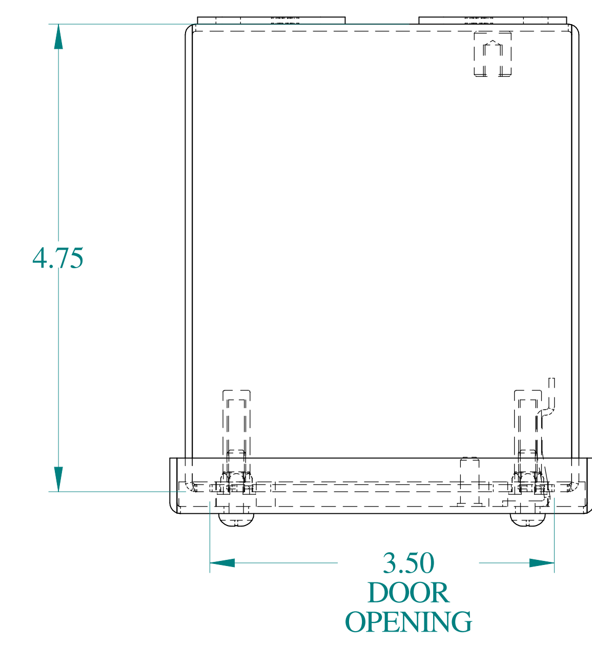
TOP VIEW
