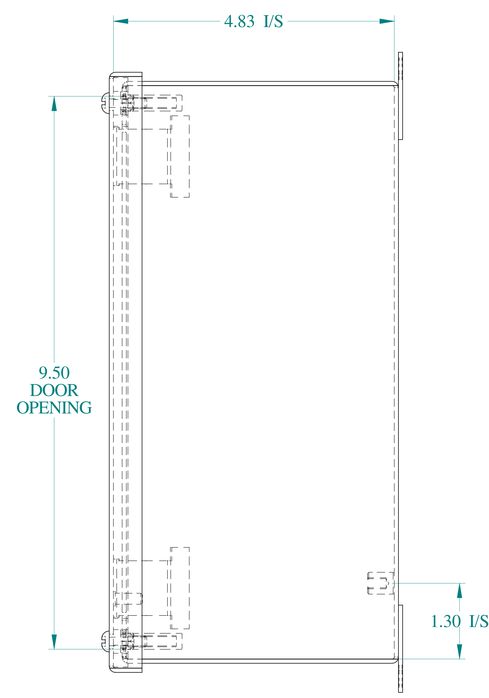
SIDE VIEW
