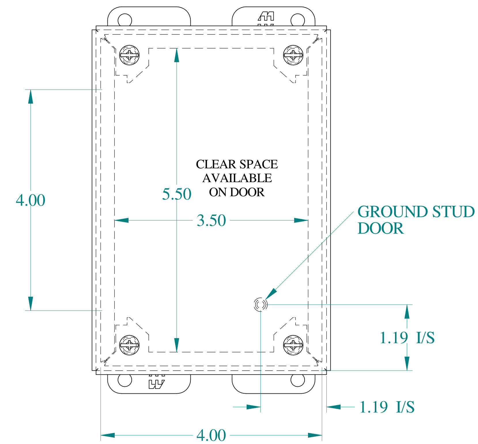
FRONT VIEW
