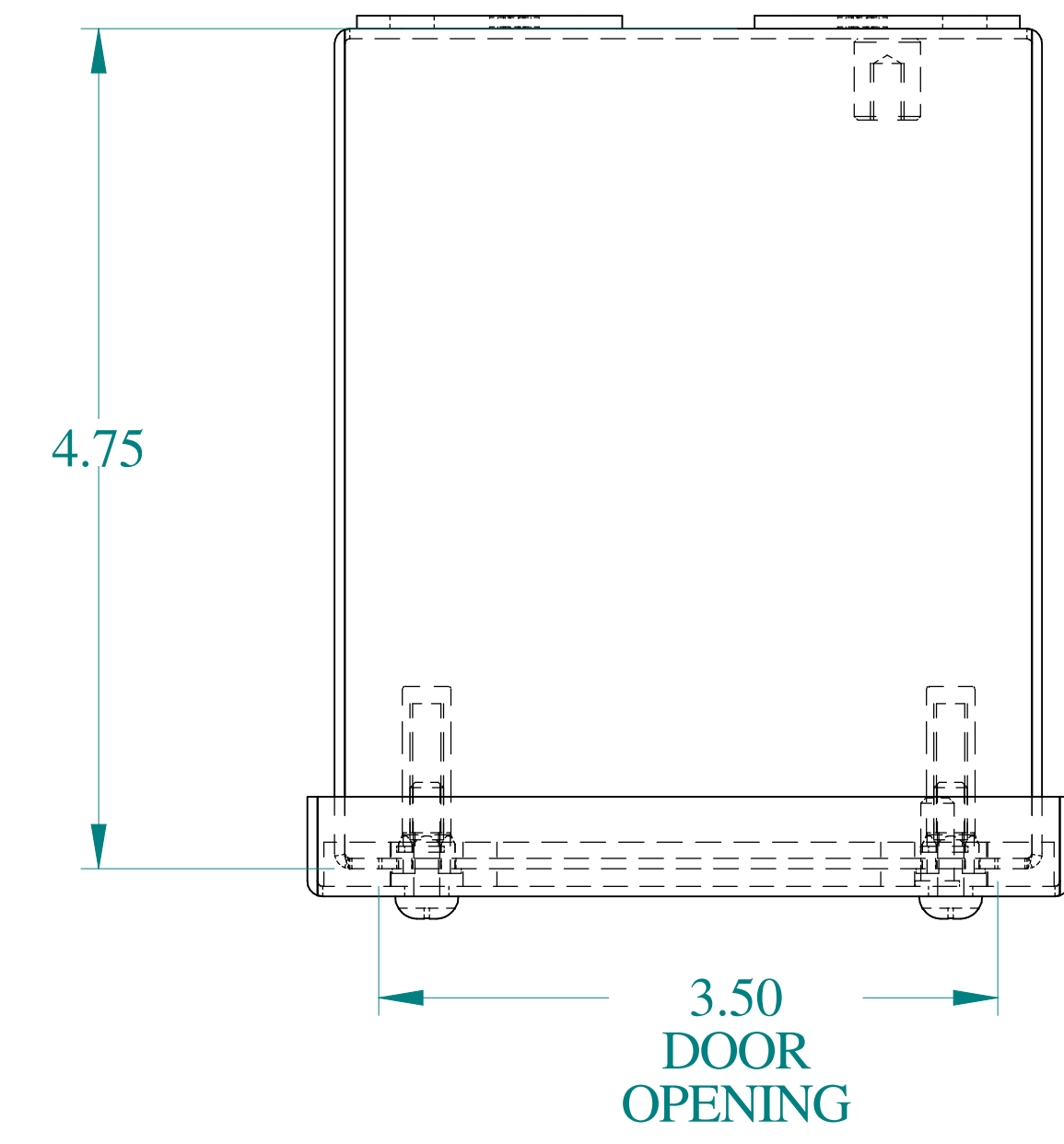
TOP VIEW
