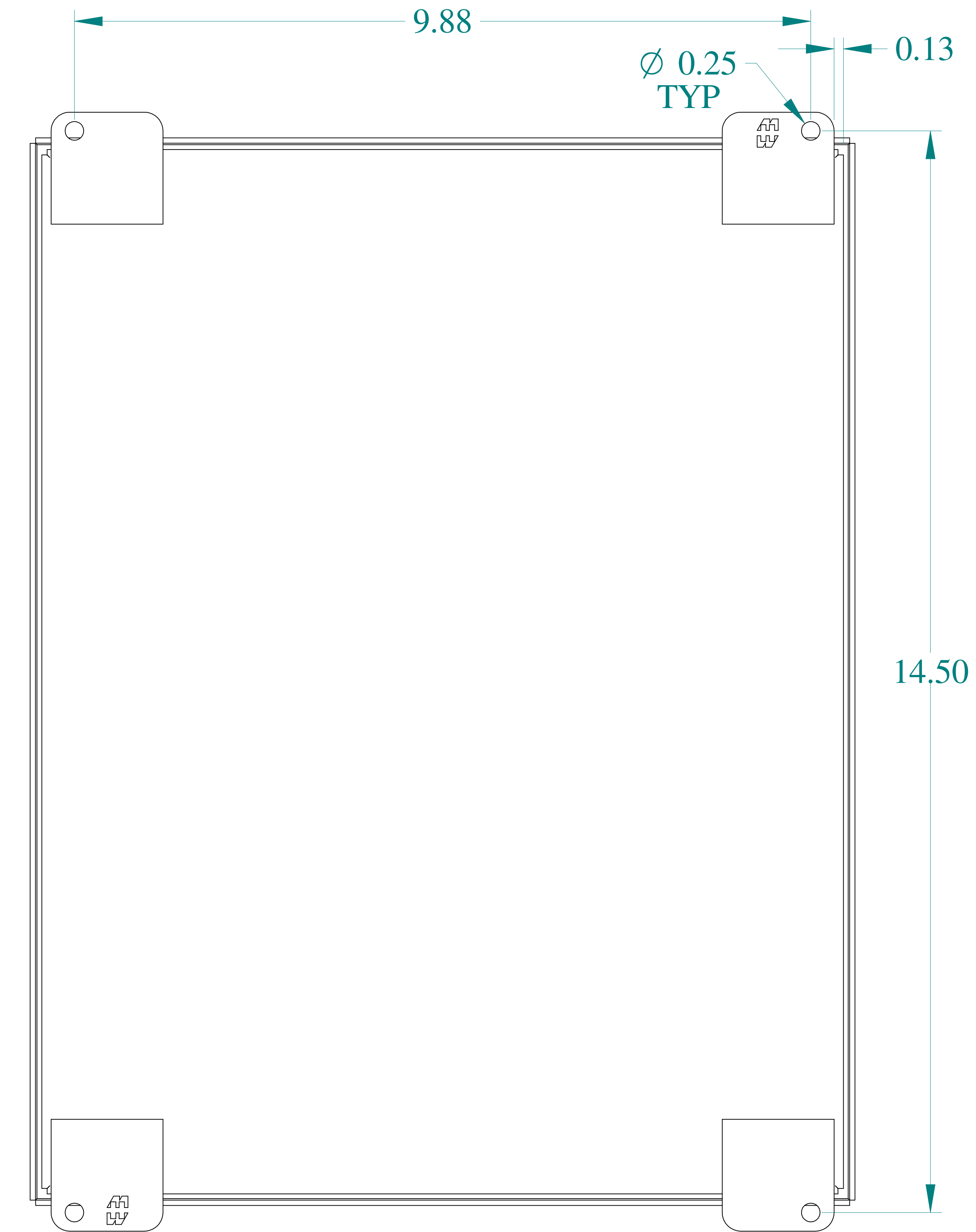
BACK VIEW
