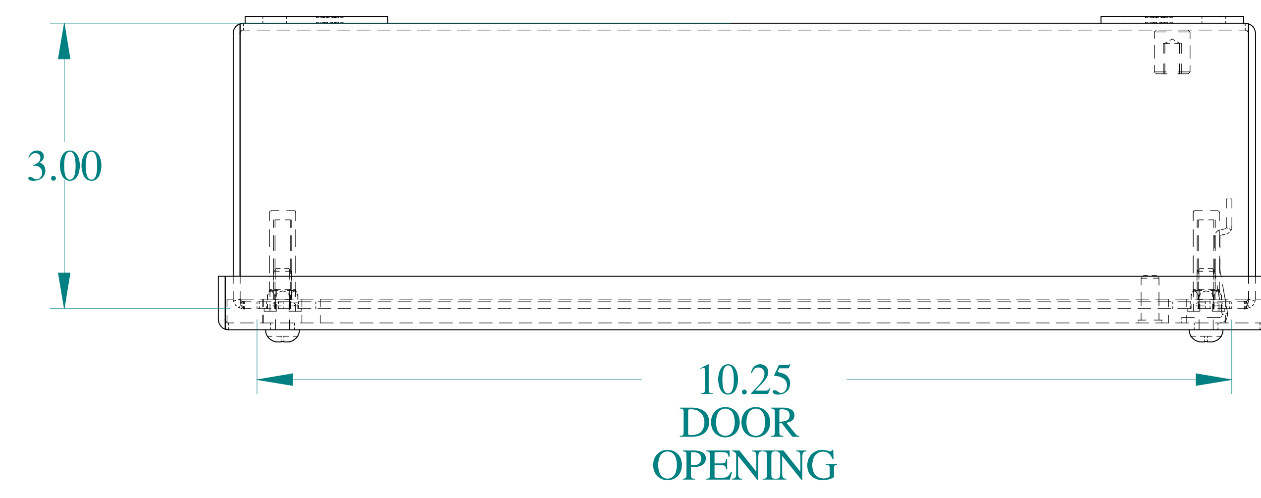
TOP VIEW
