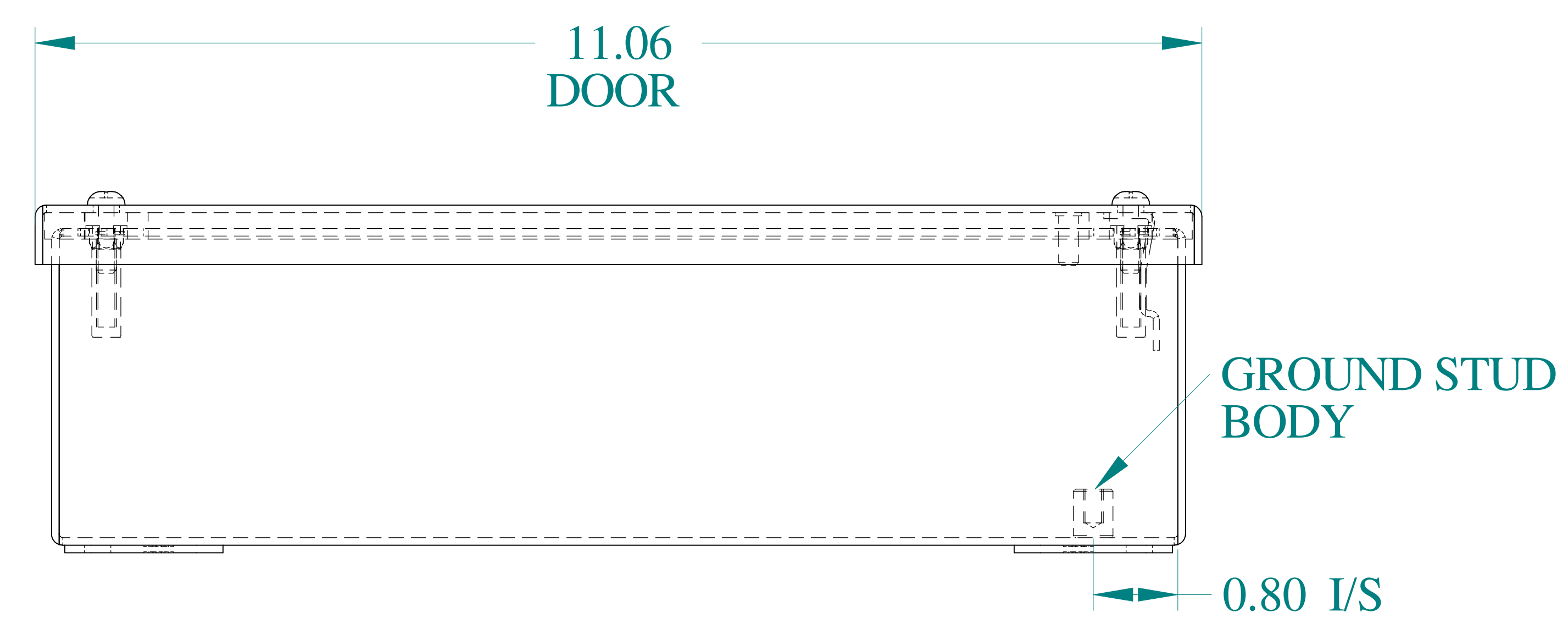
BOTTOM VIEW
