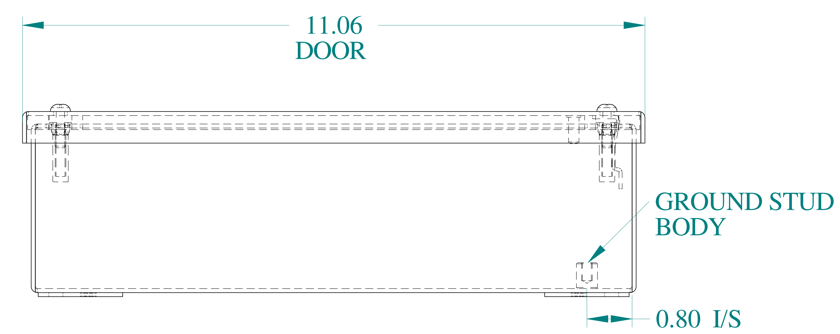
BOTTOM VIEW
