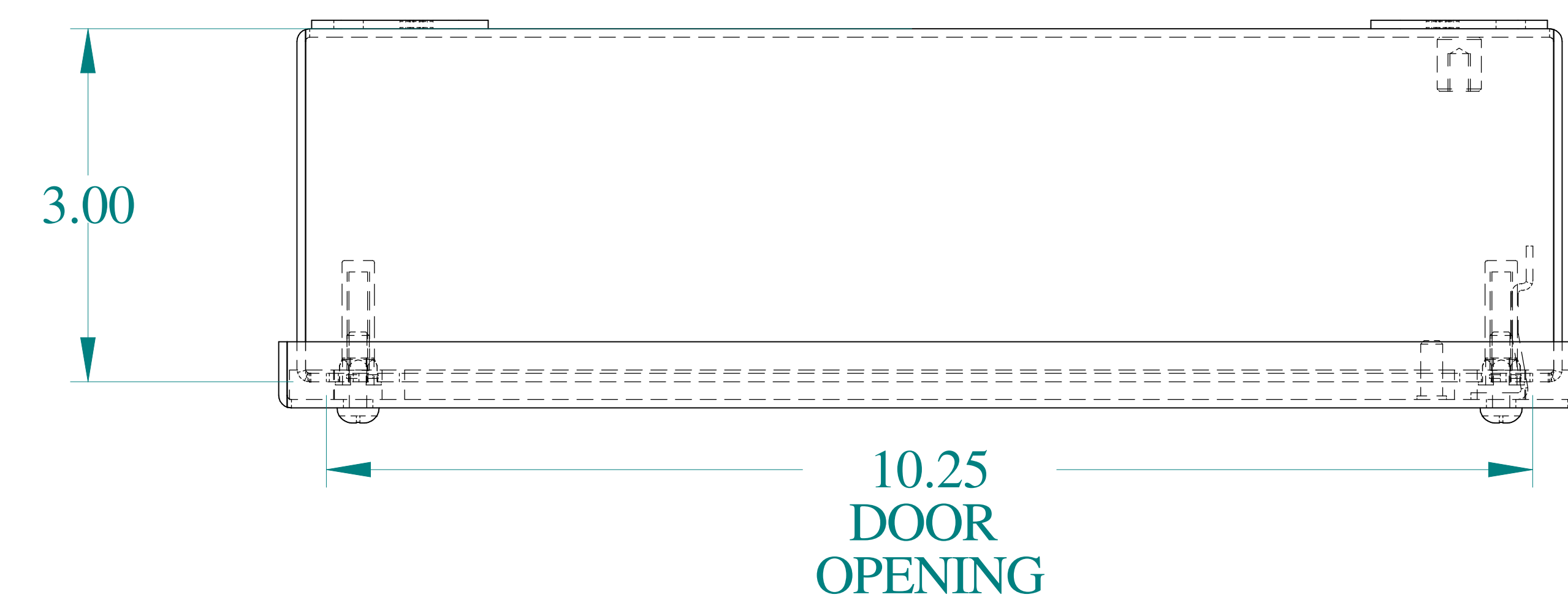
TOP VIEW
