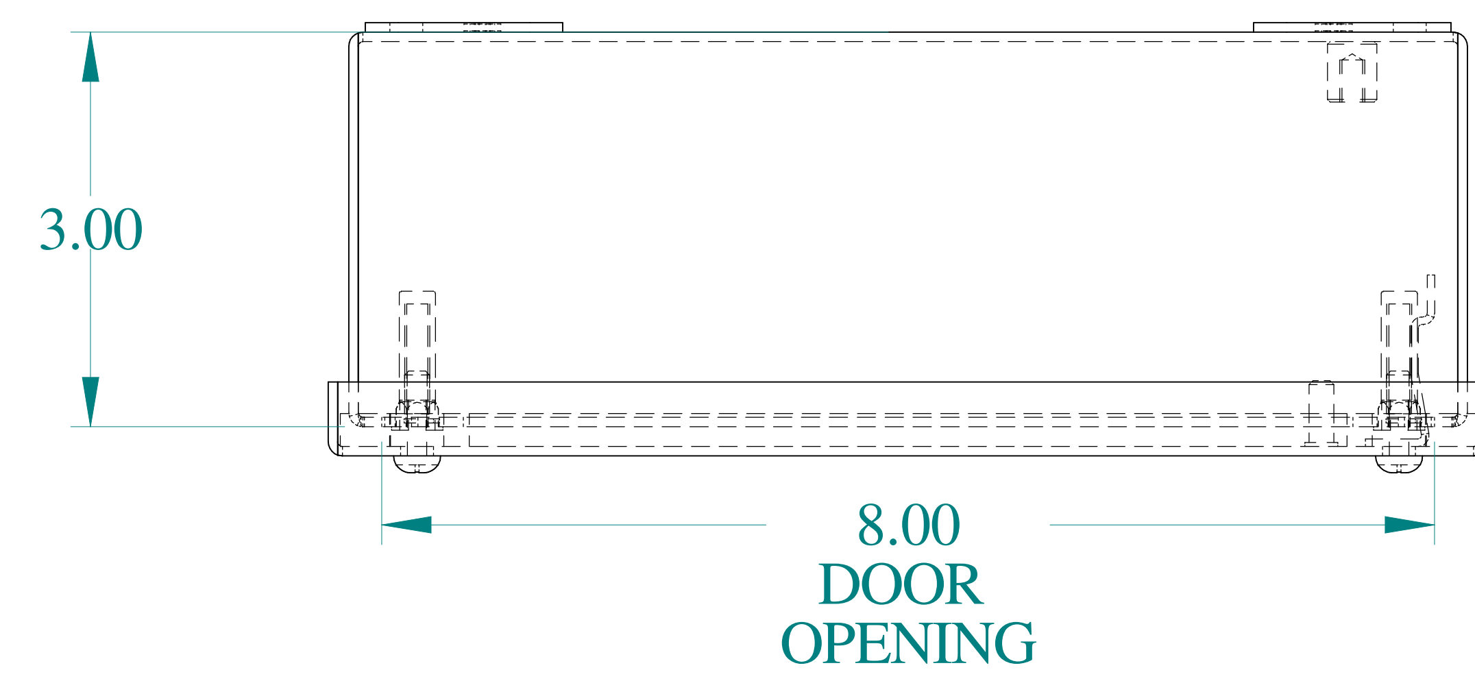
TOP VIEW
