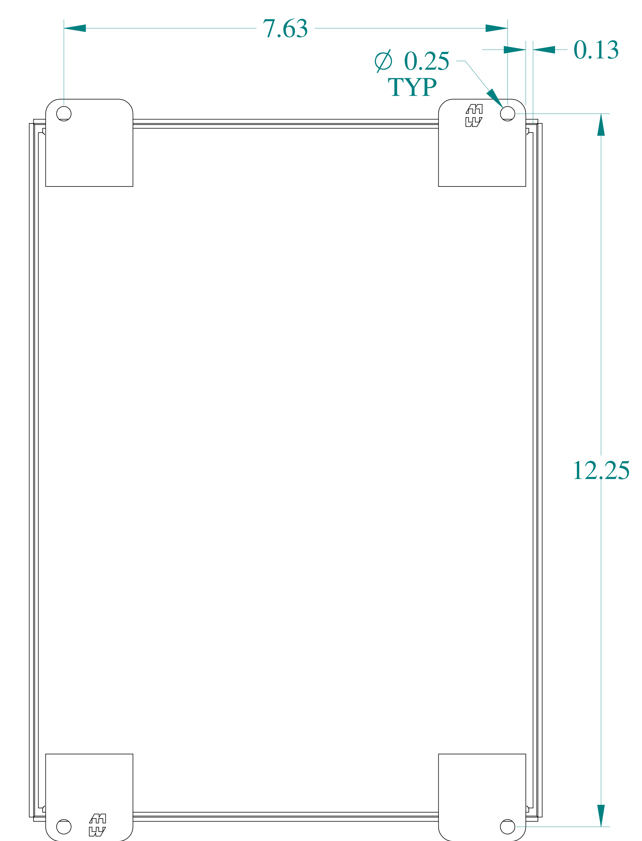
BACK VIEW
