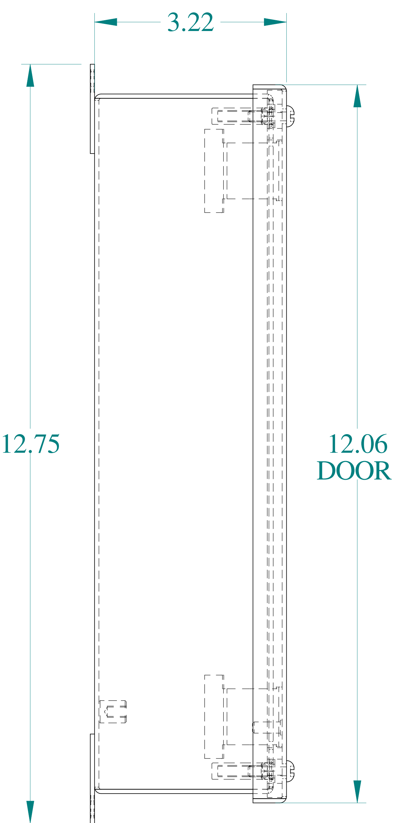
SIDE VIEW
