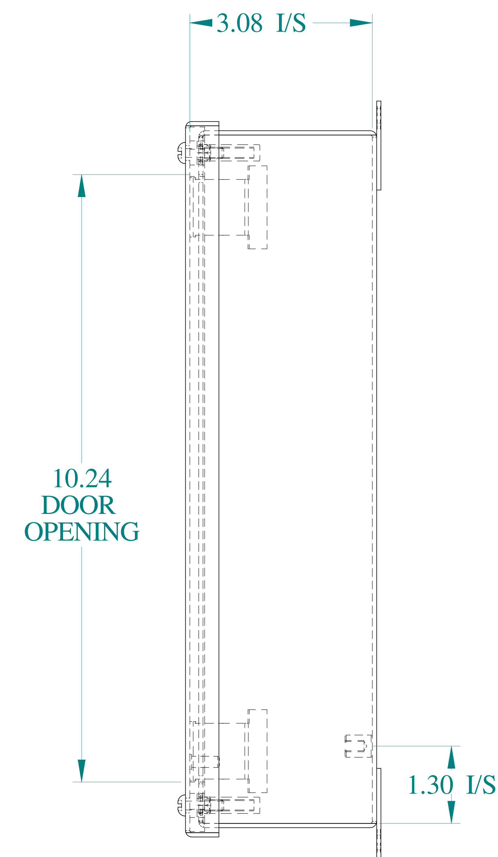
SIDE VIEW
