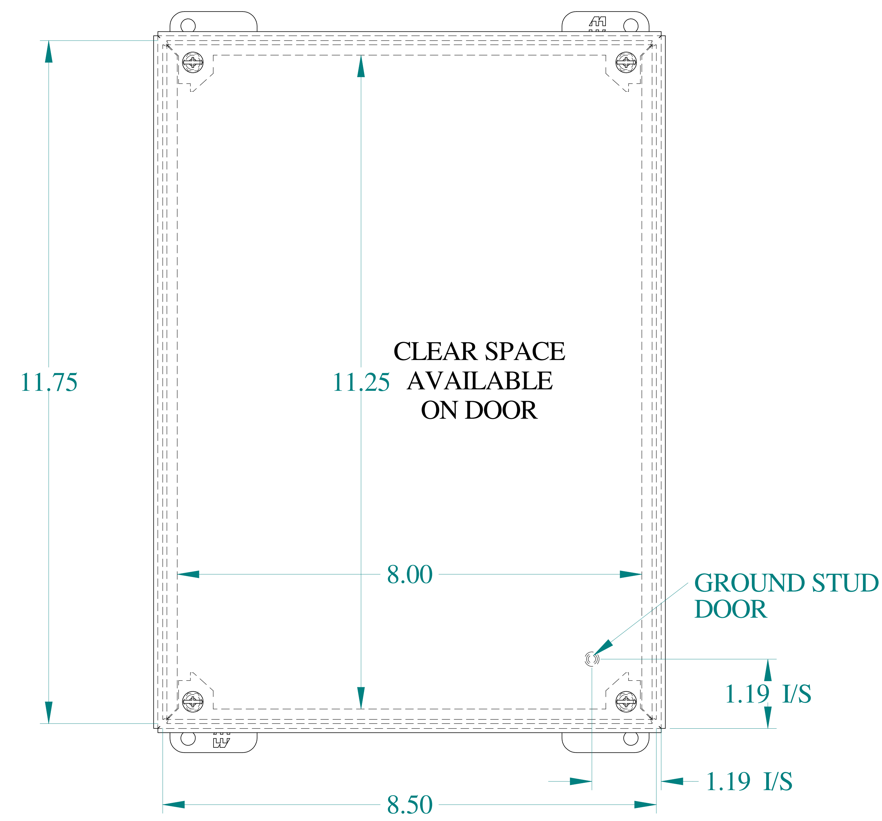
FRONT VIEW
