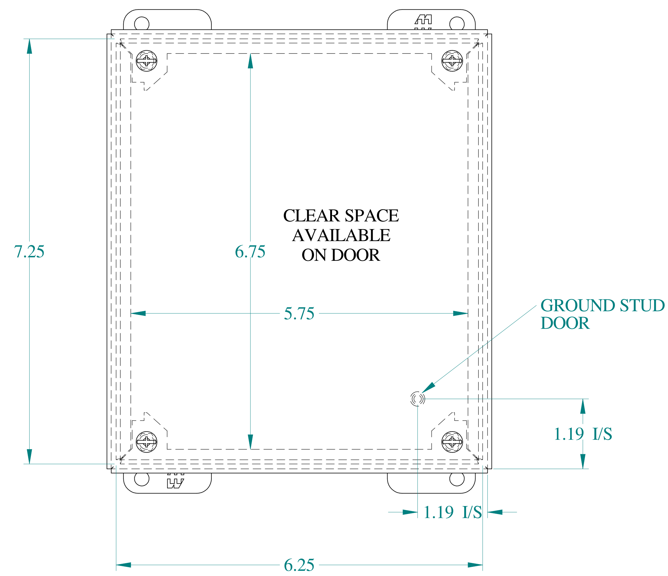
FRONT VIEW
