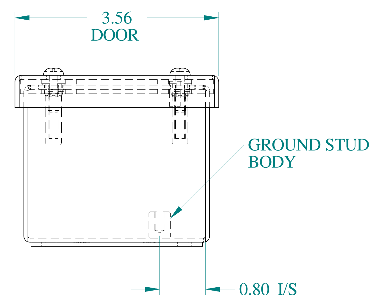
BOTTOM VIEW
