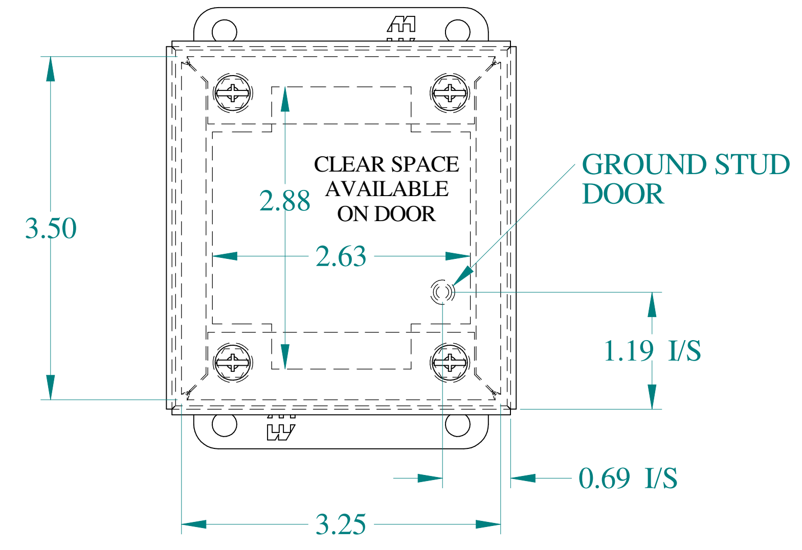
FRONT VIEW
