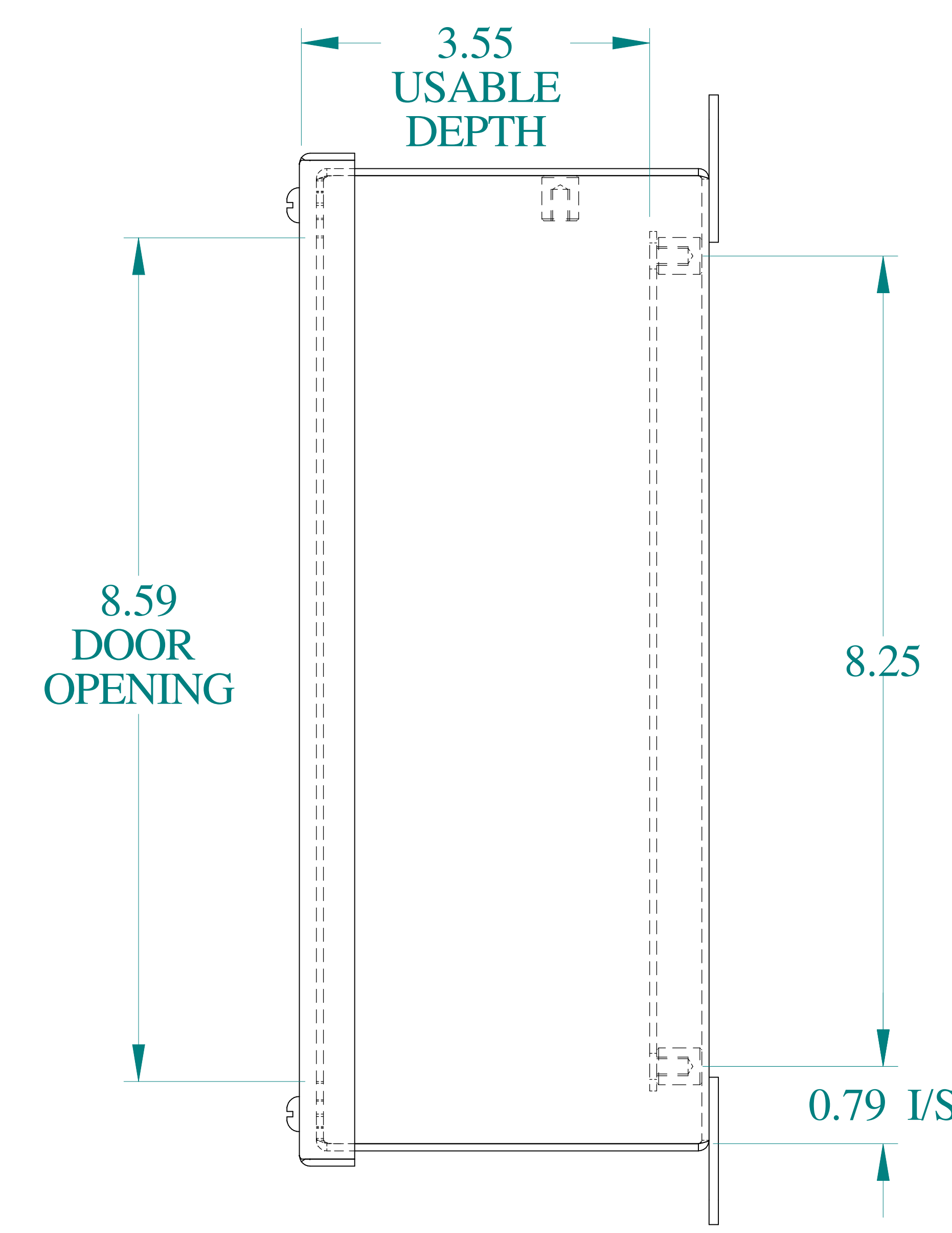
SIDE VIEW
