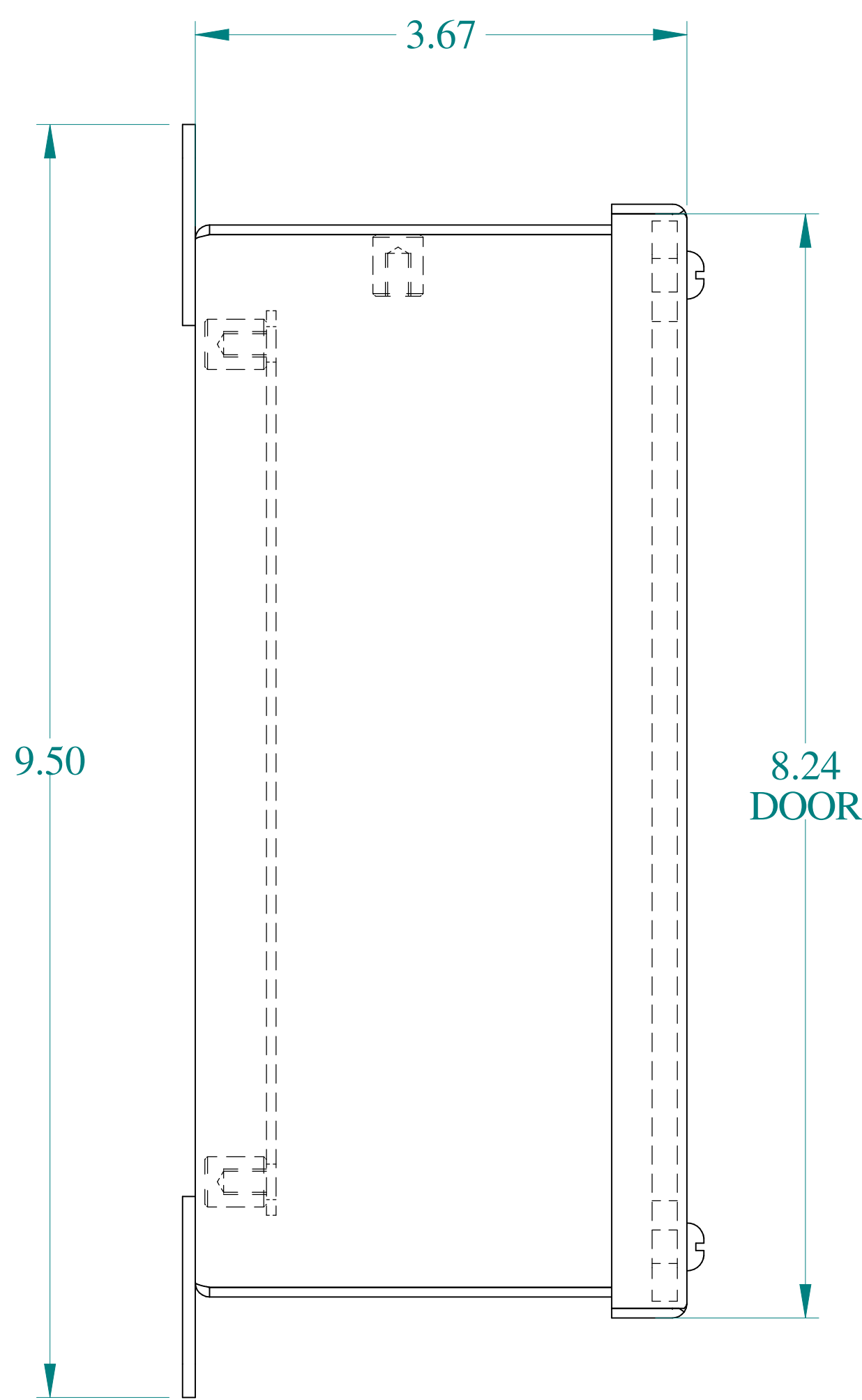
SIDE VIEW
