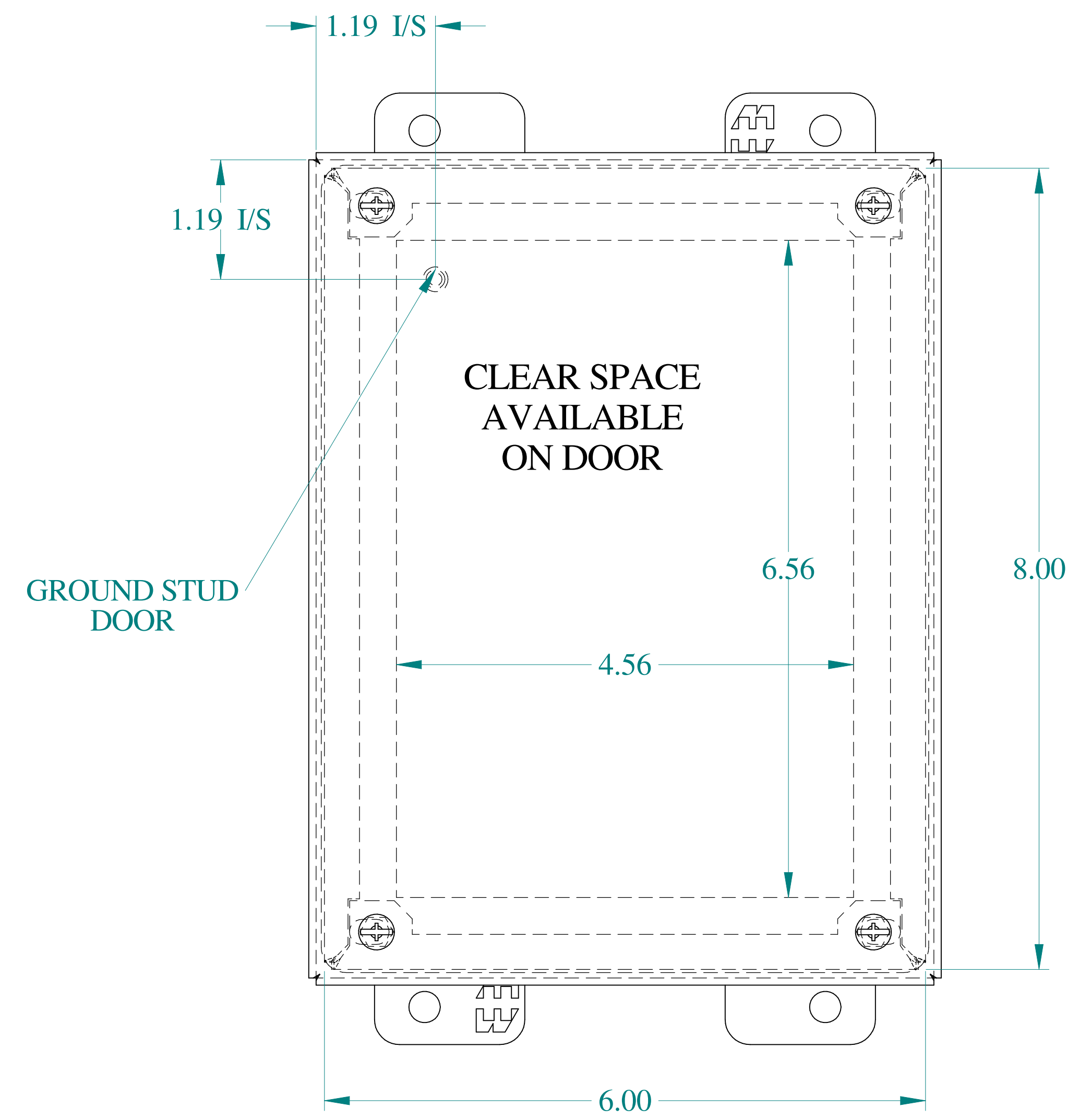
FRONT VIEW
