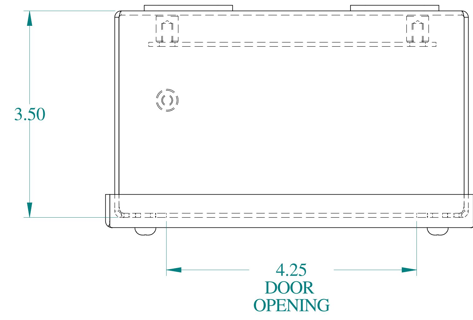
TOP VIEW
