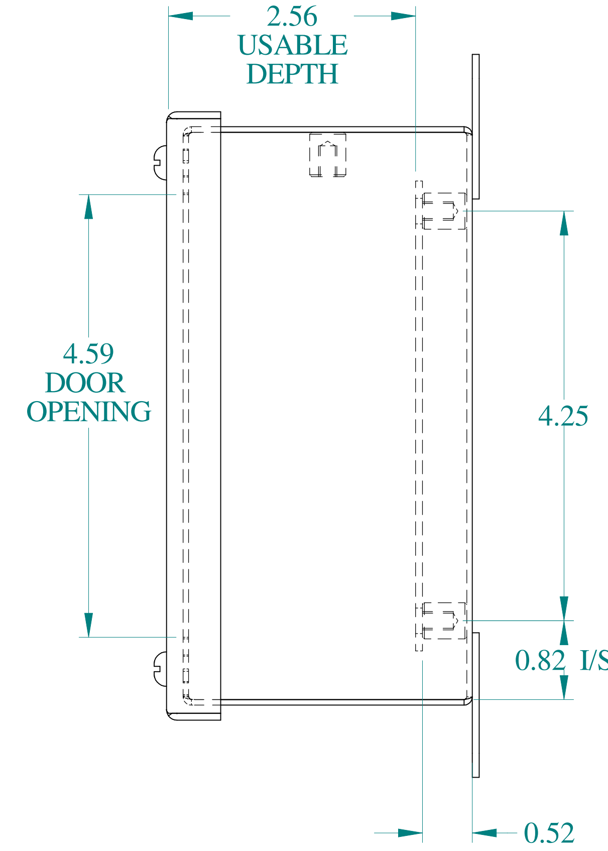
SIDE VIEW
