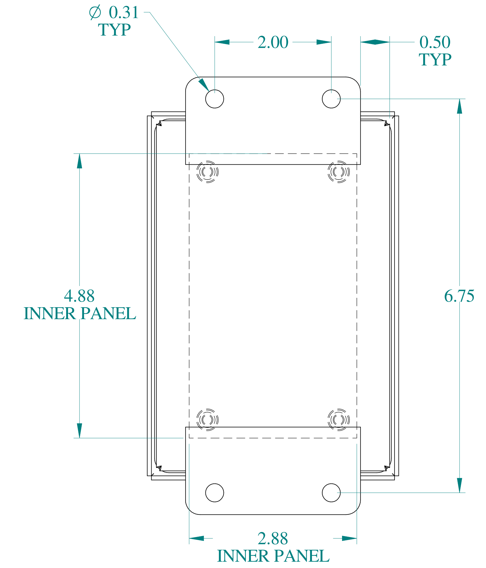
BACK VIEW
