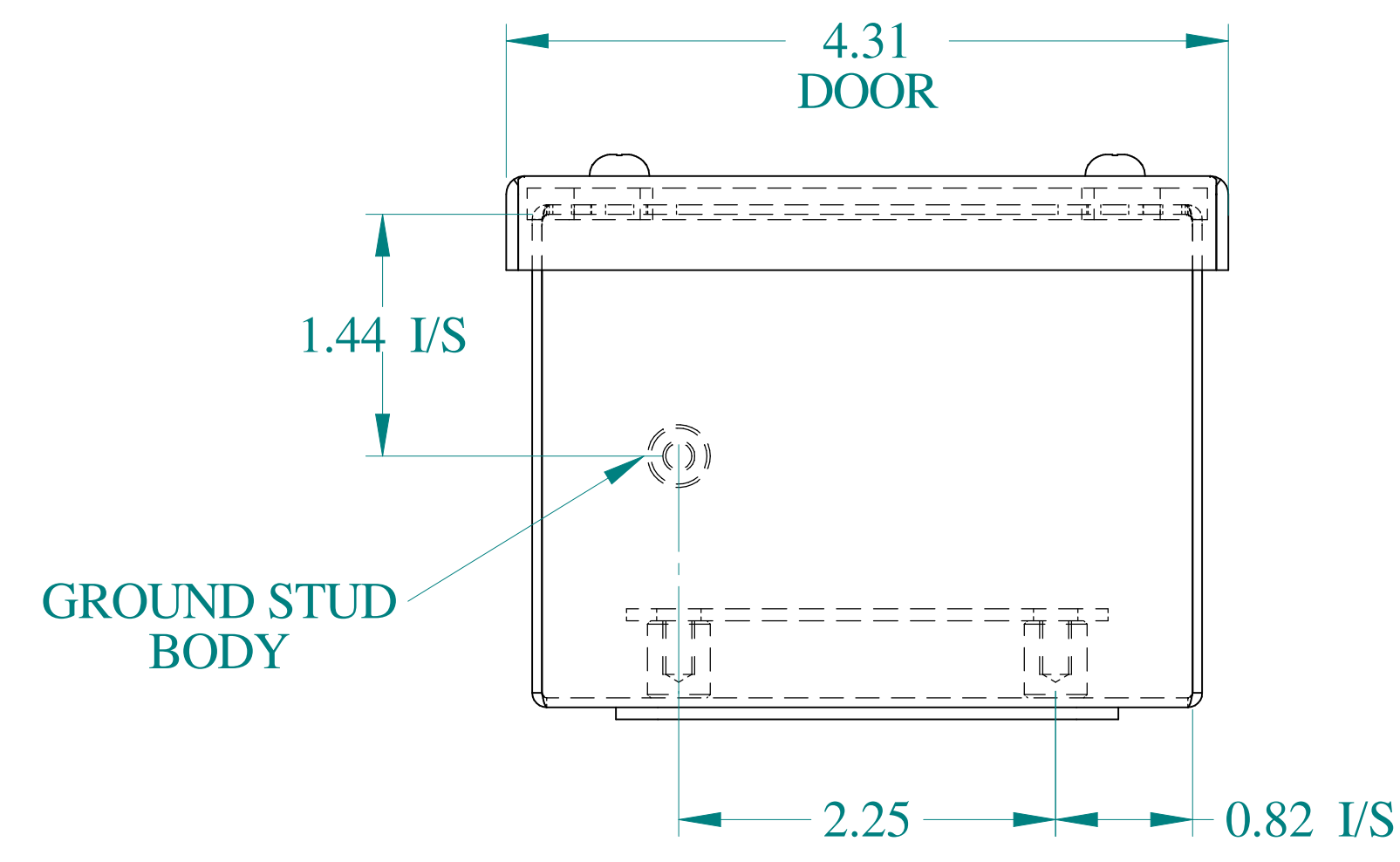
BOTTOM VIEW
