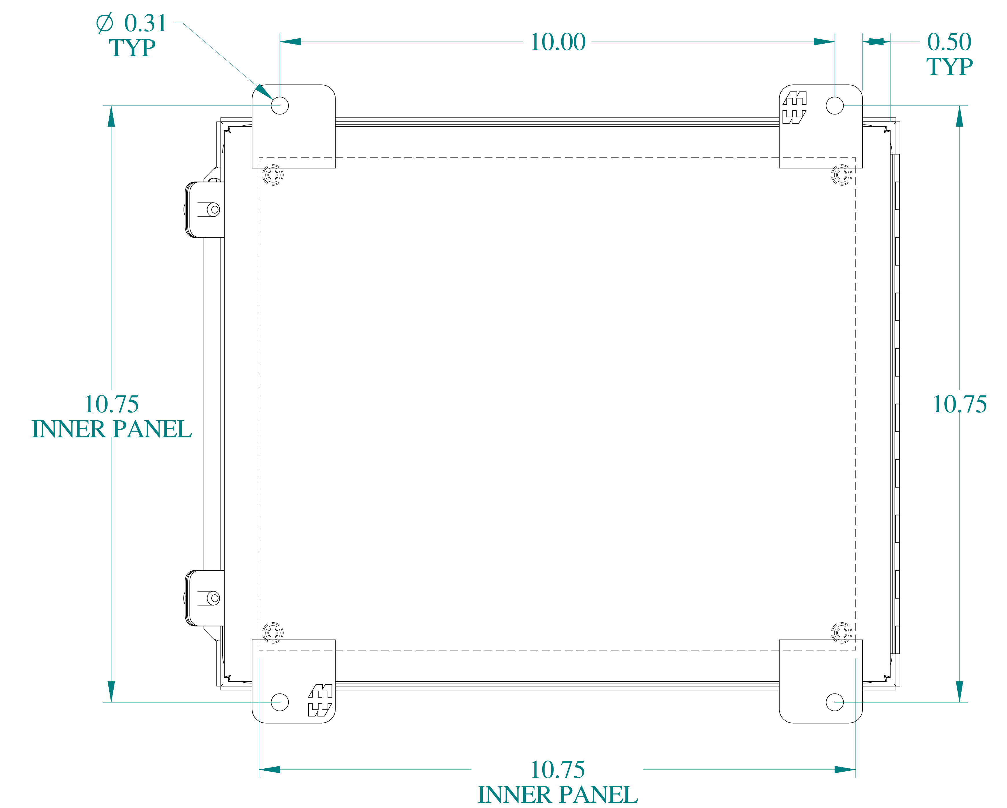
BACK VIEW
