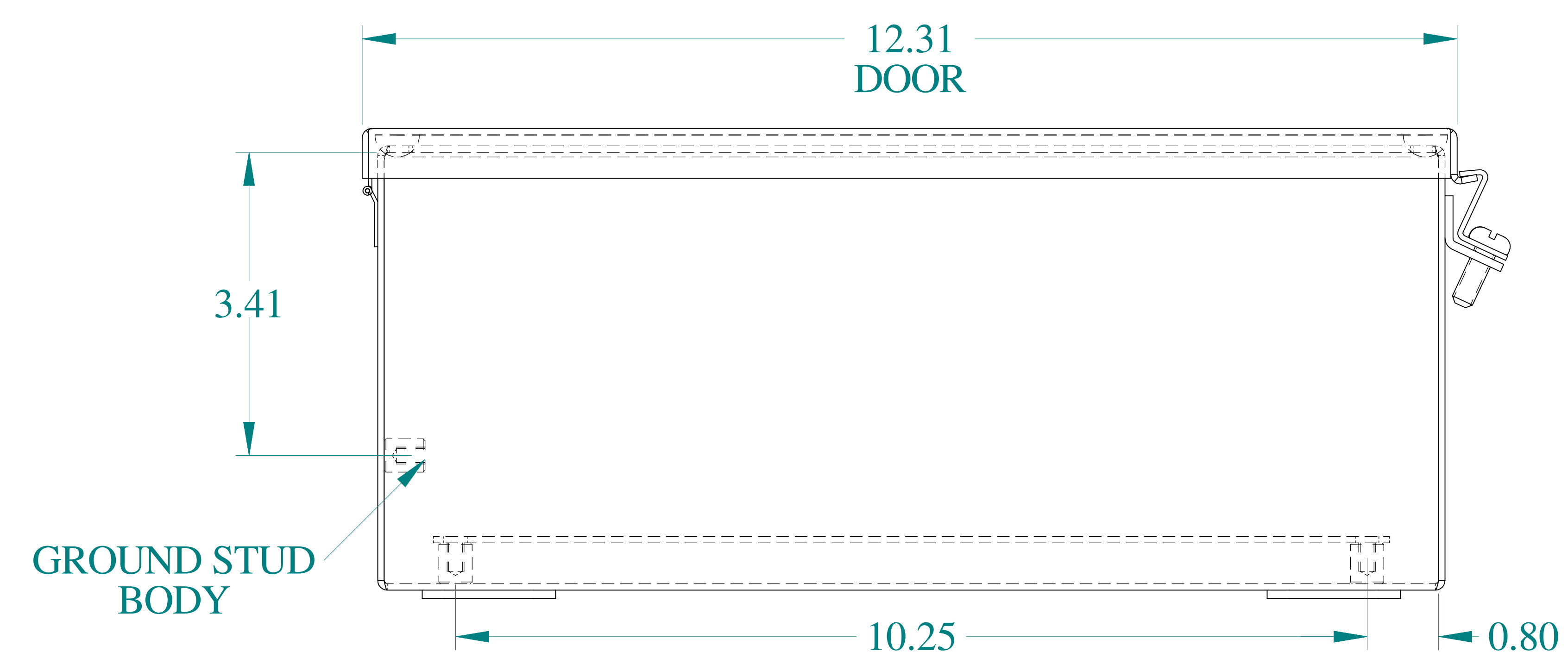
BOTTOM VIEW
