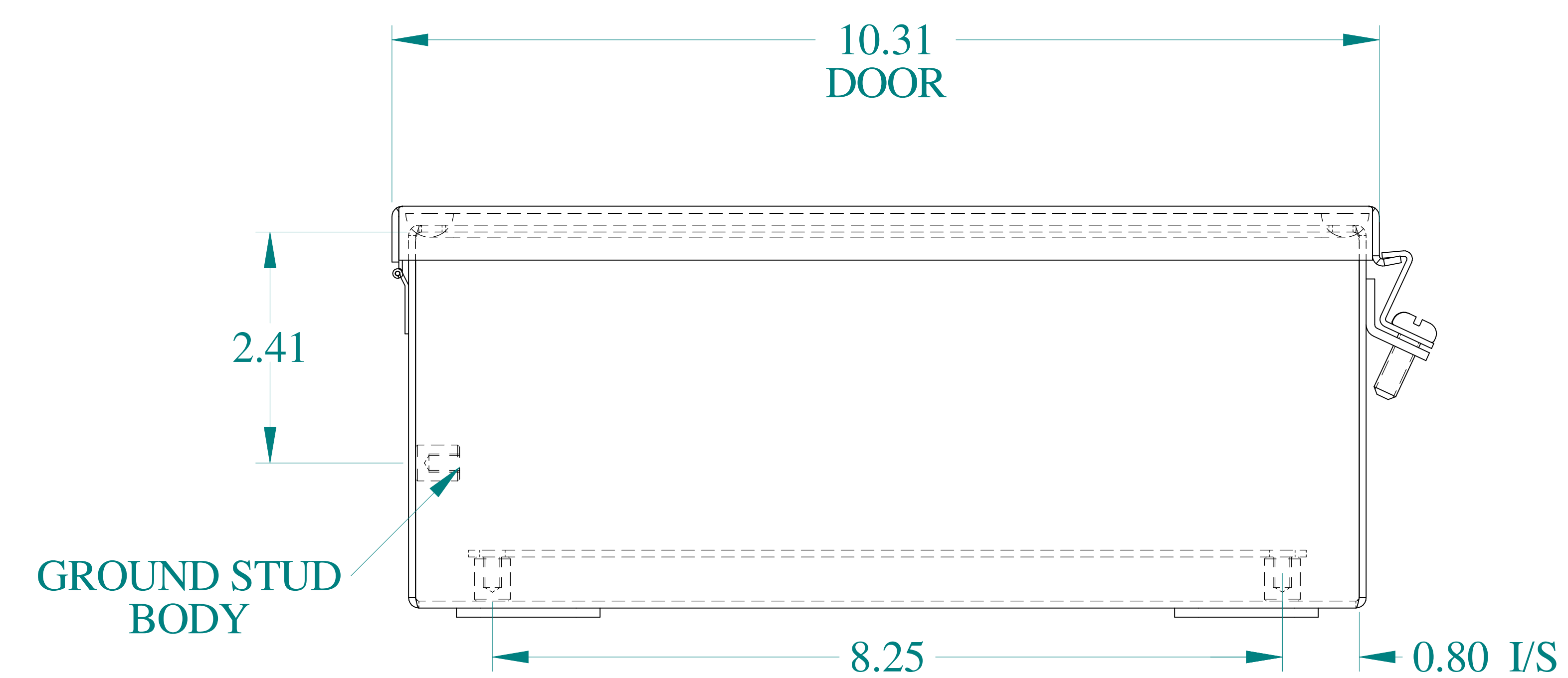
BOTTOM VIEW
