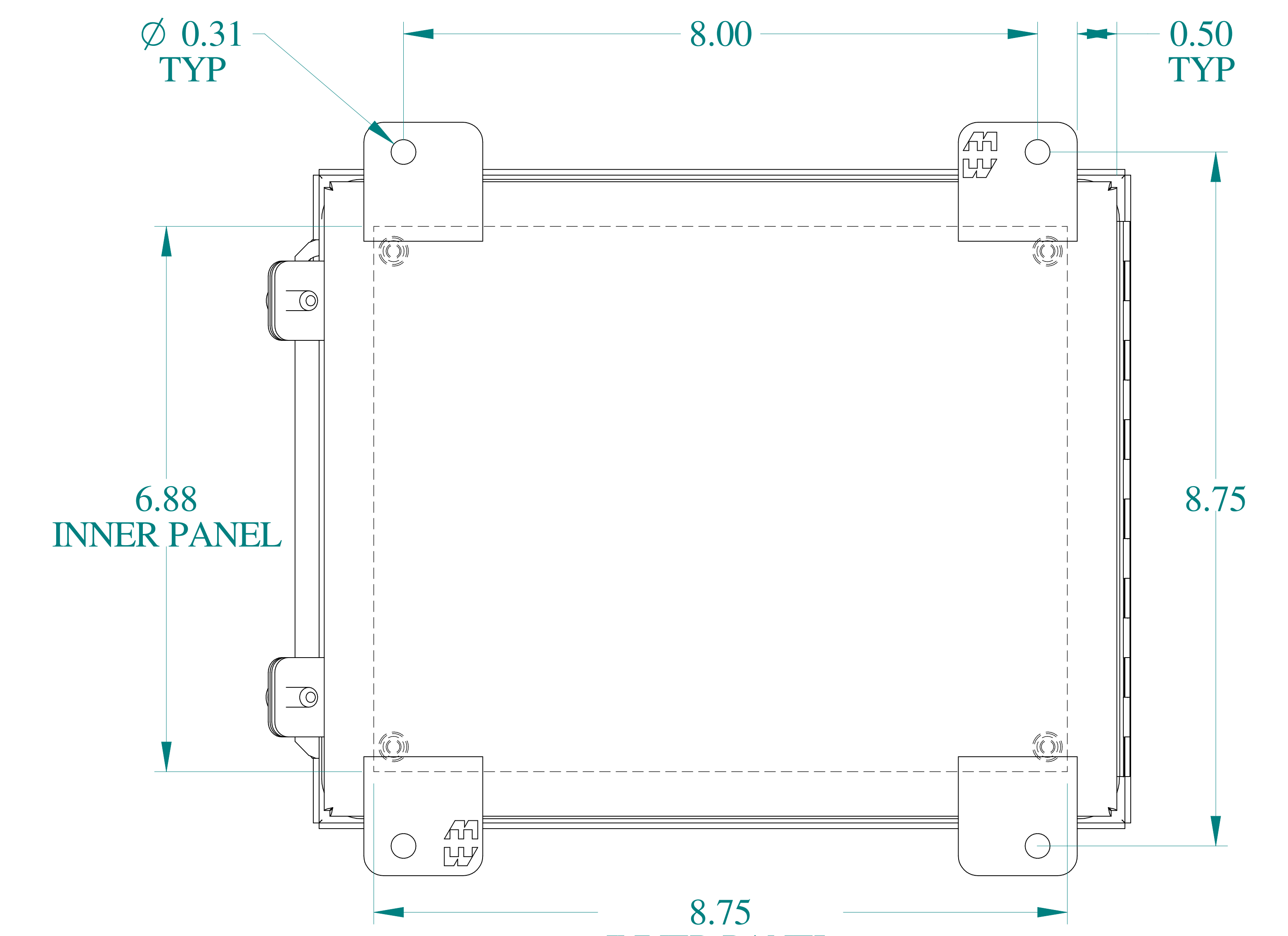
BACK VIEW
