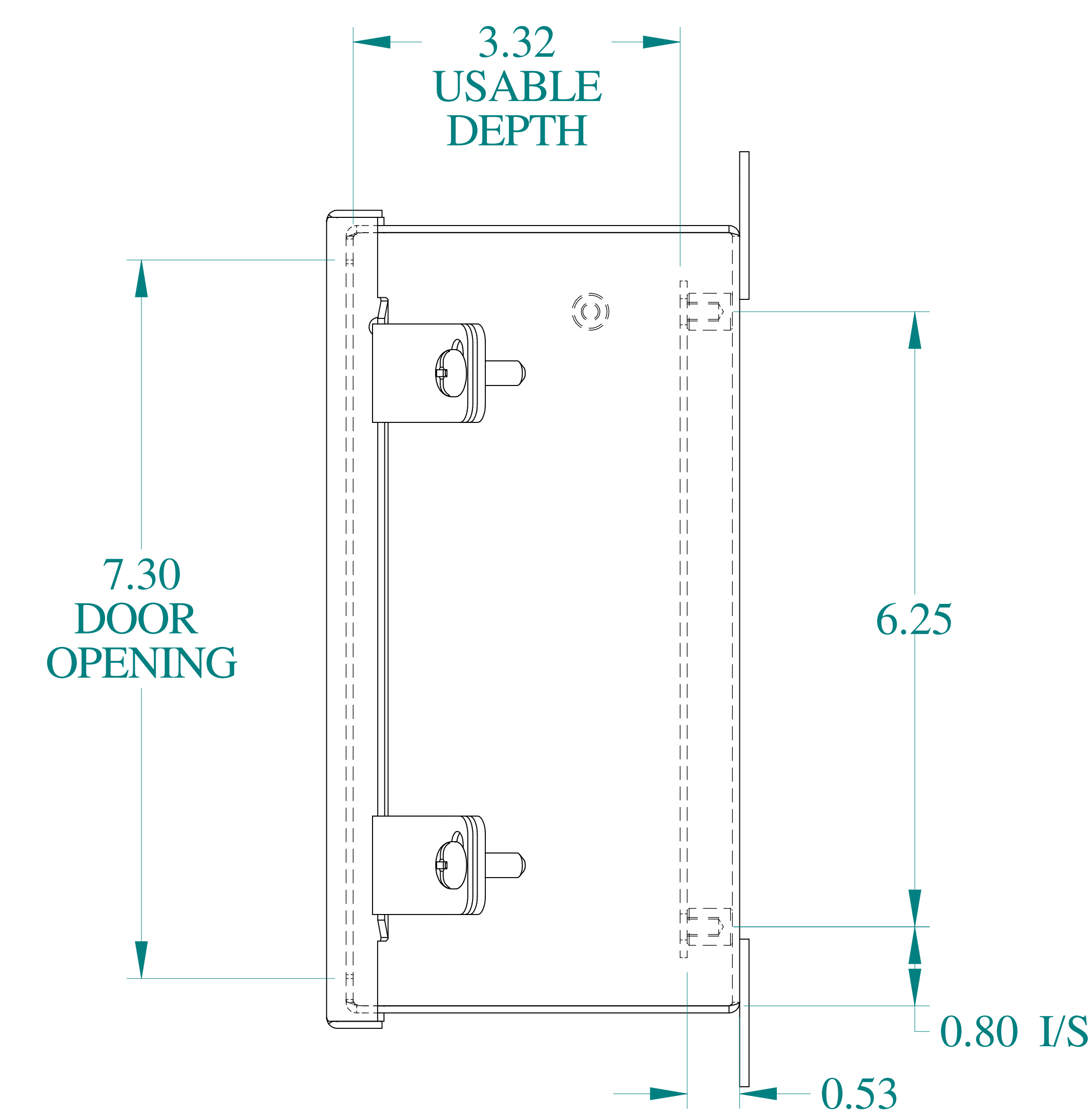
SIDE VIEW
