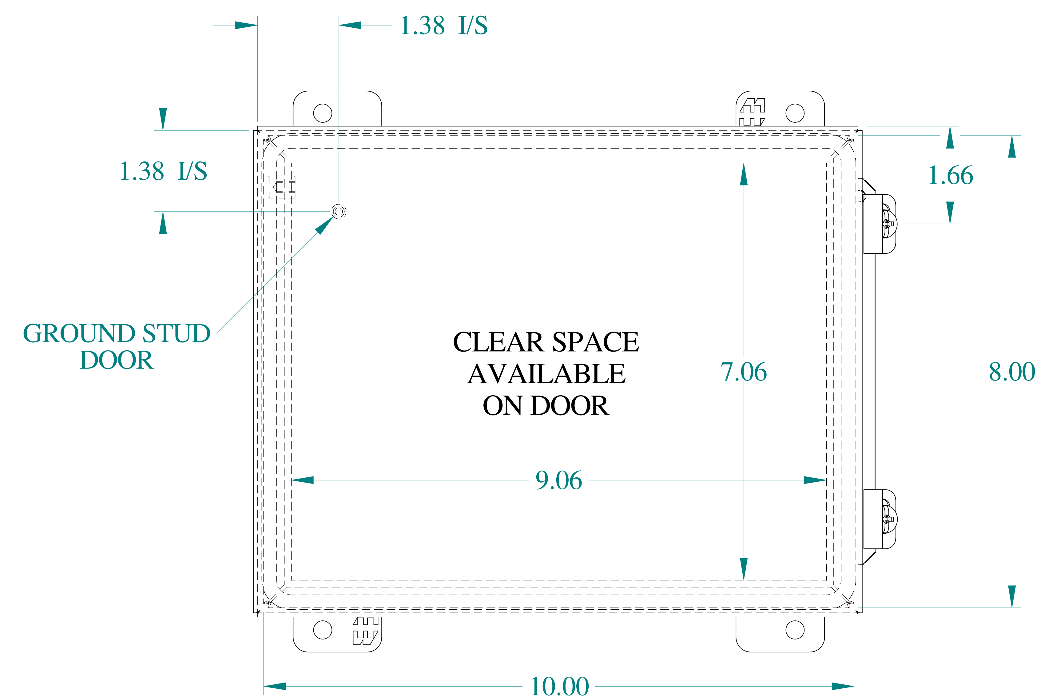
FRONT VIEW
