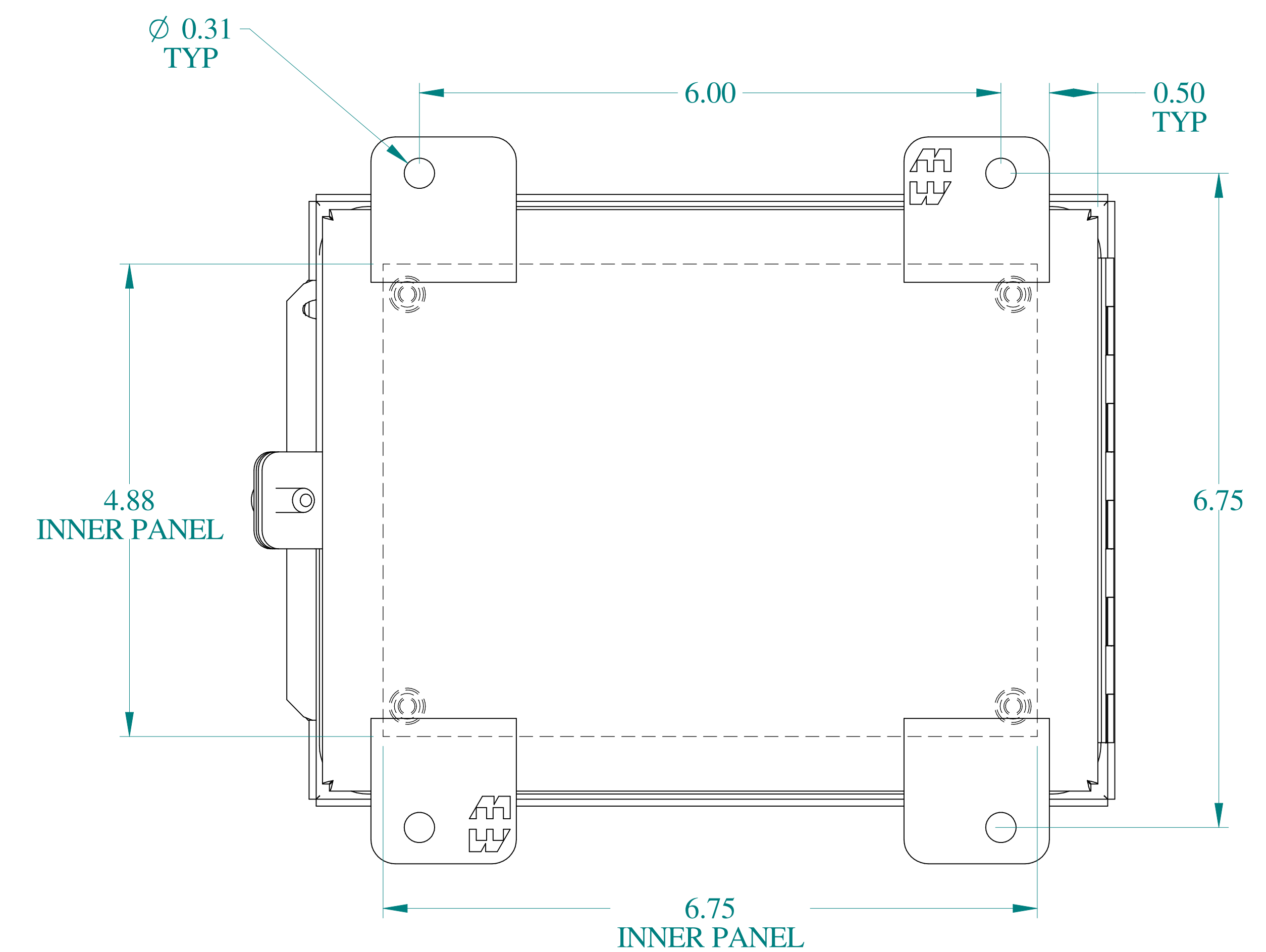
BACK VIEW
