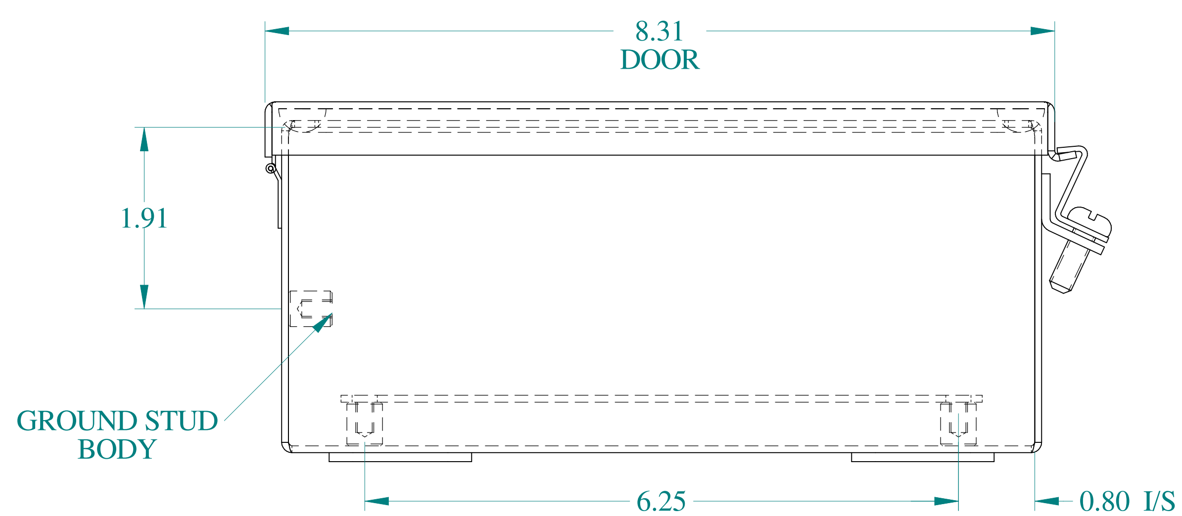
BOTTOM VIEW
