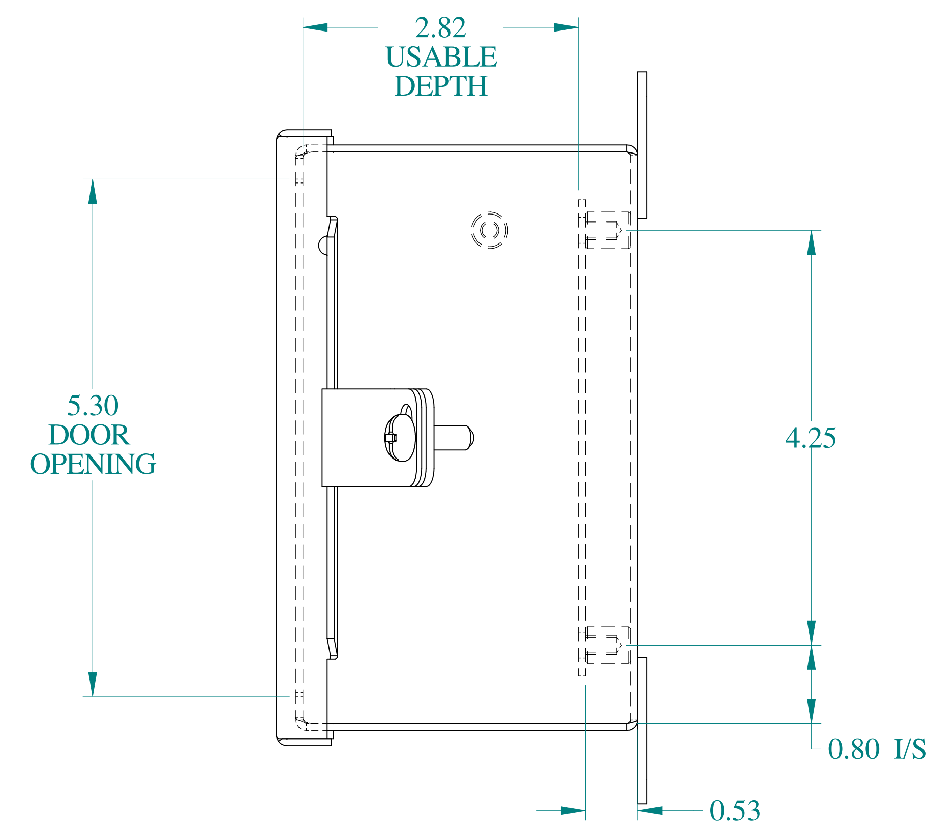
SIDE VIEW
