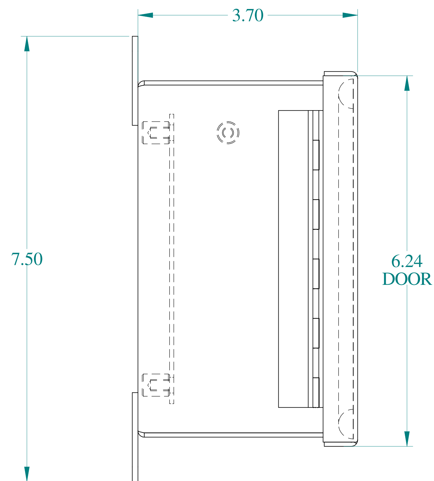
SIDE VIEW
