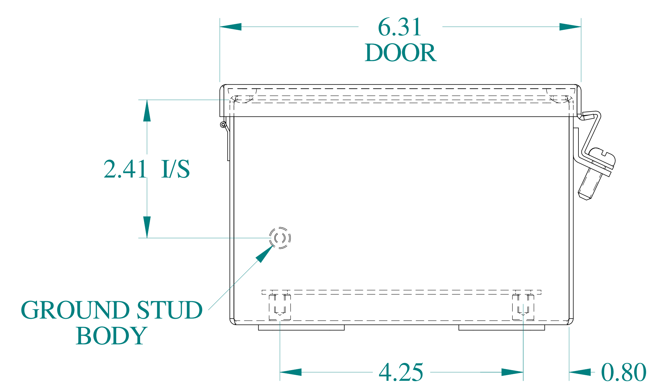
BOTTOM VIEW
