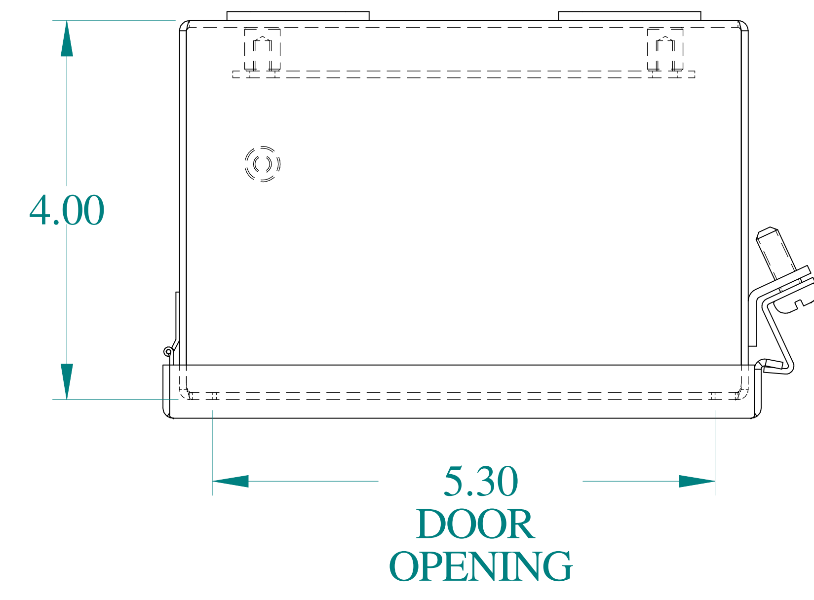
TOP VIEW
