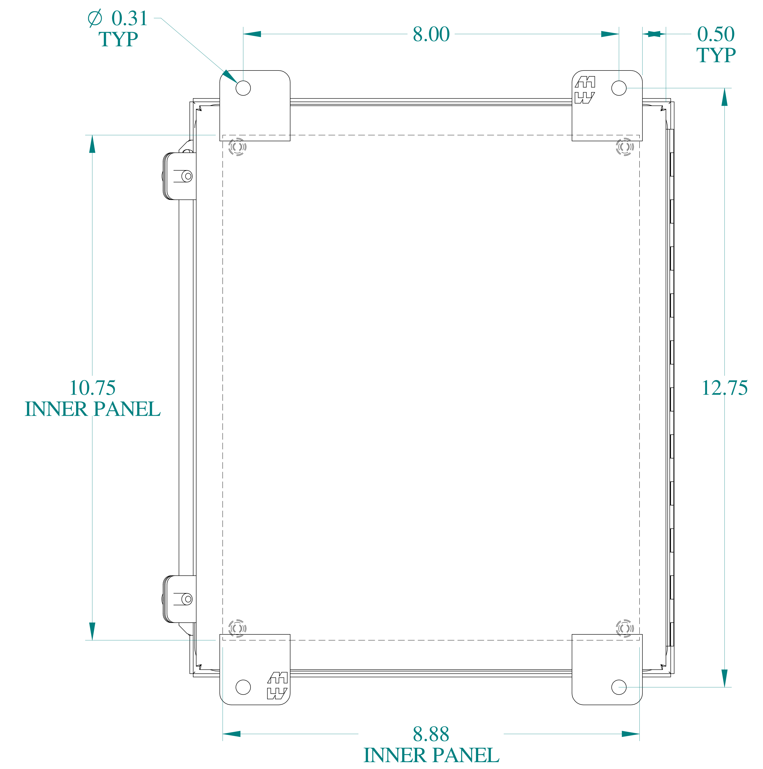
BACK VIEW
