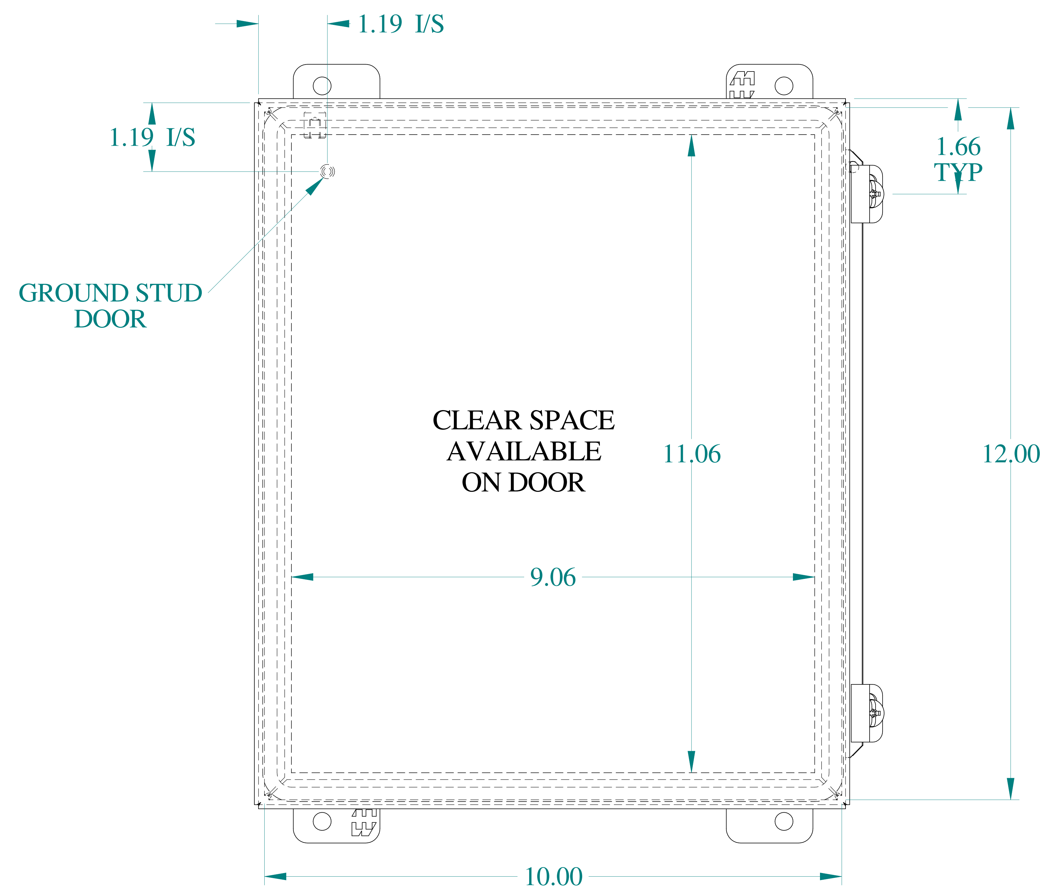
FRONT VIEW
