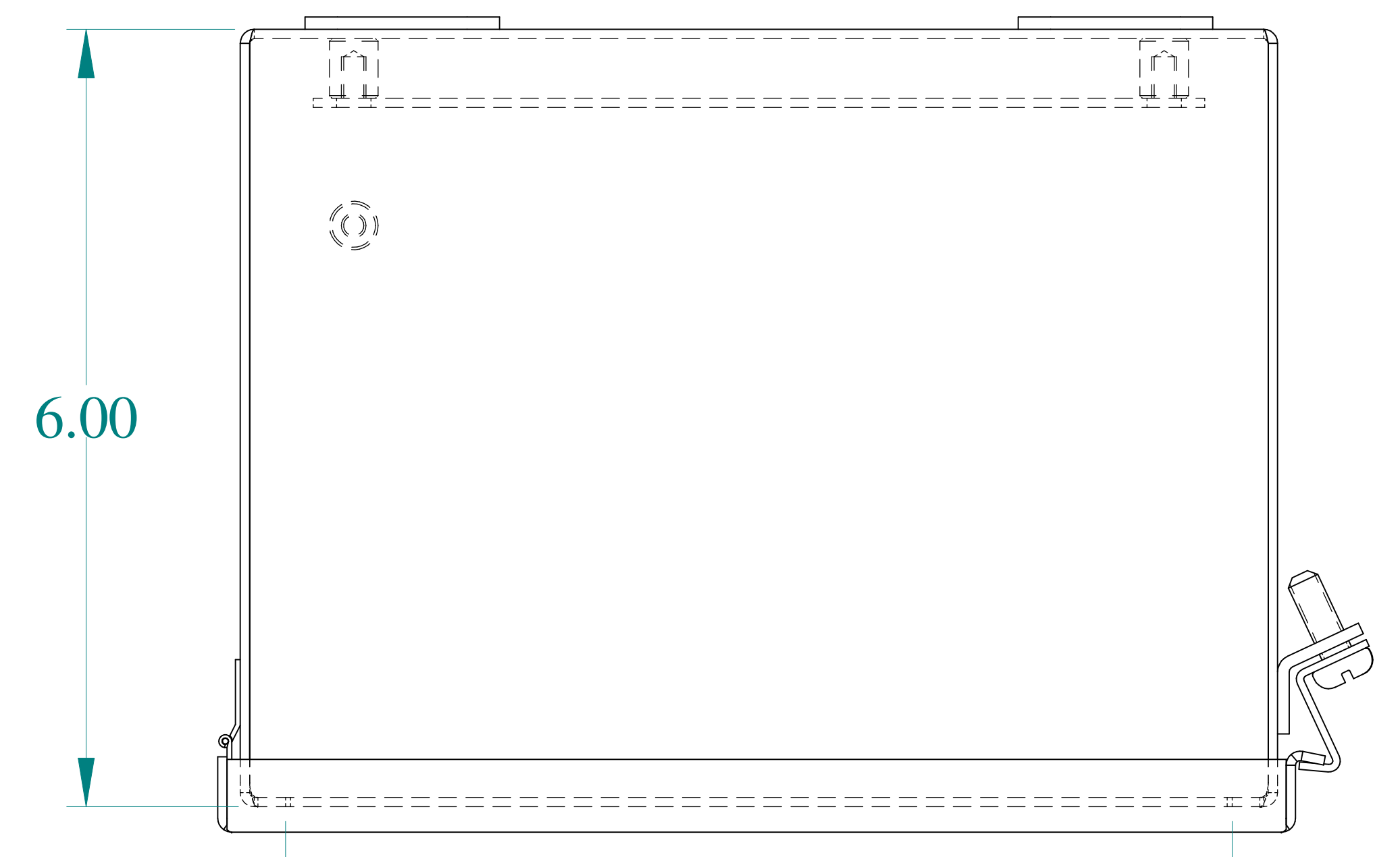
7.30 DOOR OPENING TOP VIEW
