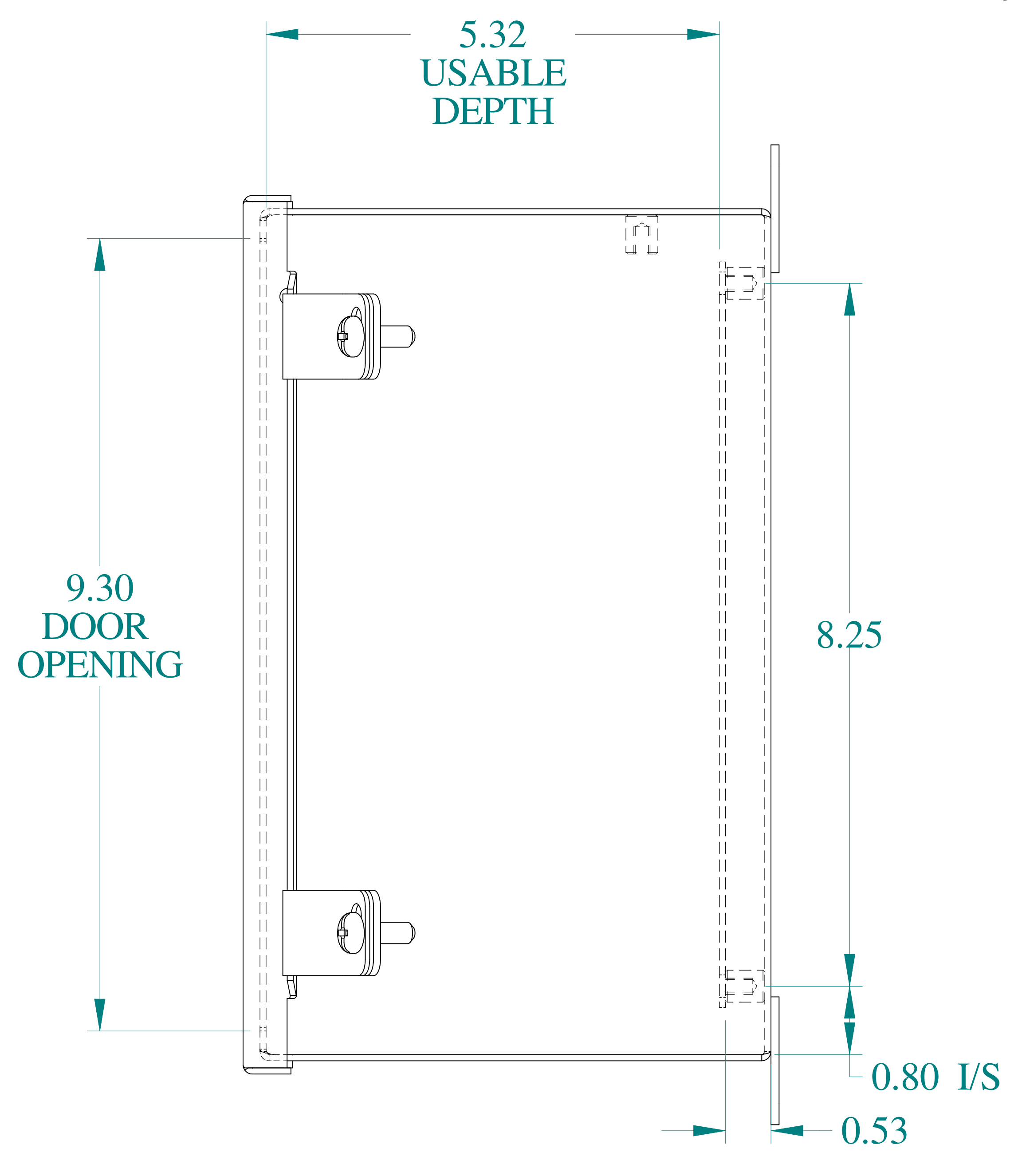
SIDE VIEW
