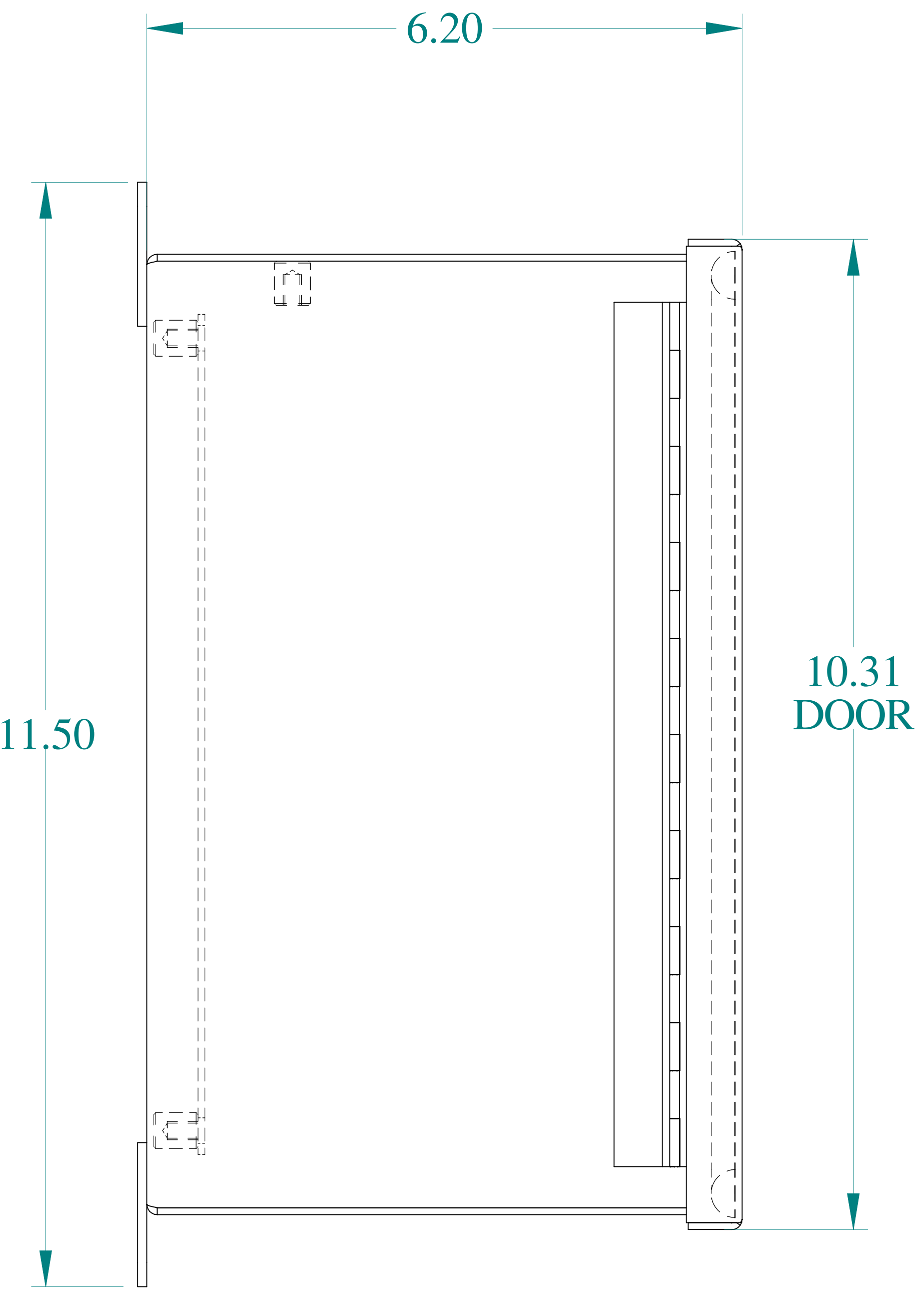
SIDE VIEW
