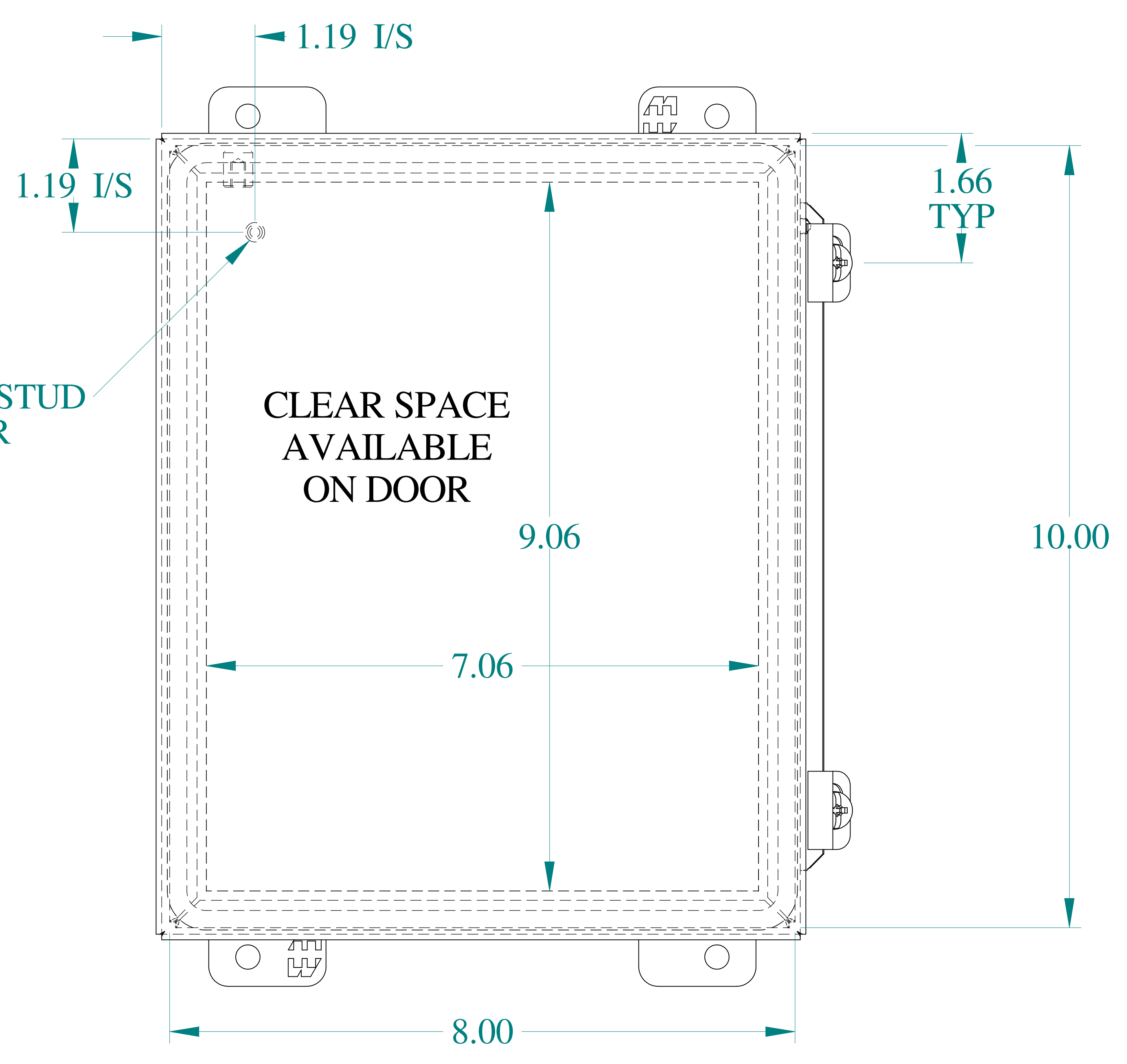
FRONT VIEW
