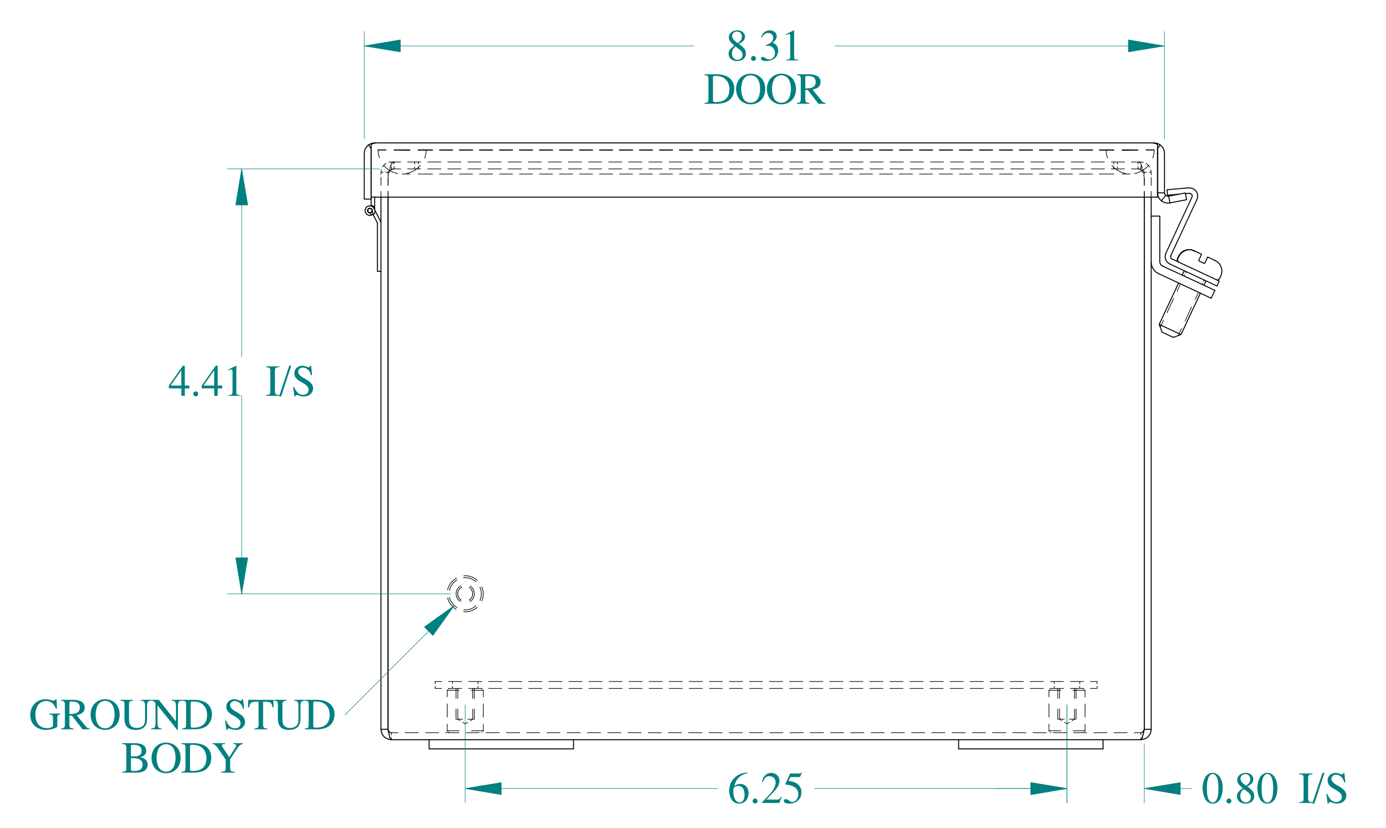
BOTTOM VIEW
