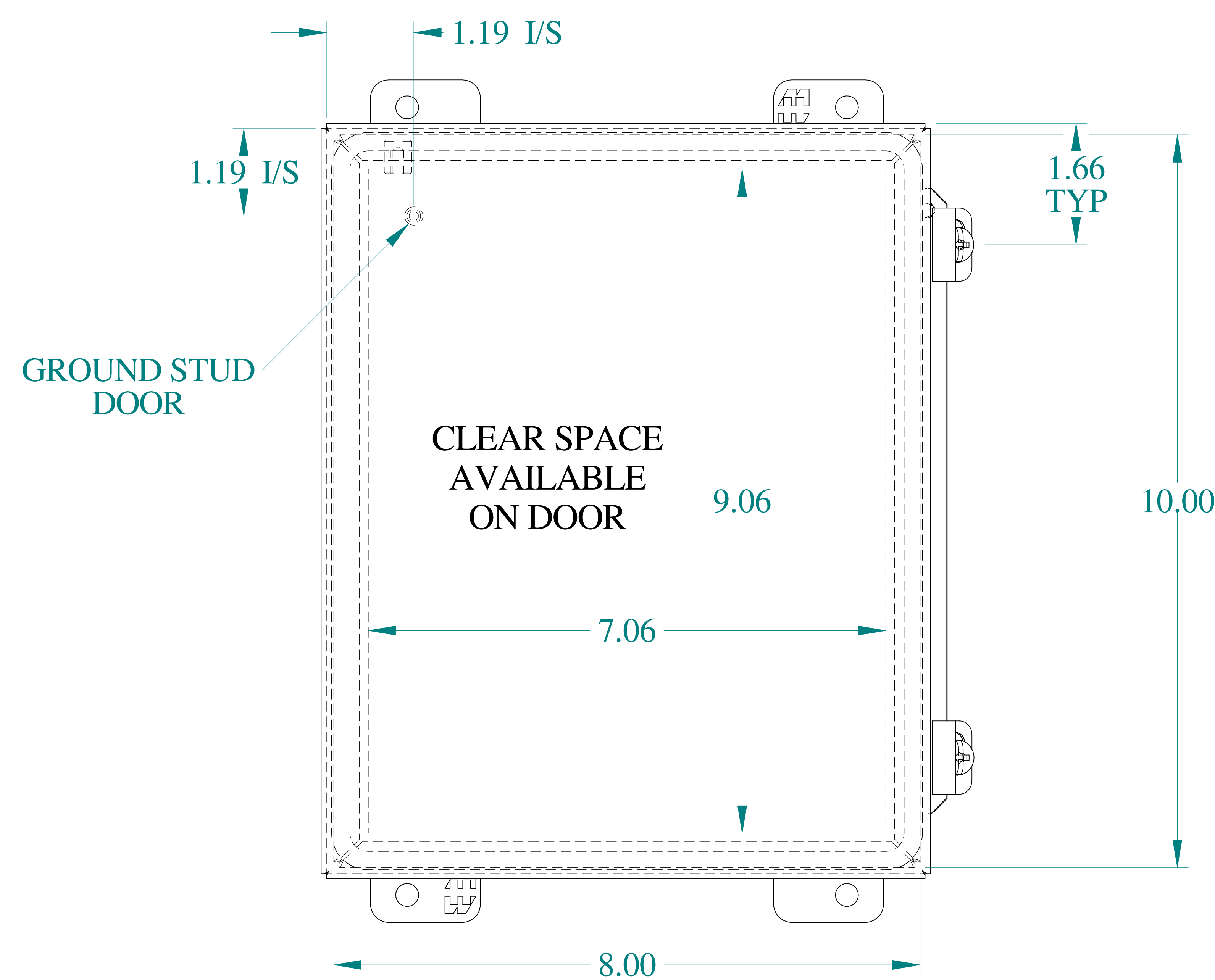
FRONT VIEW
