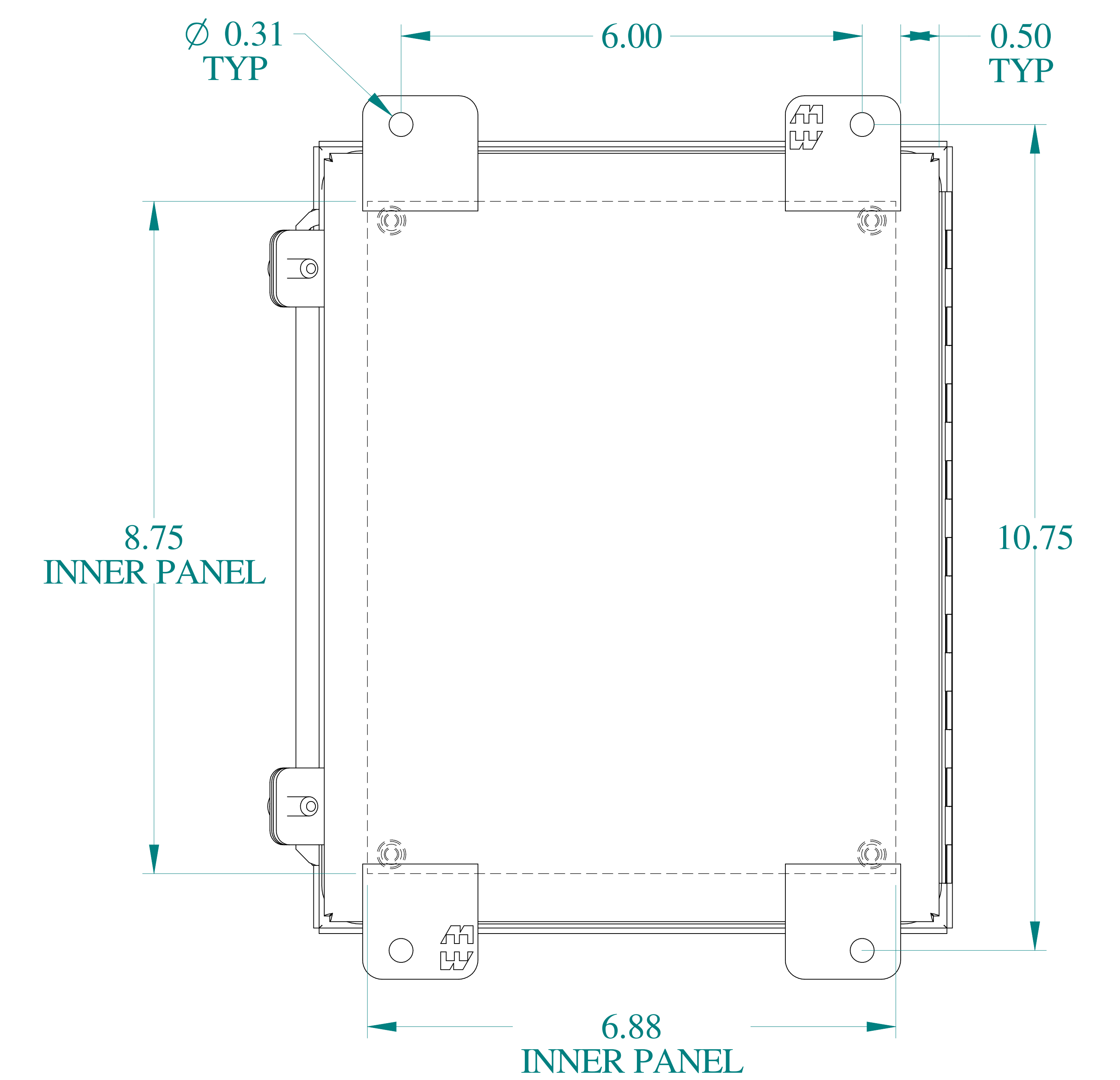
BACK VIEW
