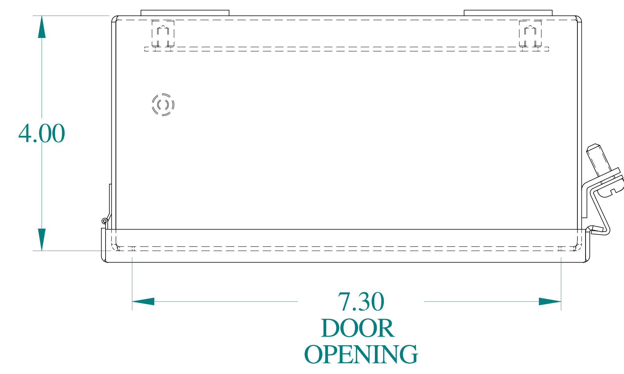
TOP VIEW
