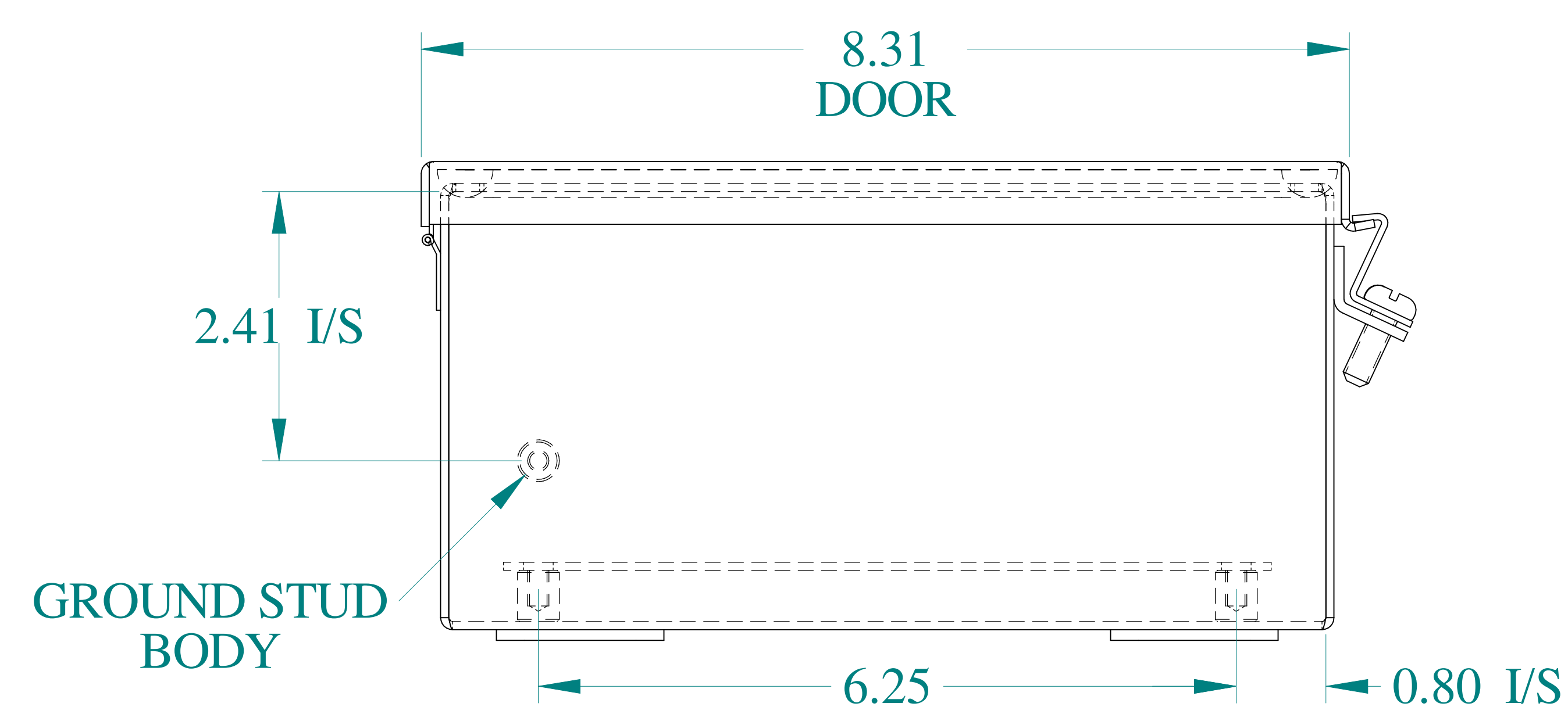
BOTTOM VIEW
