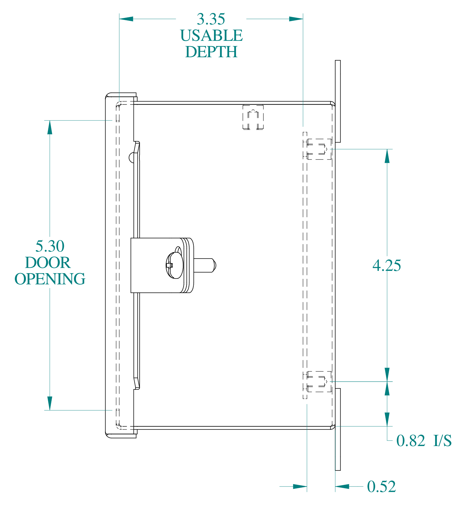
SIDE VIEW
