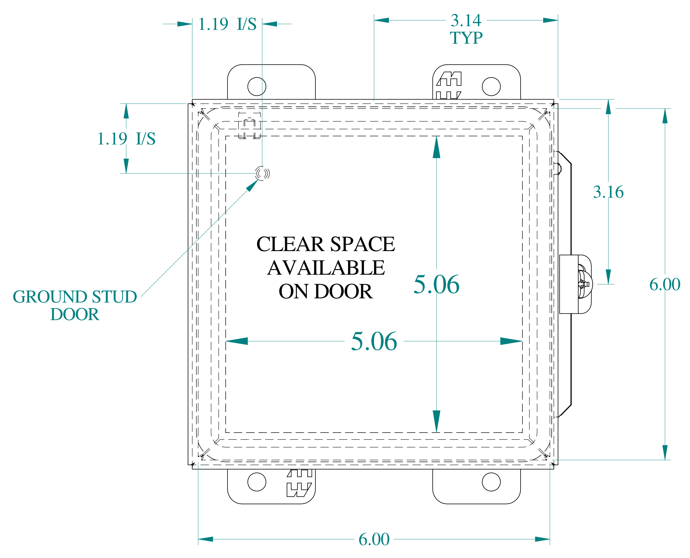
FRONT VIEW
