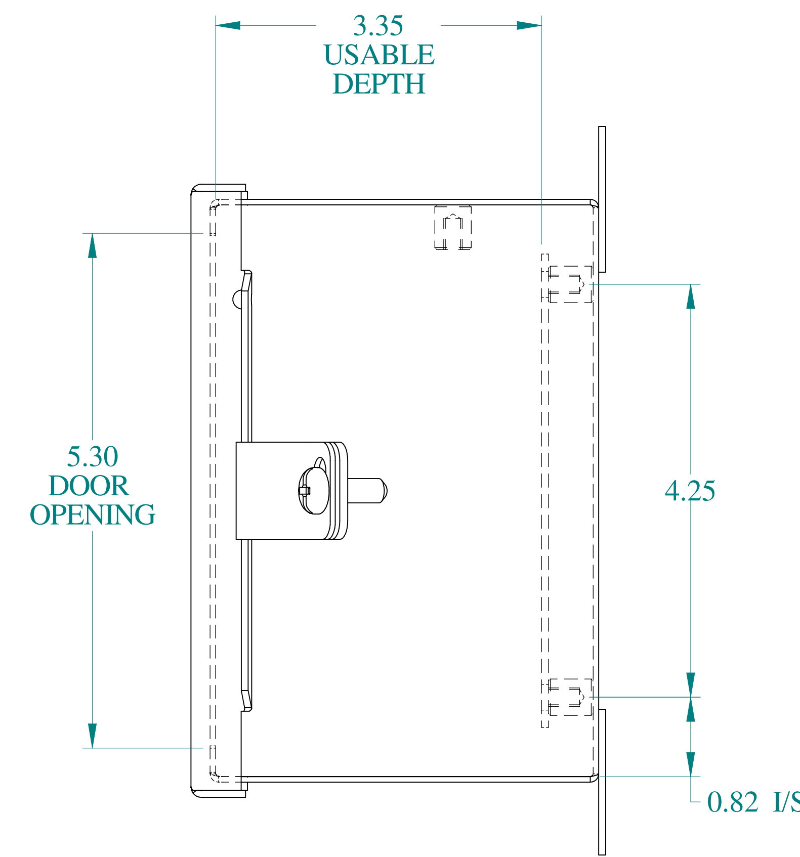
SIDE VIEW
