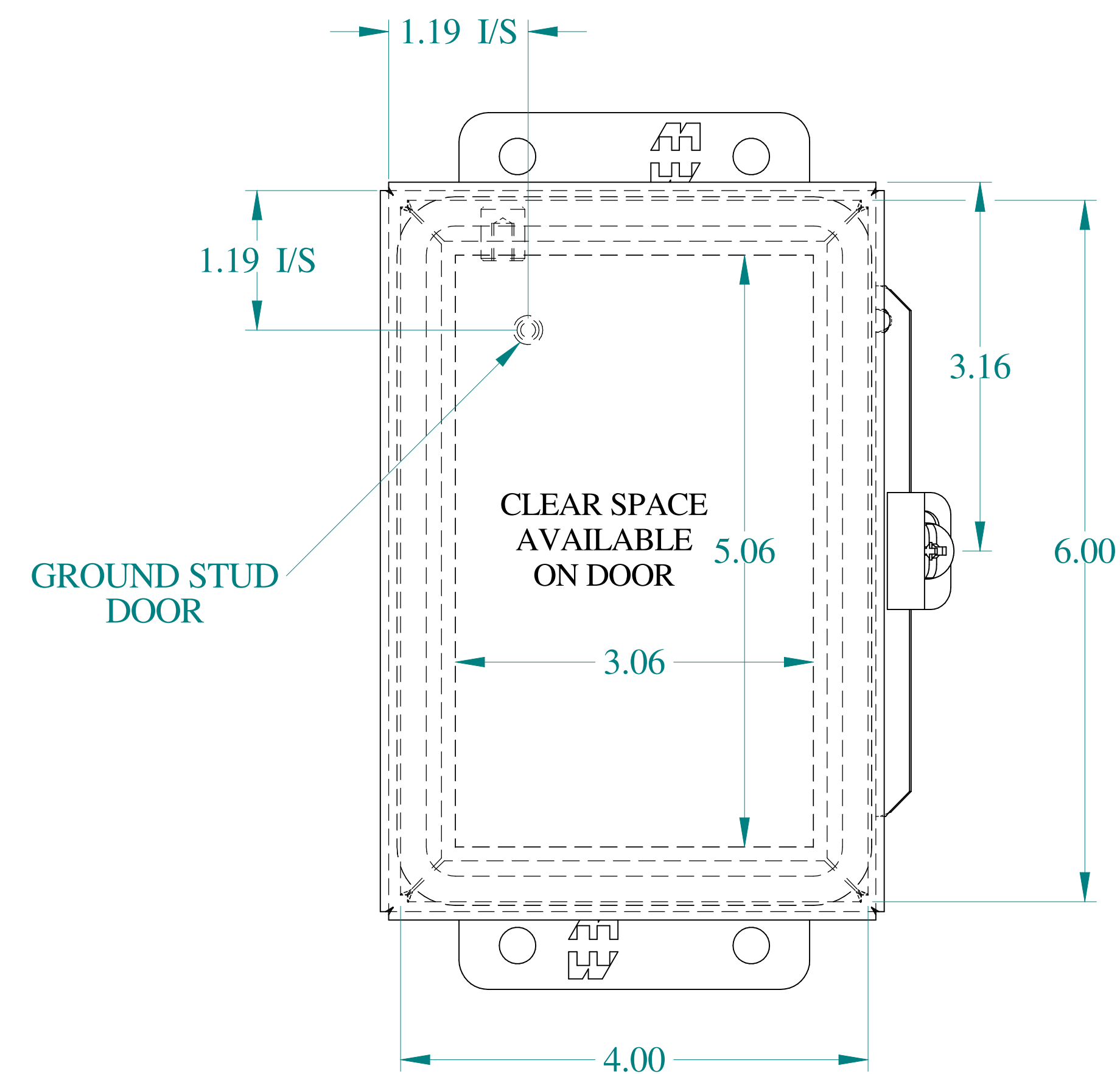
FRONT VIEW
