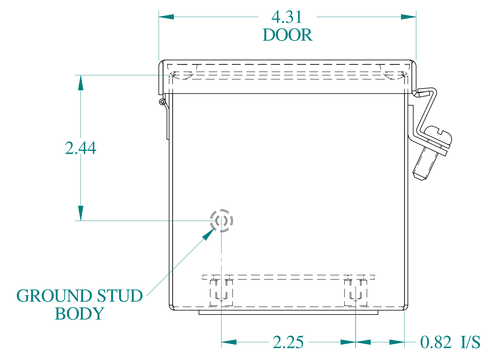
BOTTOM VIEW
