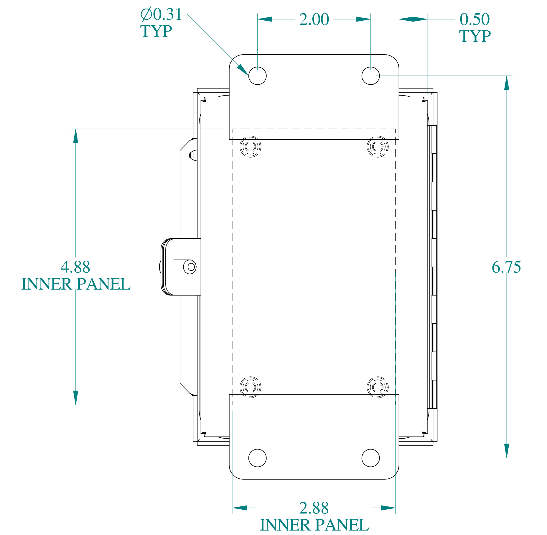
BACK VIEW
