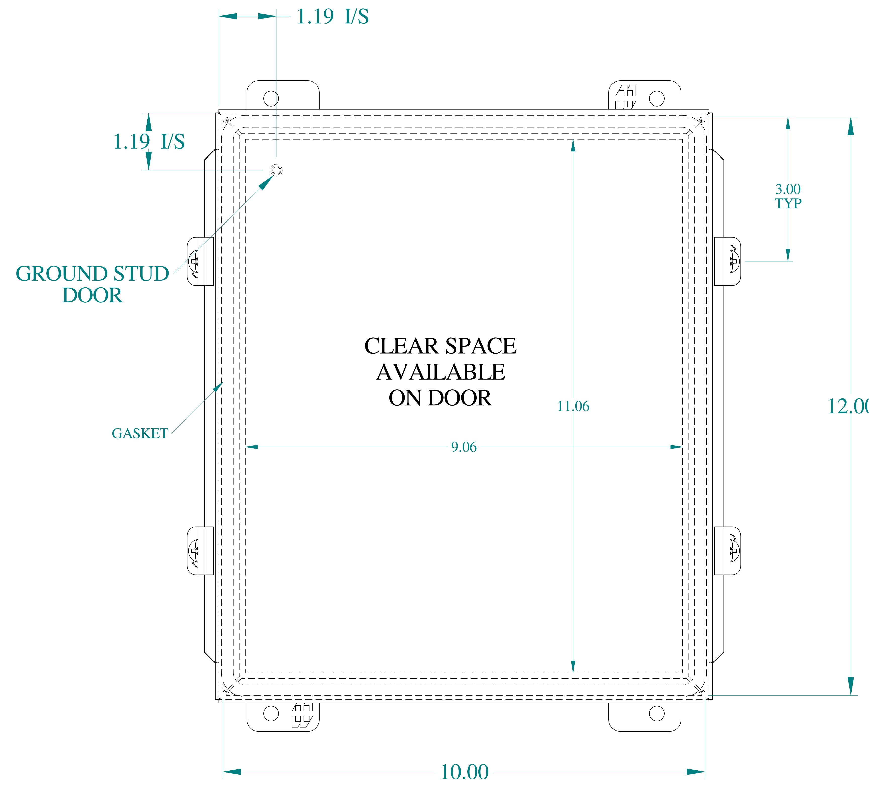
FRONT VIEW
