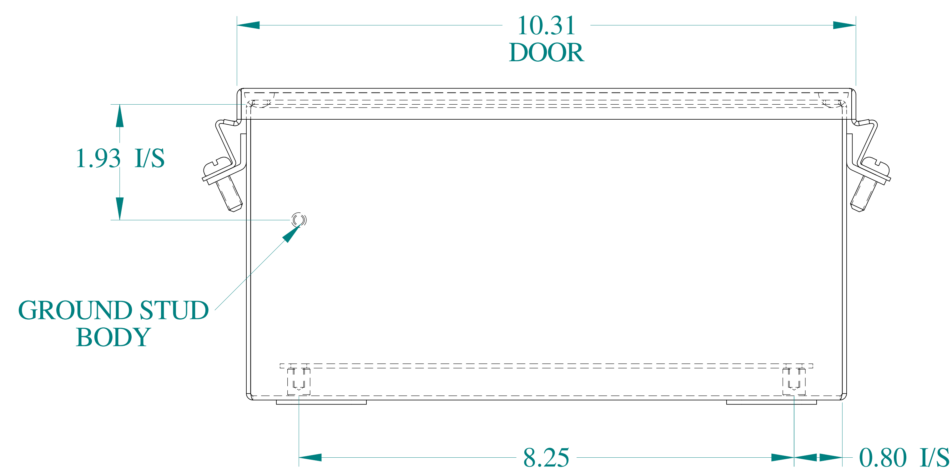
BOTTOM VIEW
