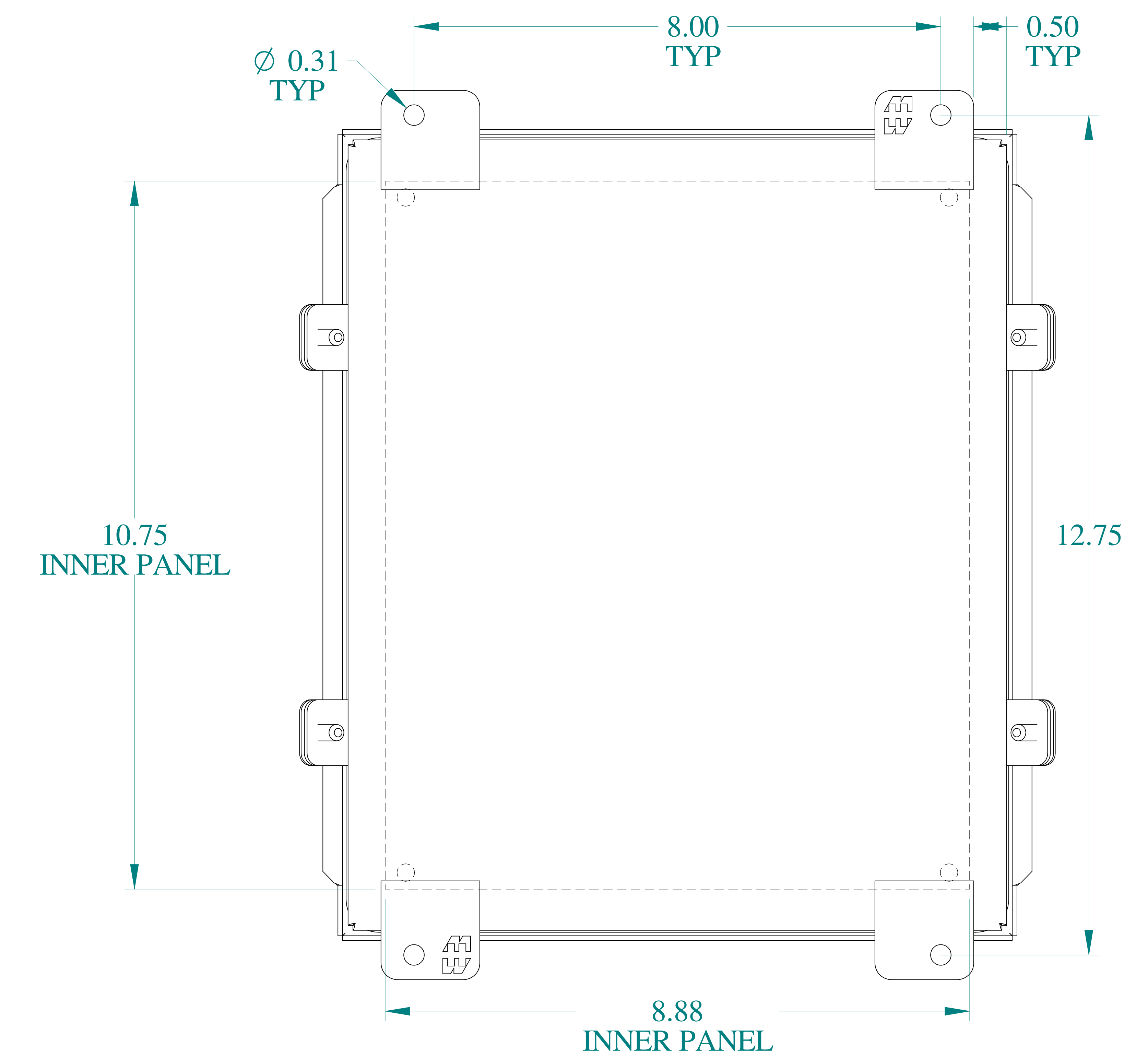
BACK VIEW
