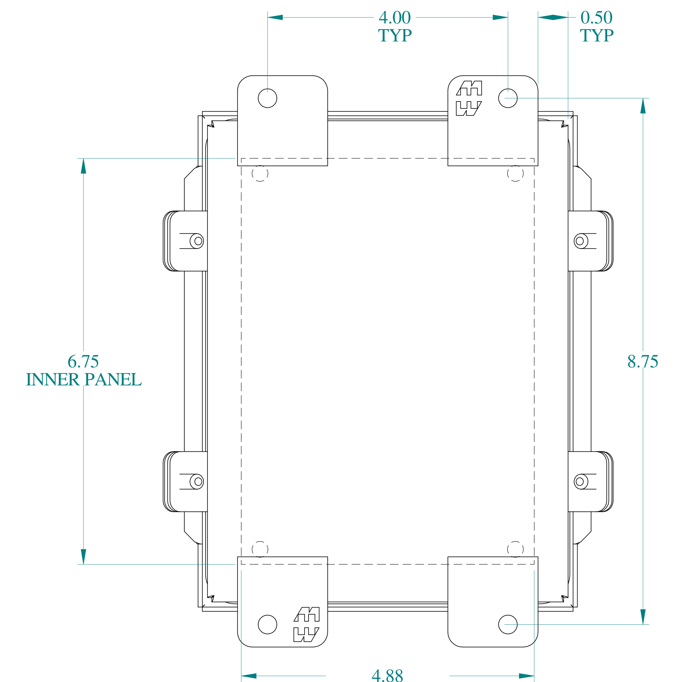
BACK VIEW
