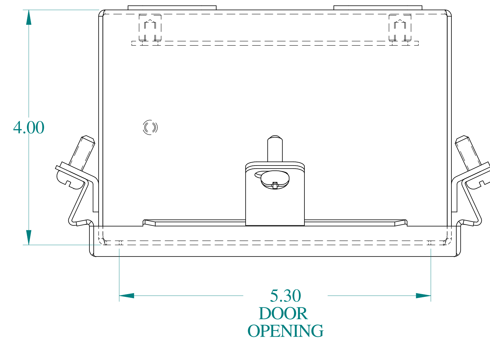
TOP VIEW
