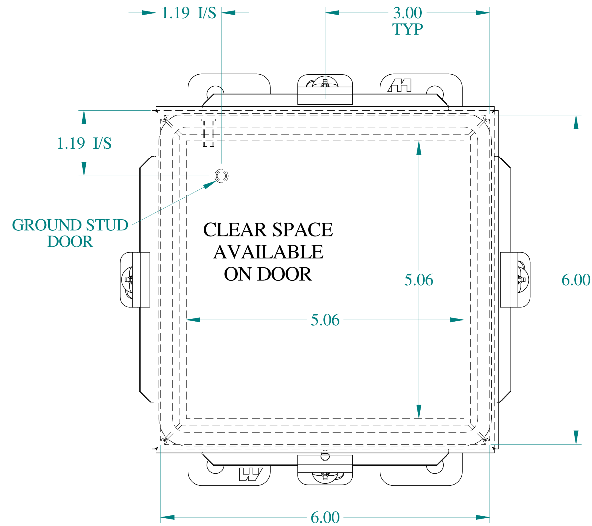
FRONT VIEW
