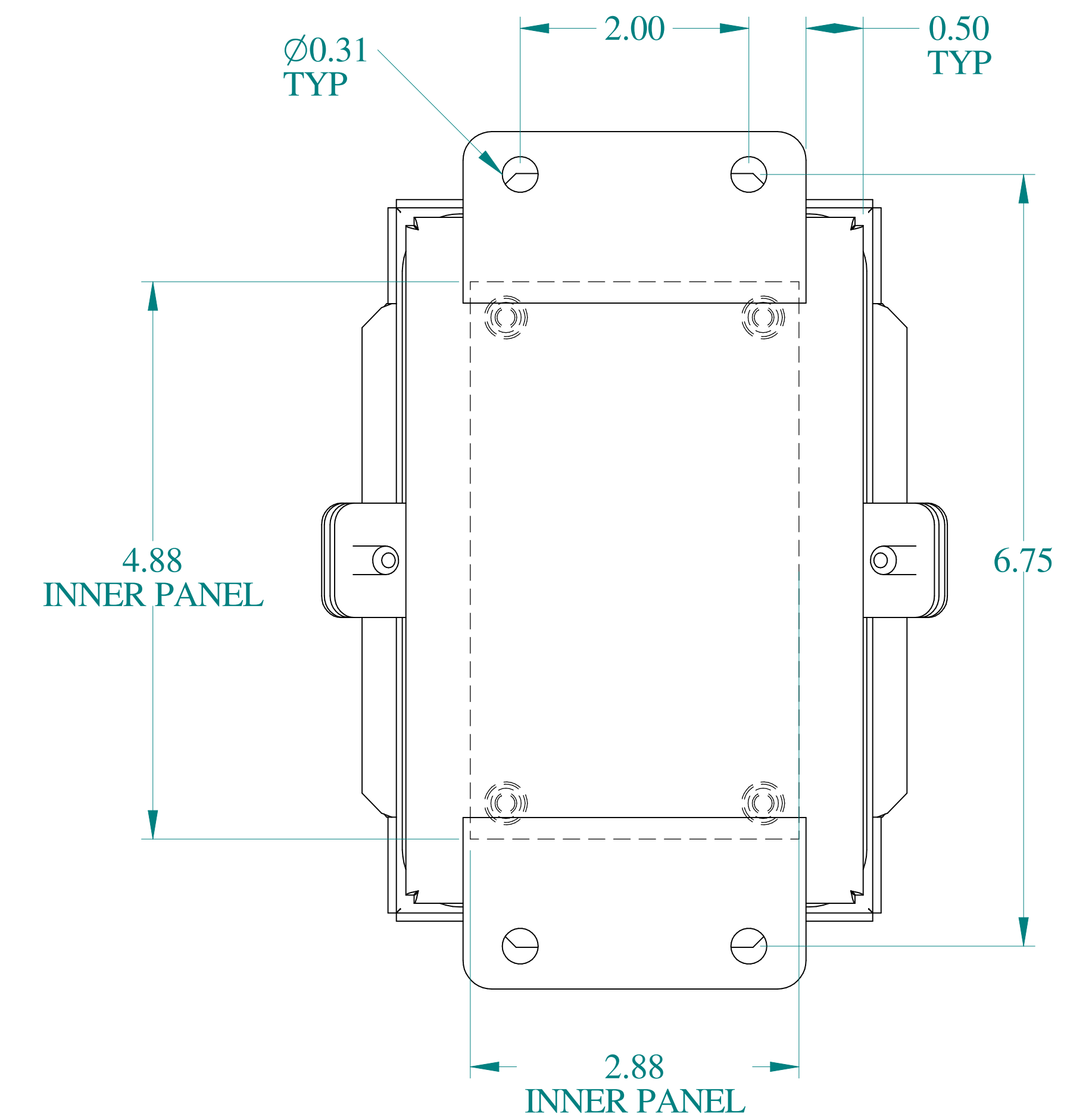
BACK VIEW
