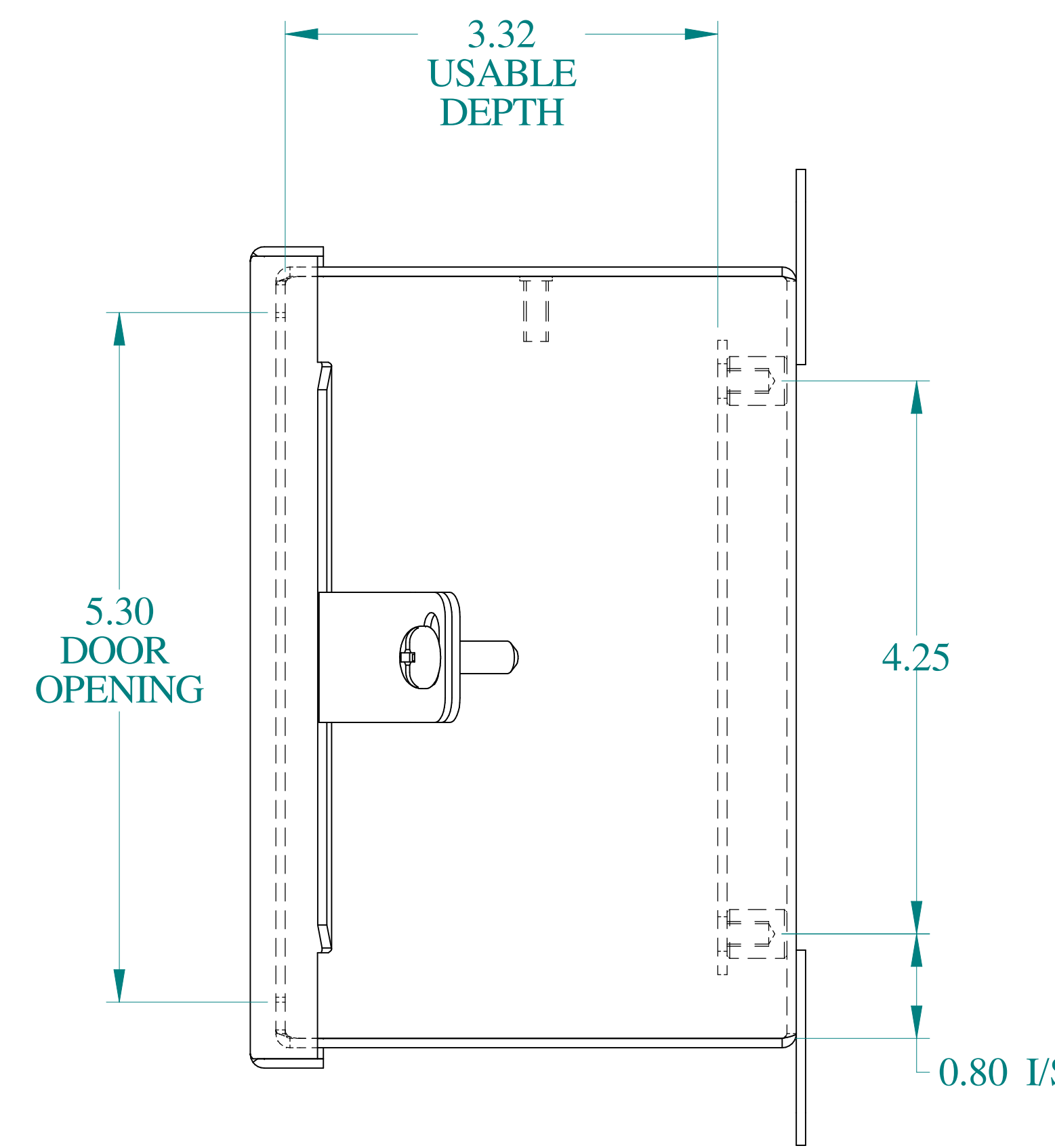
SIDE VIEW
