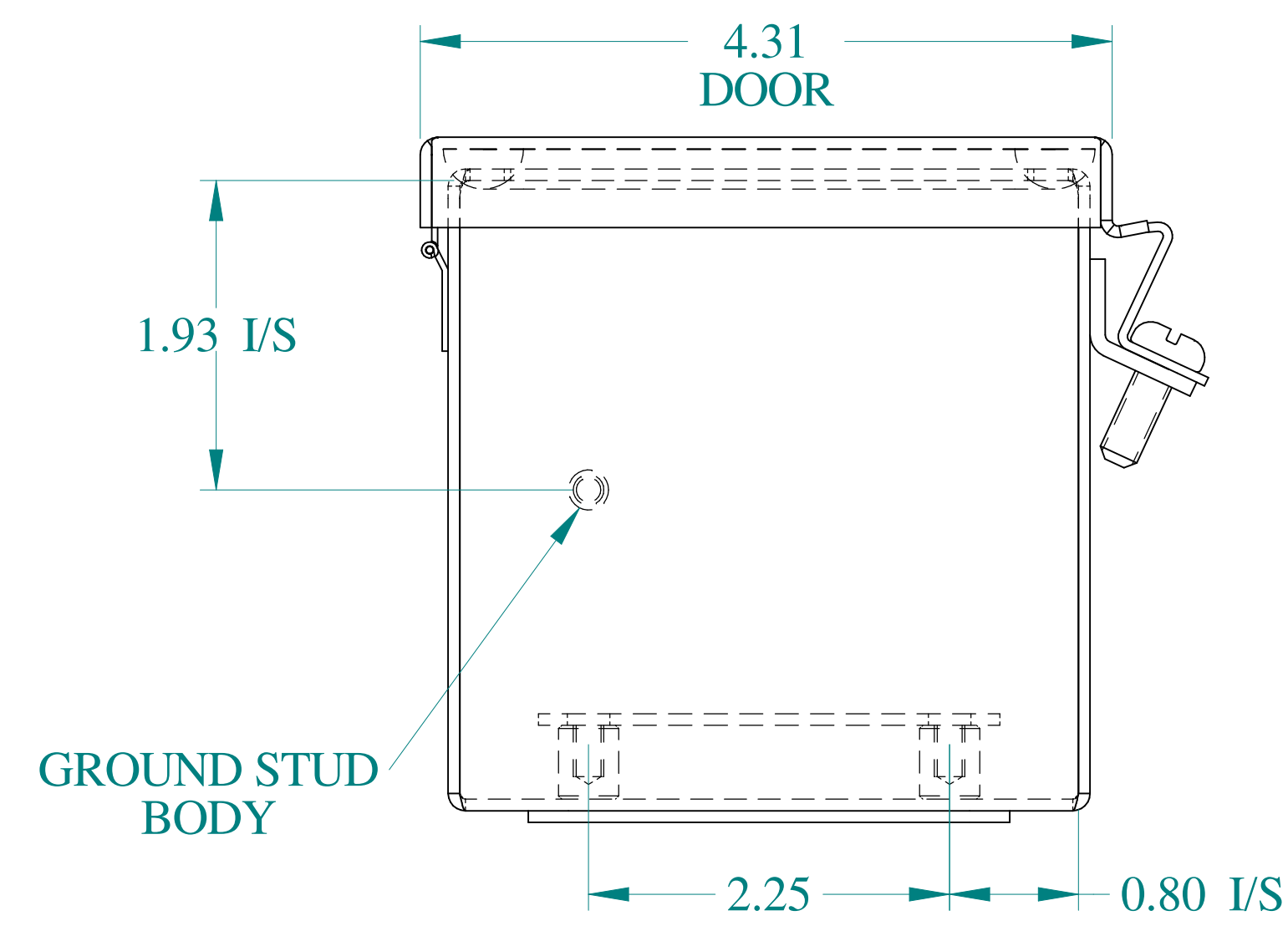
BOTTOM VIEW
