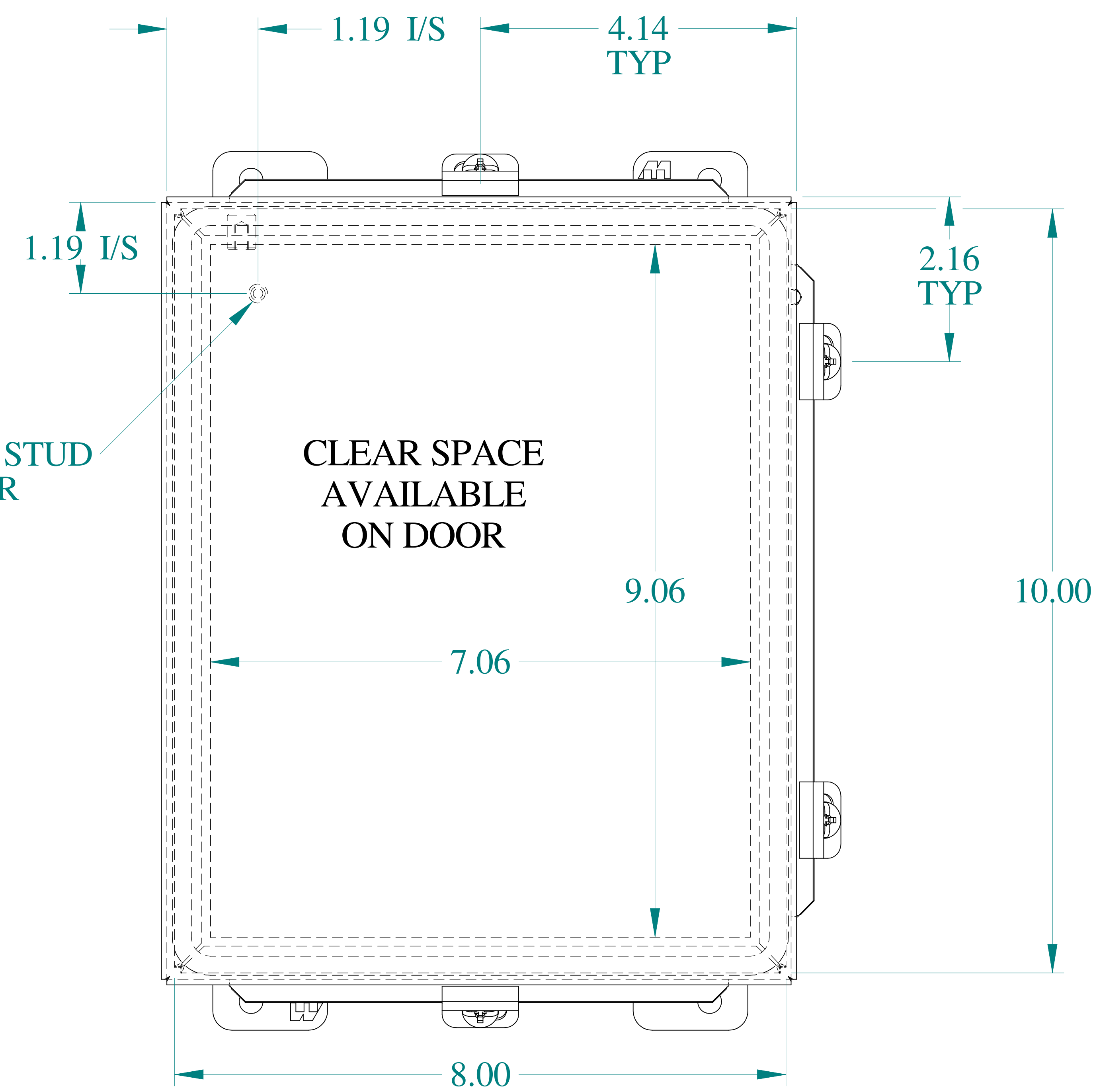
FRONT VIEW
