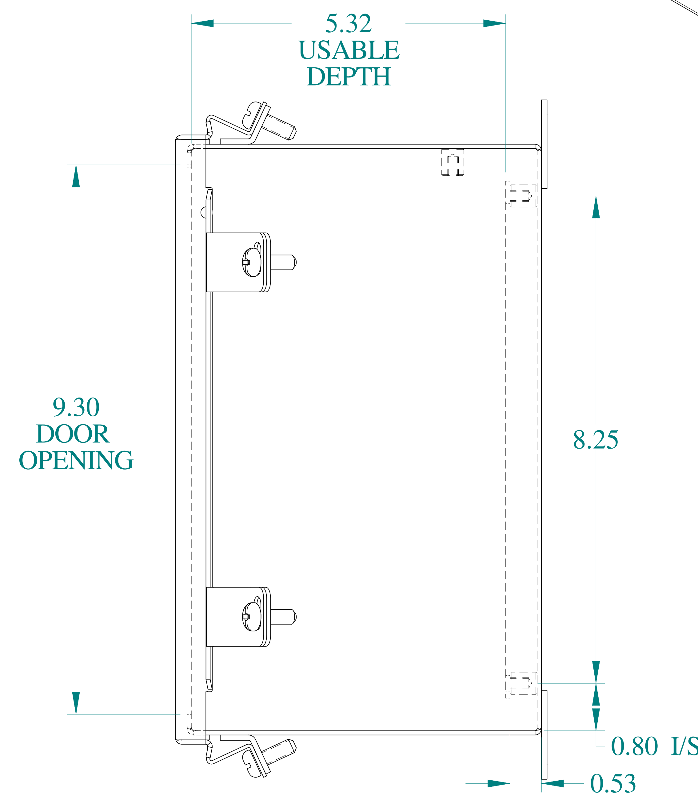
SIDE VIEW
