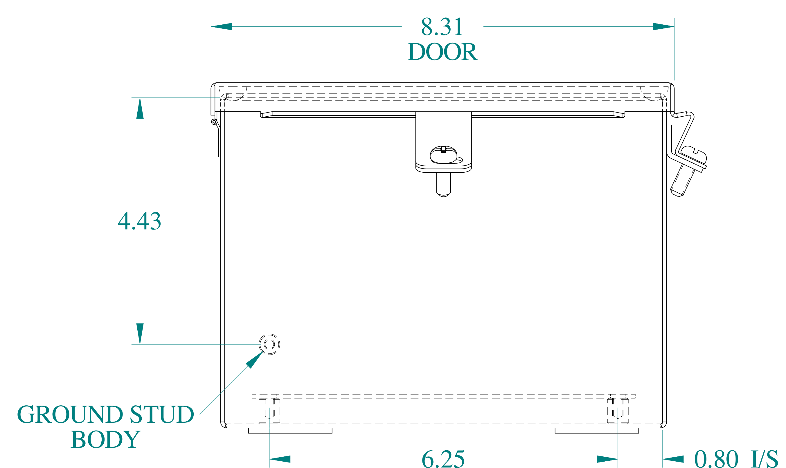
BOTTOM VIEW
