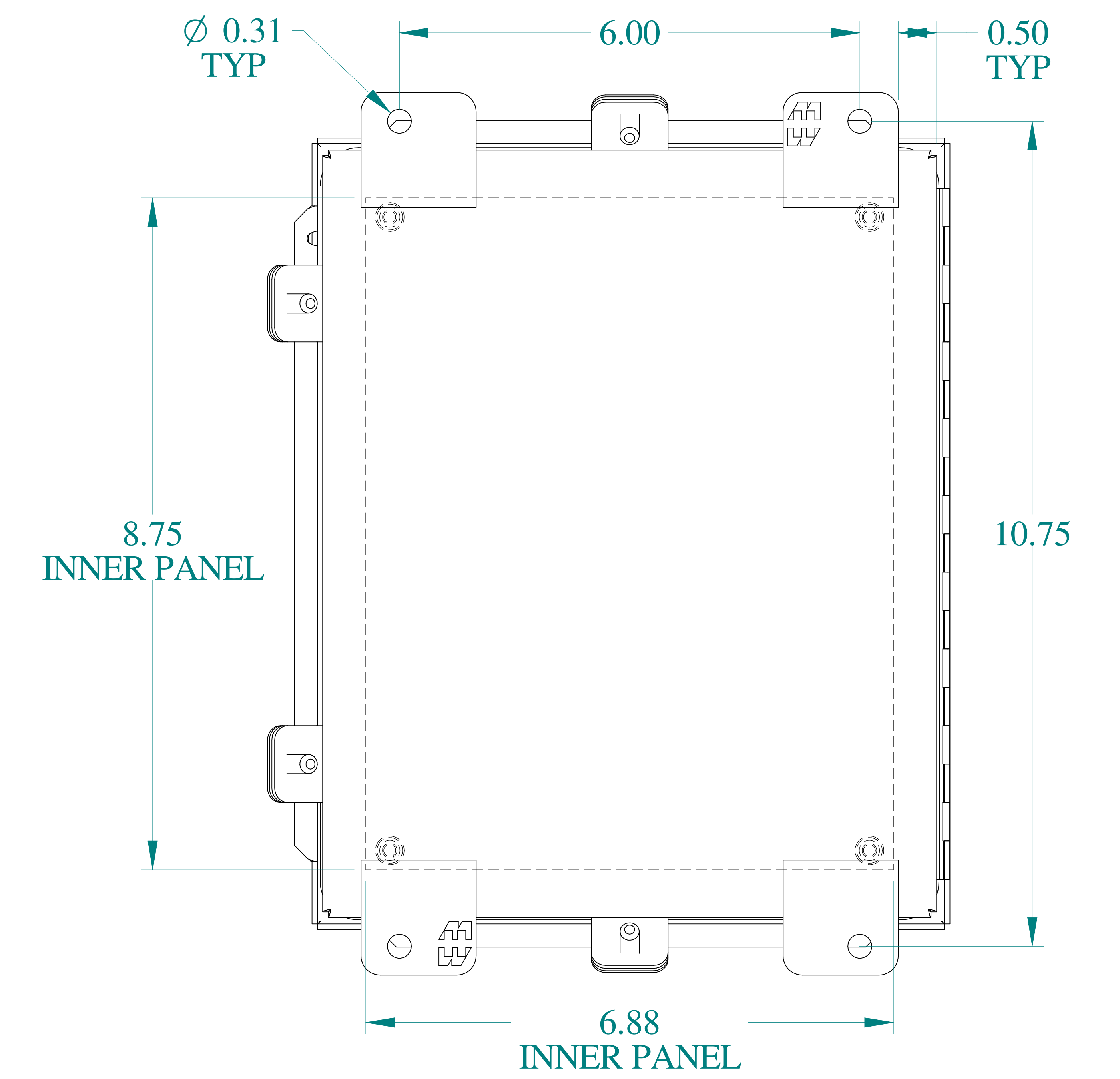
BACK VIEW
