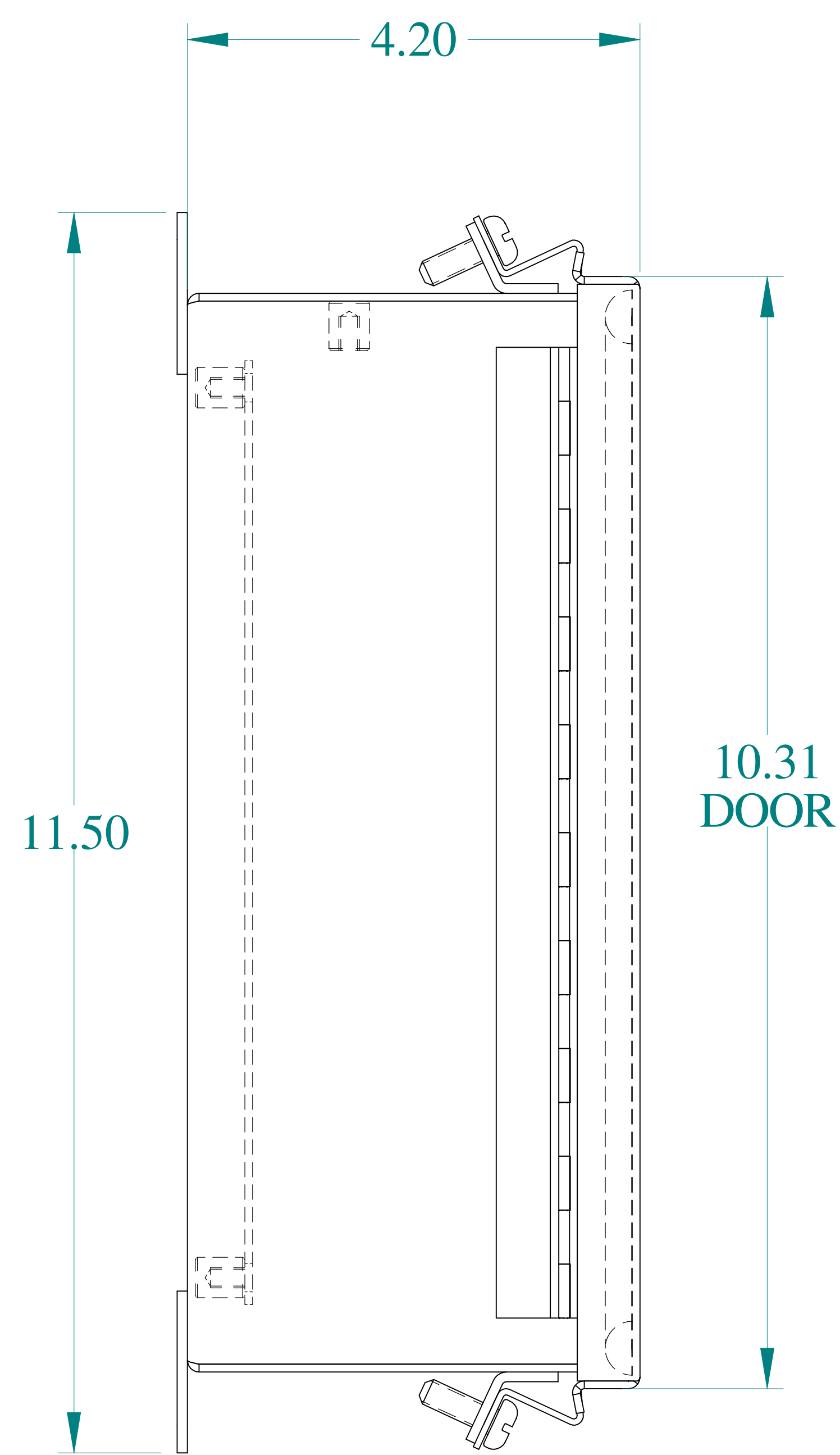
SIDE VIEW
