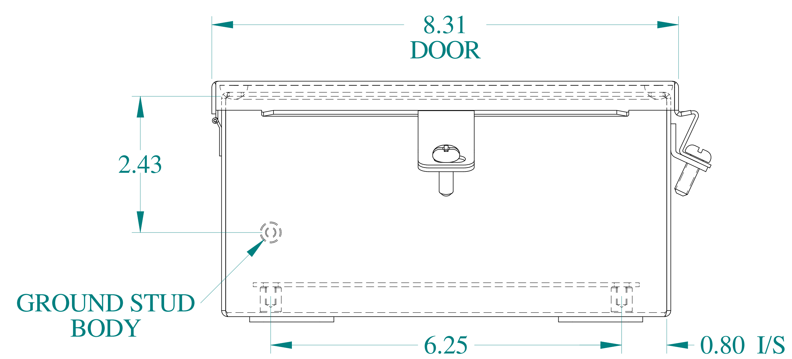
BOTTOM VIEW
