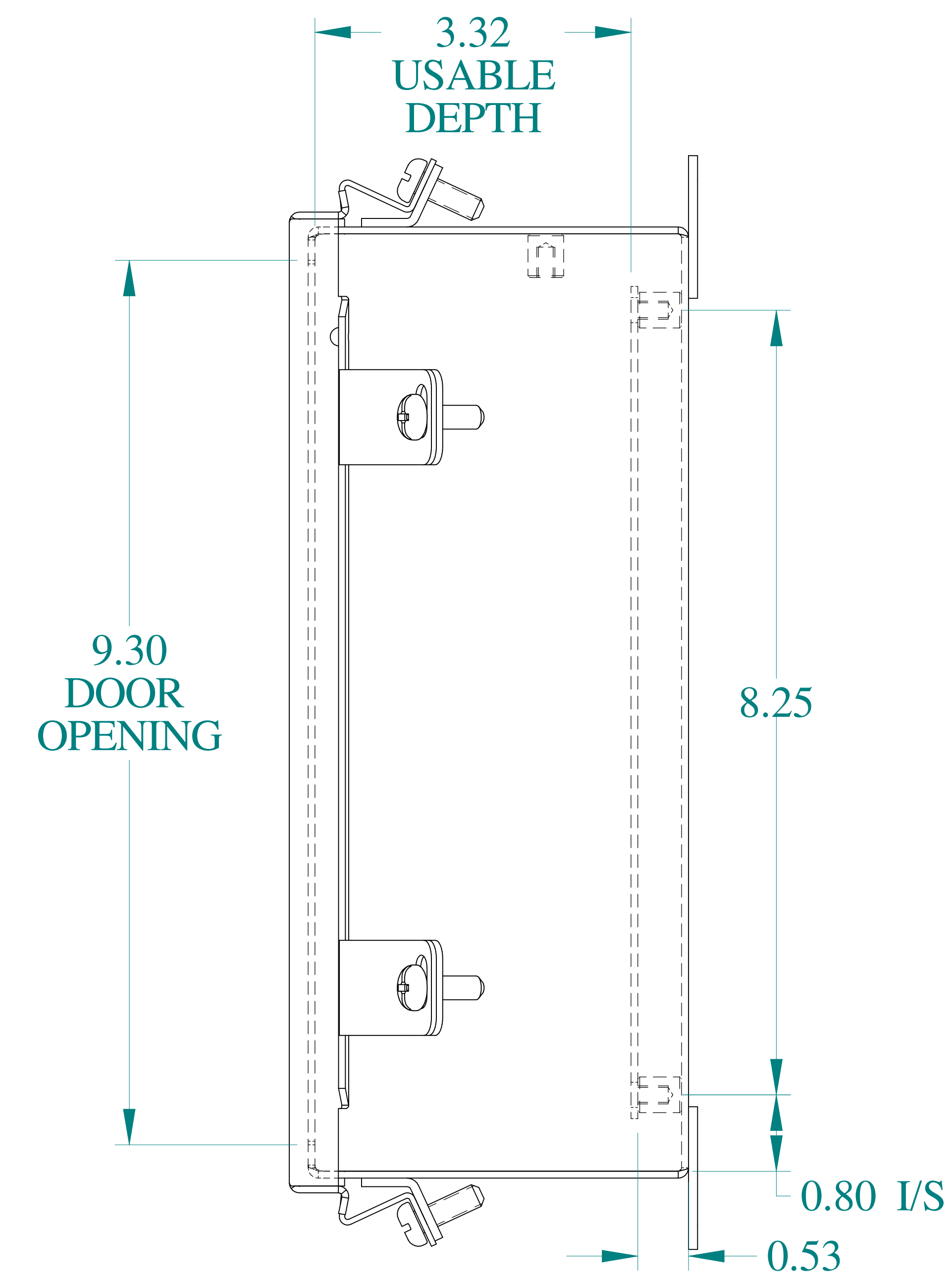
SIDE VIEW
