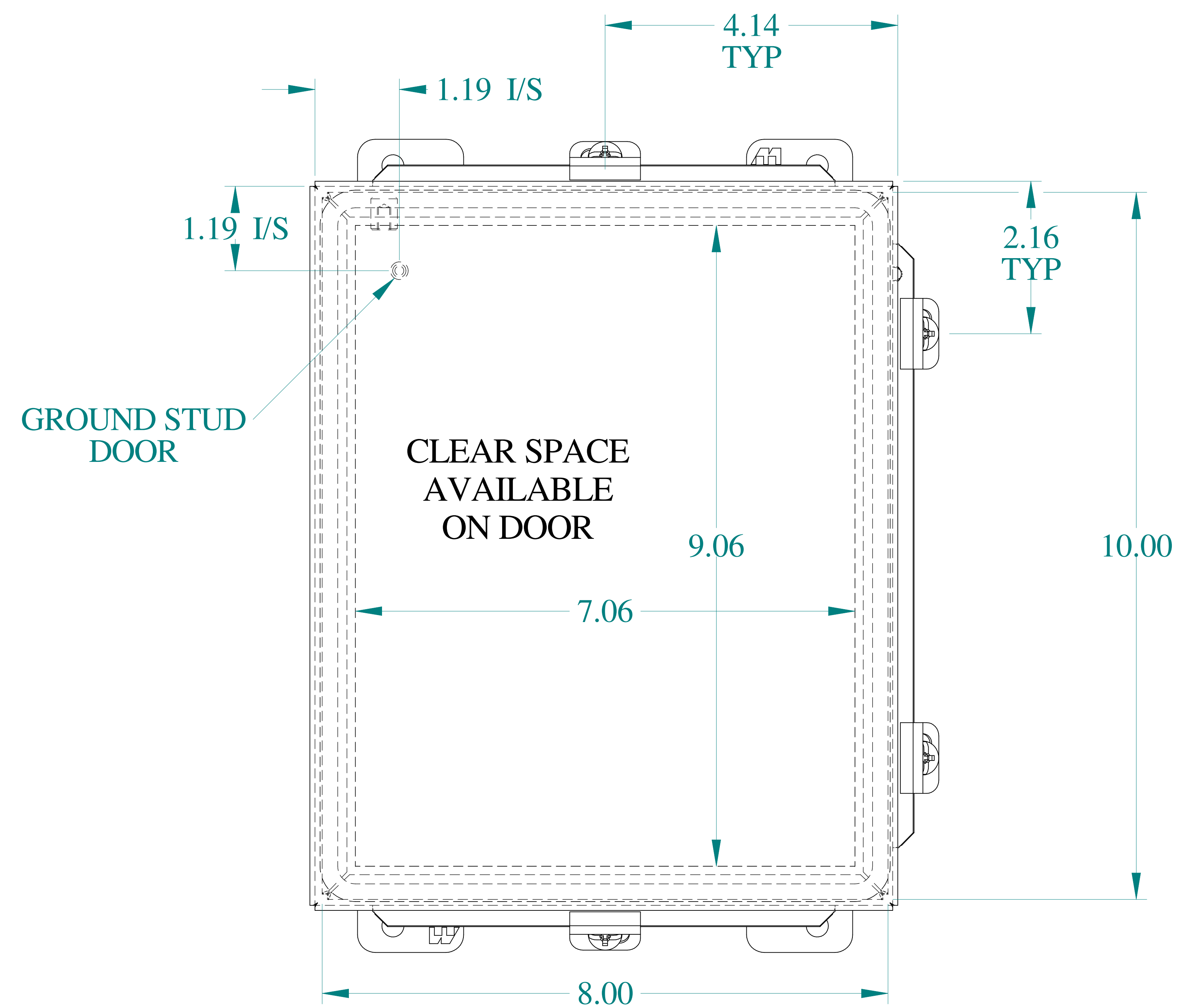
FRONT VIEW
