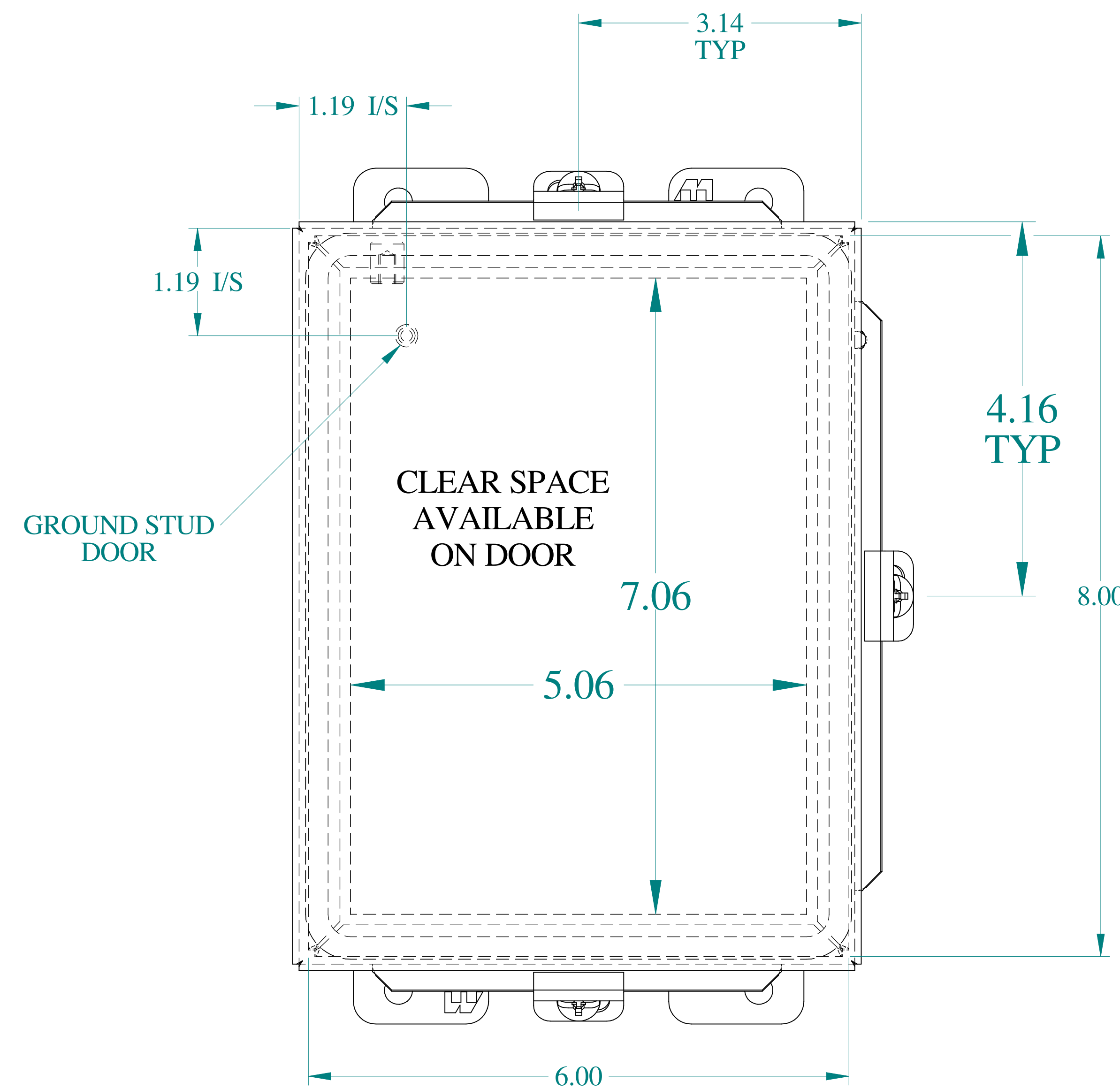
FRONT VIEW
