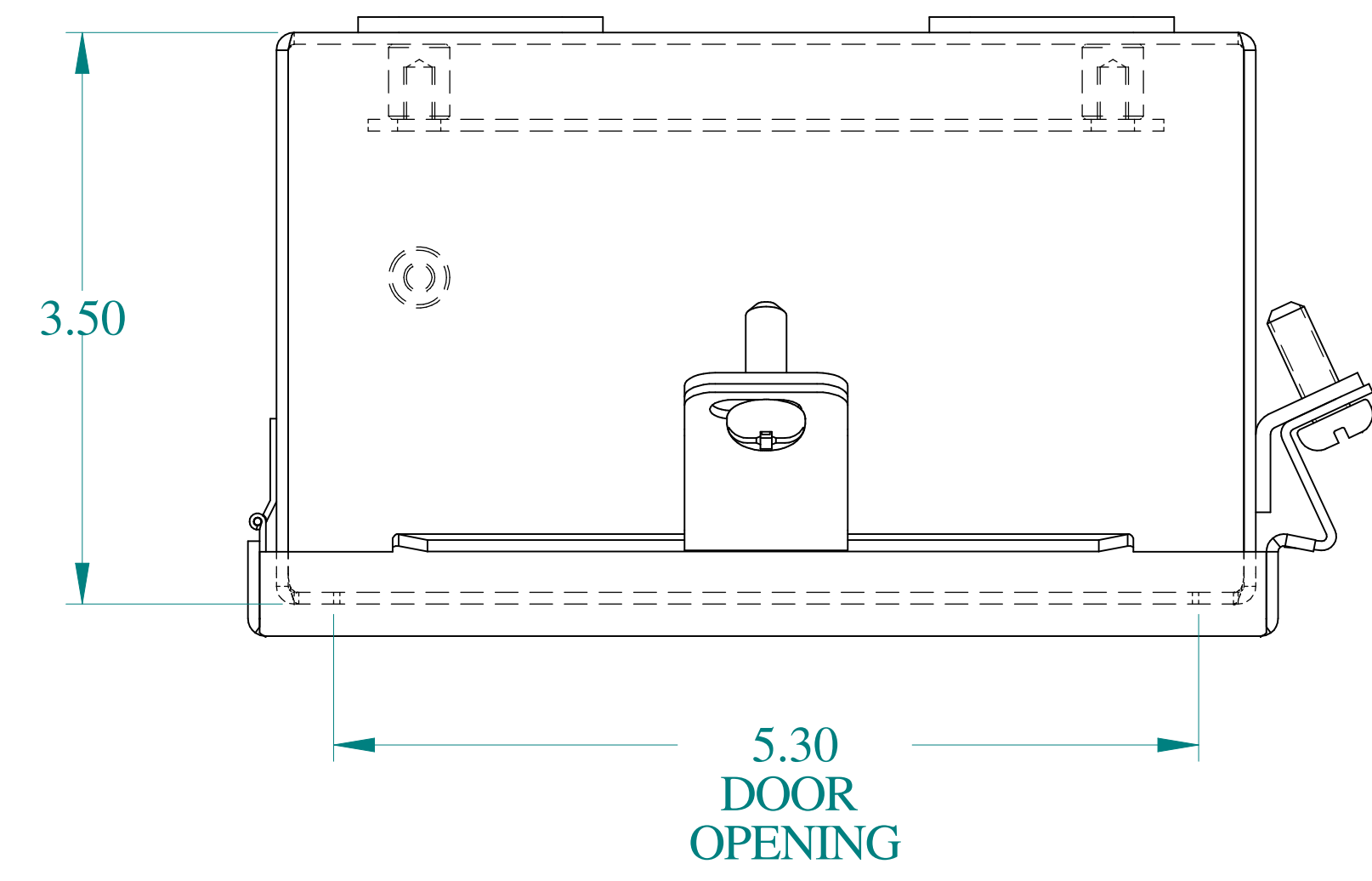
TOP VIEW
