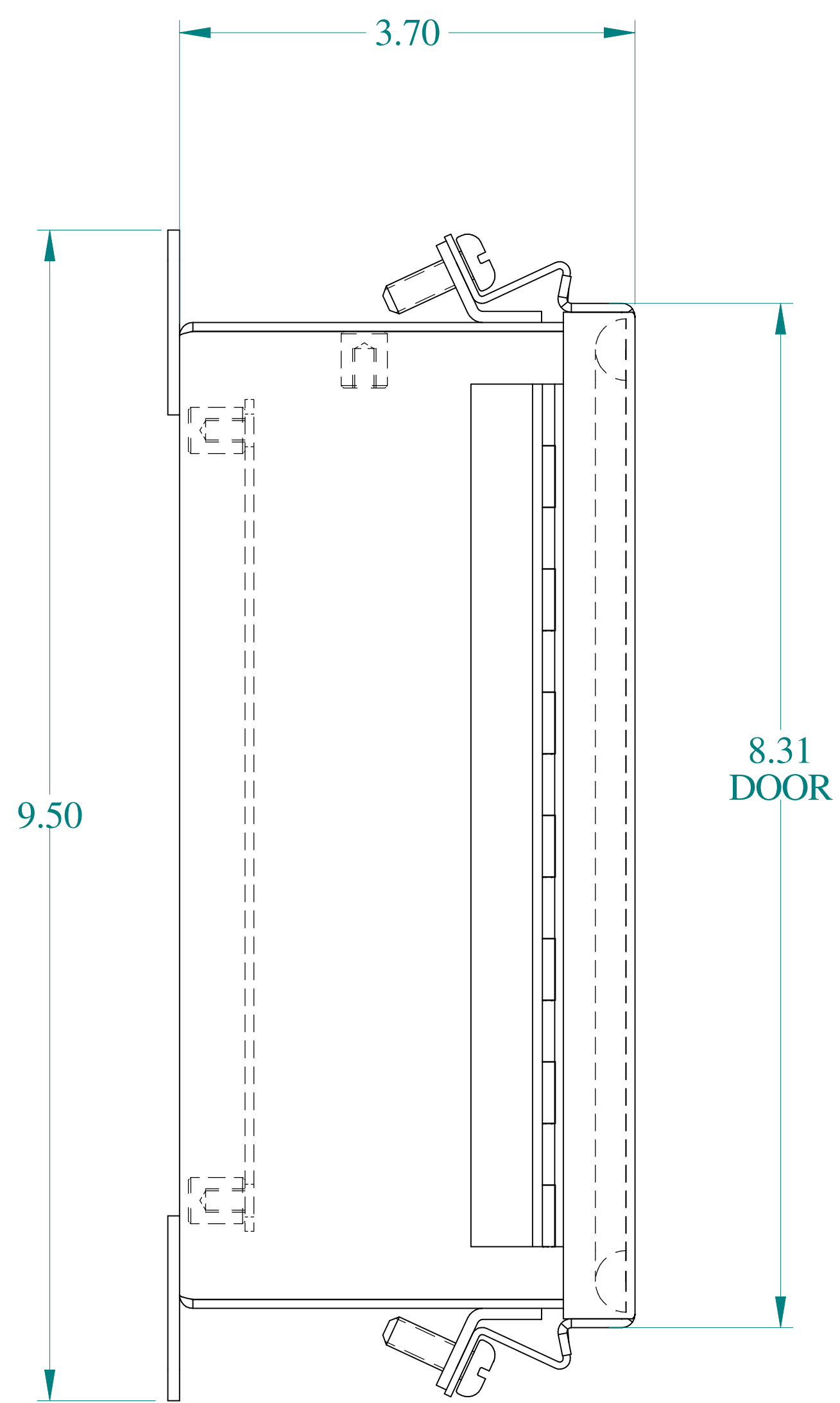
SIDE VIEW
