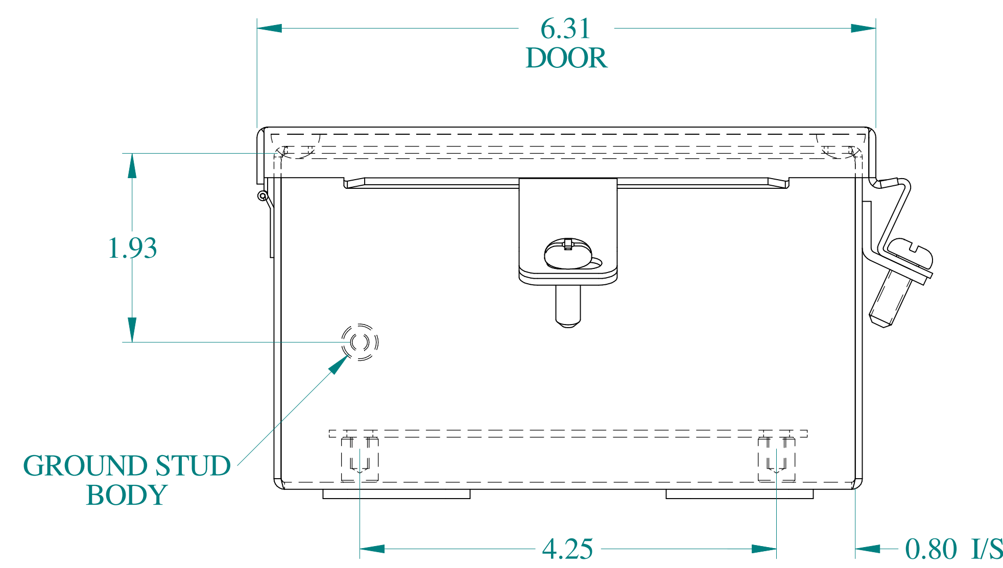
BOTTOM VIEW
