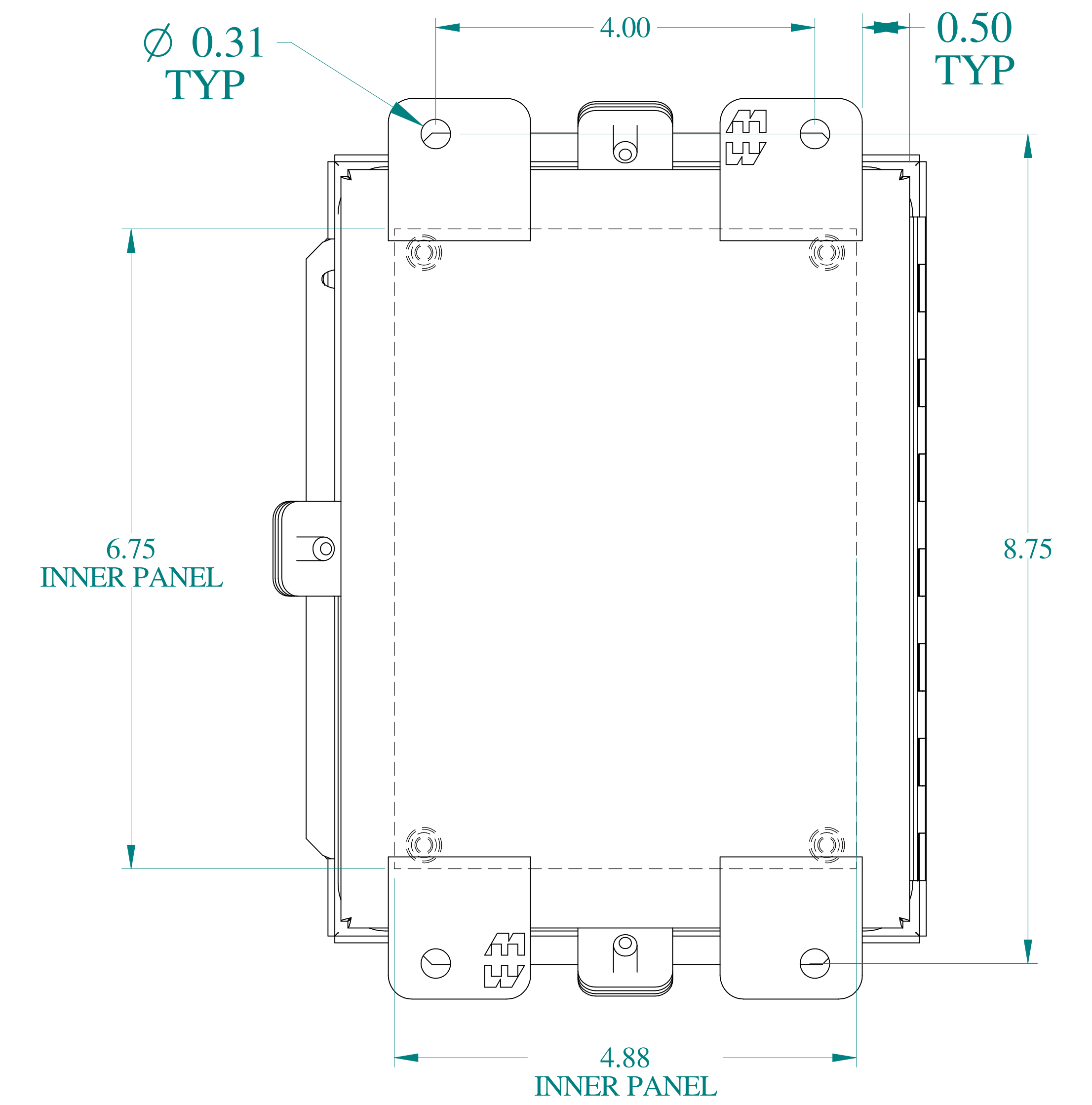
BACK VIEW
