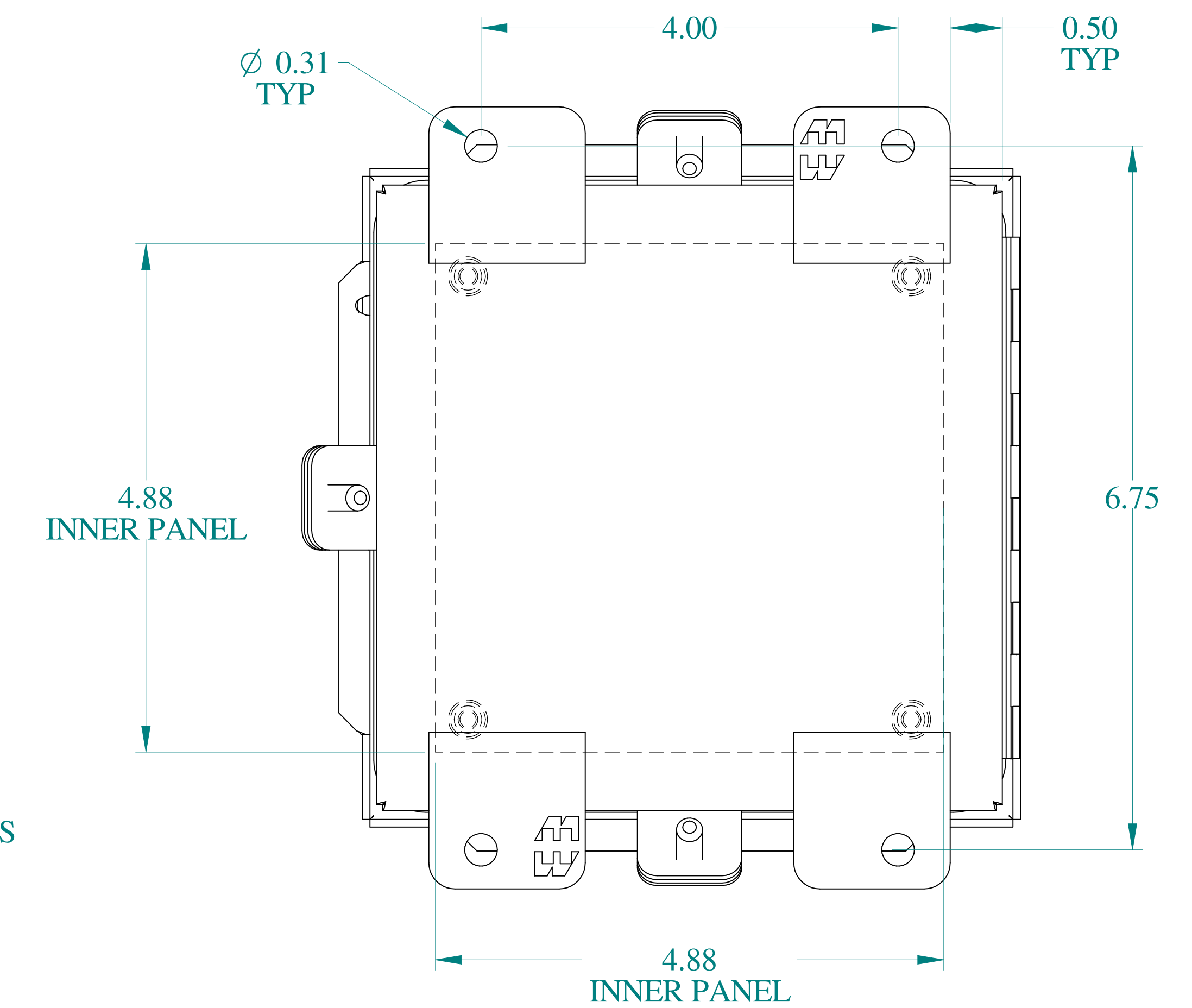
BACK VIEW
