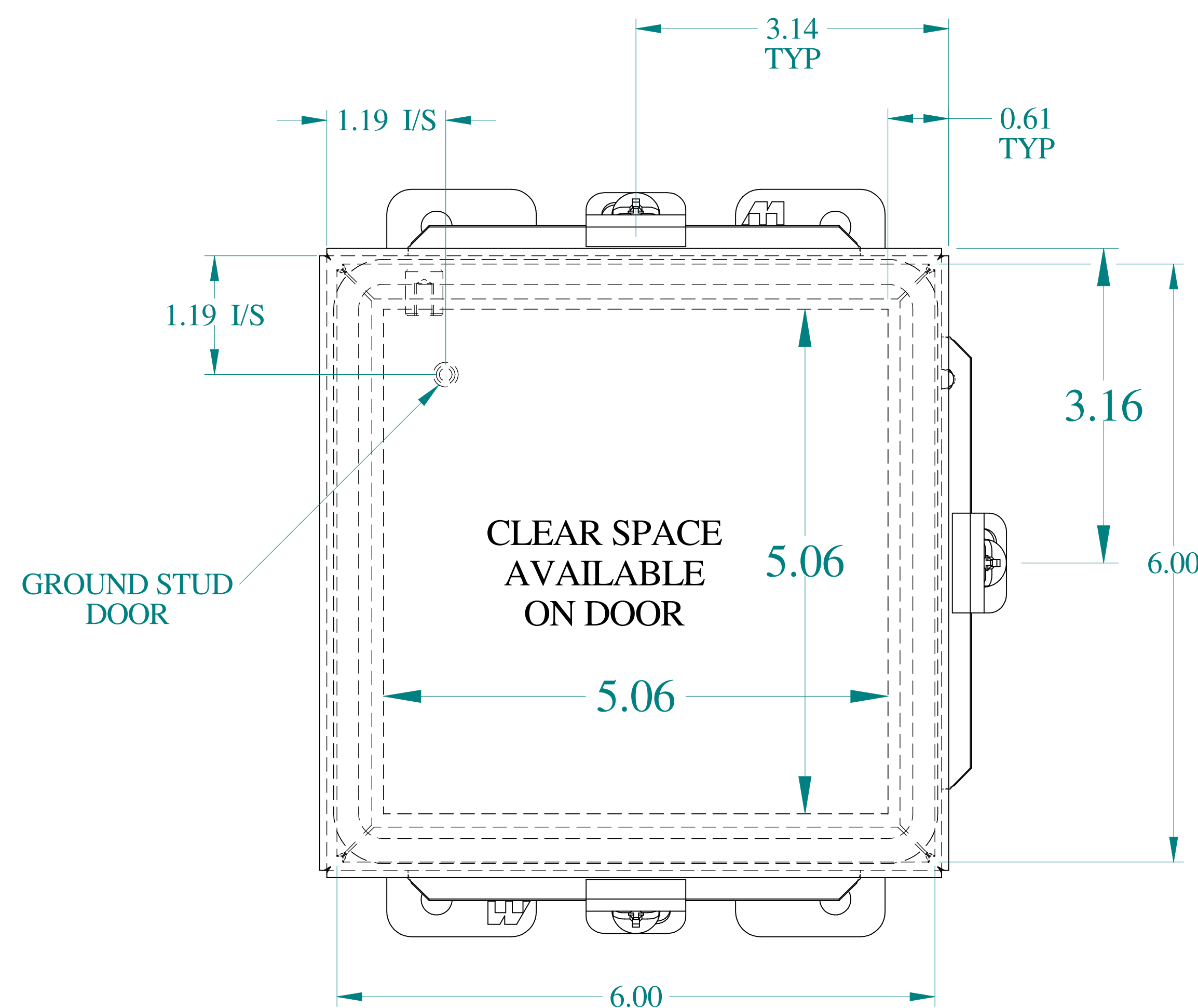
FRONT VIEW
