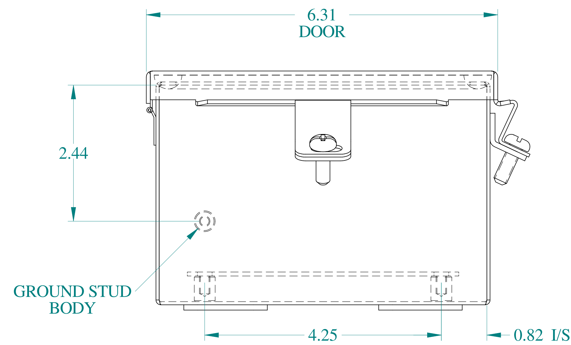
BOTTOM VIEW
