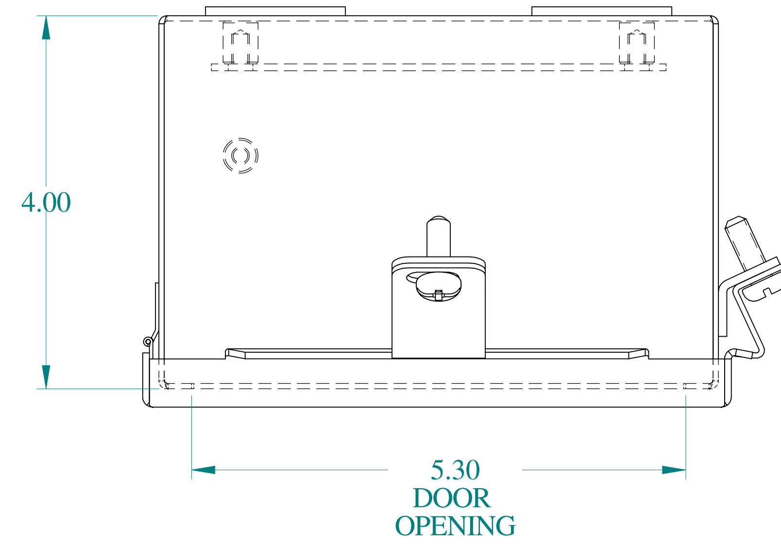
TOP VIEW
