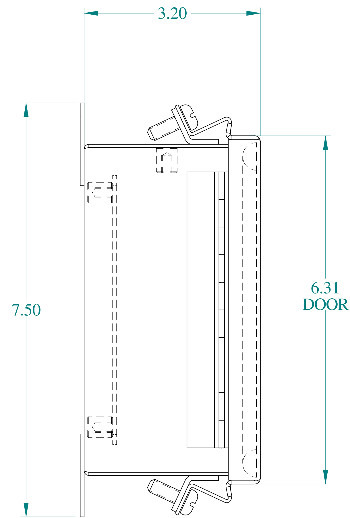
SIDE VIEW
