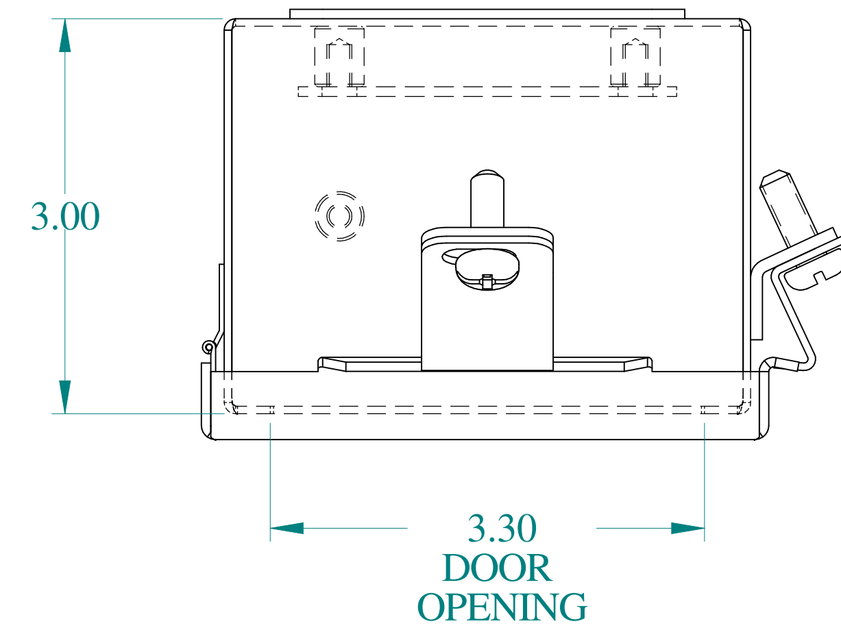
TOP VIEW
