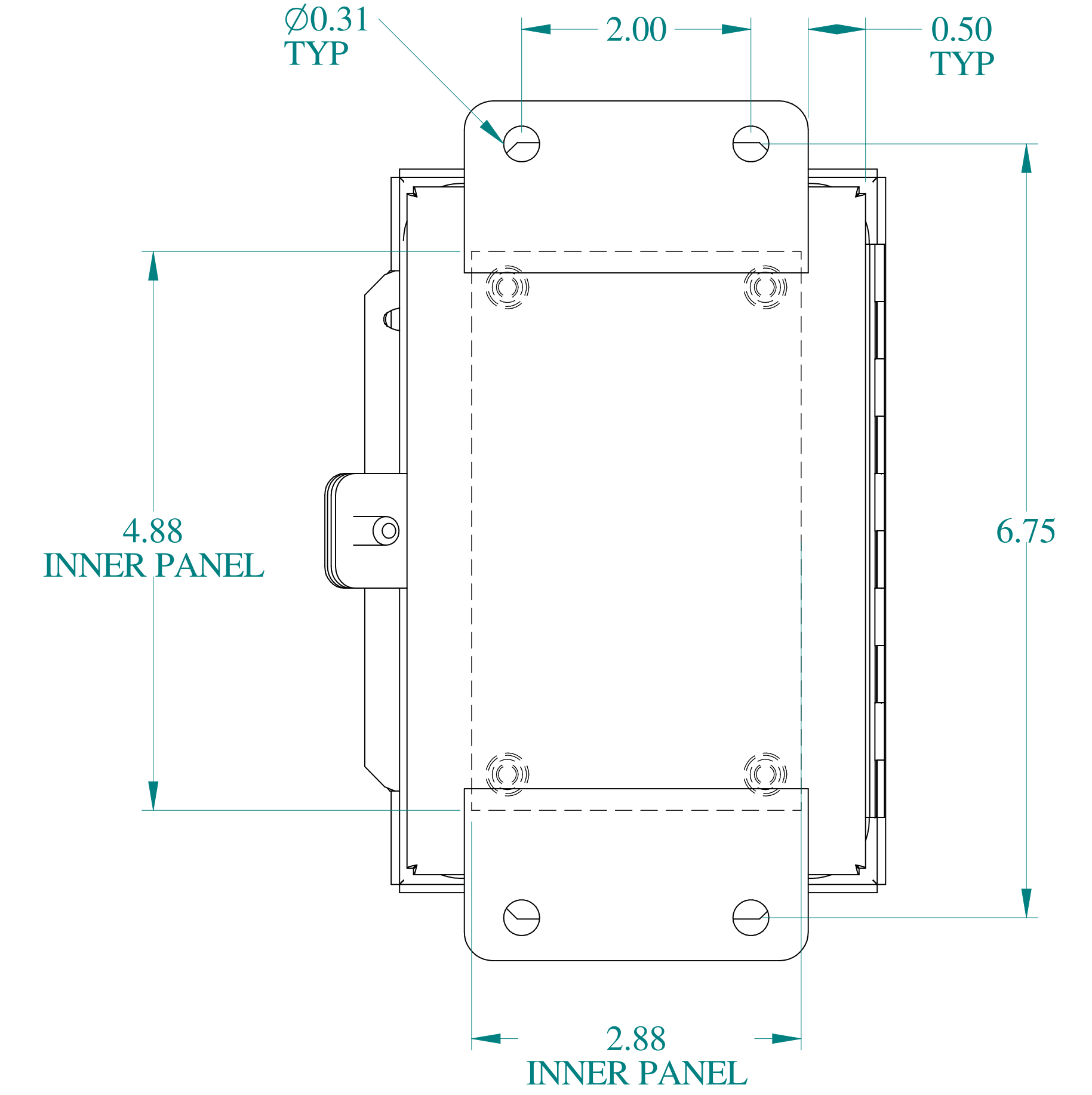
BACK VIEW
