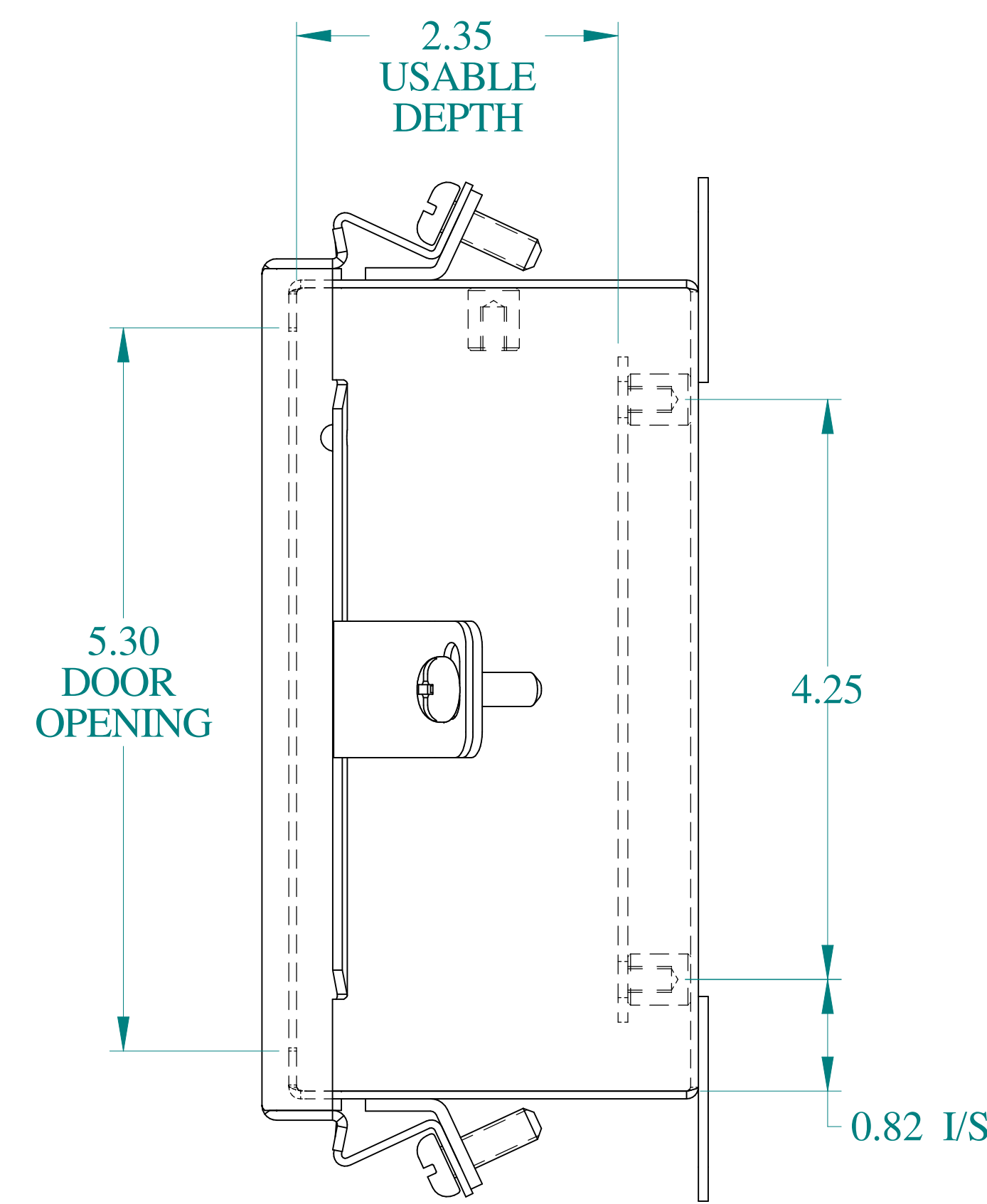
SIDE VIEW
