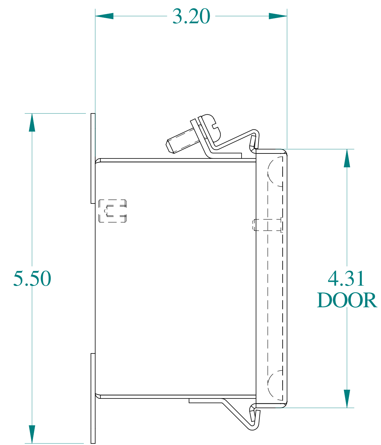
SIDE VIEW
