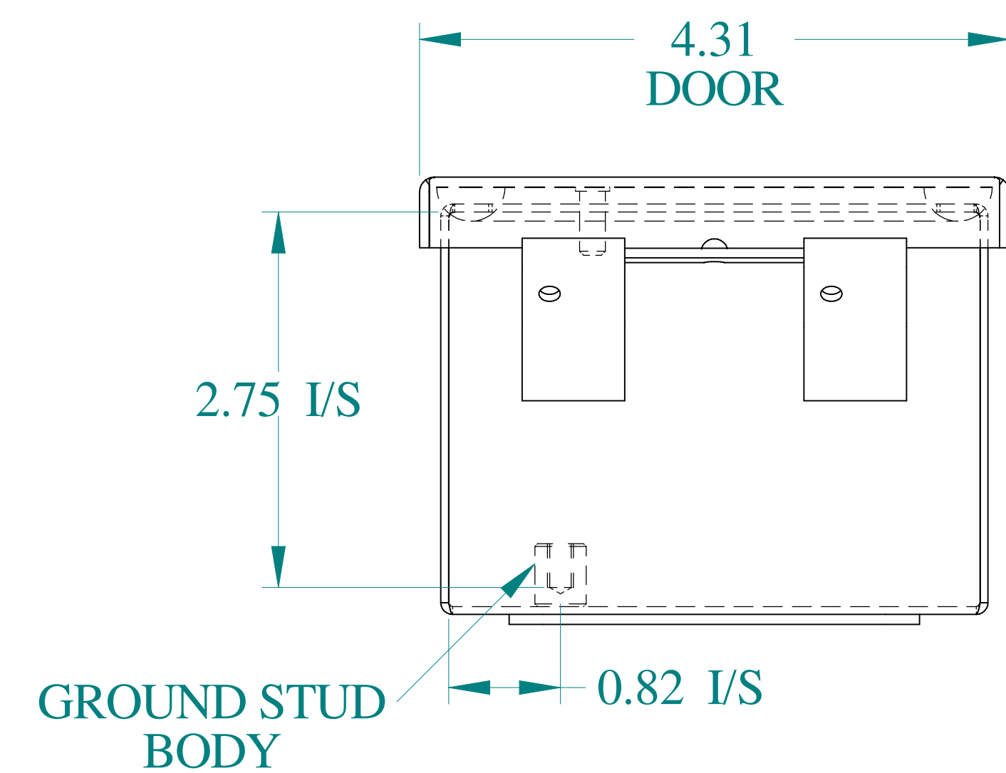
BOTTOM VIEW
