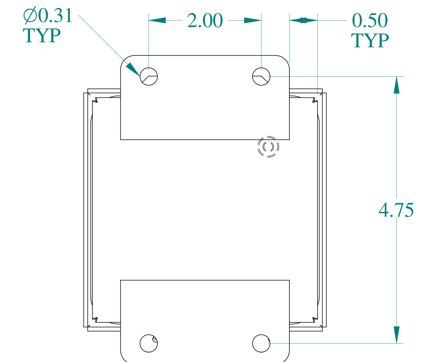
BACK VIEW
