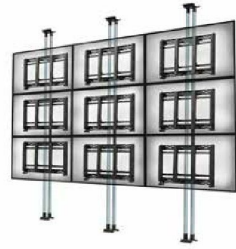
3x3 LANDSCAPE VIDEO WALL Shown in Modular Series Dual Pole Floor-to-Ceiling configuration (SmartMount® Full Service Video Wall Mount with Quick Release, DS-VW765-LQR, required)
