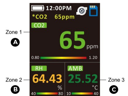
1.1 Main LCD Display
