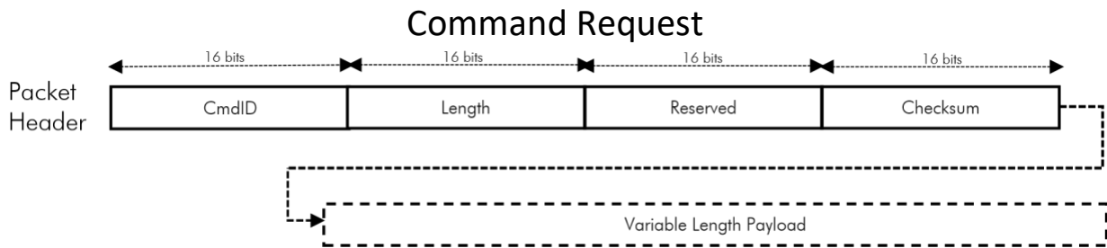
Figure 1: Request Packet Structure
