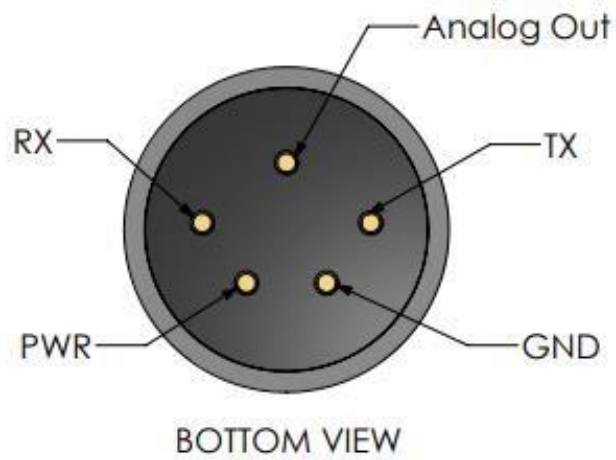
Figure 11: A2L IS electrical pin configuration
