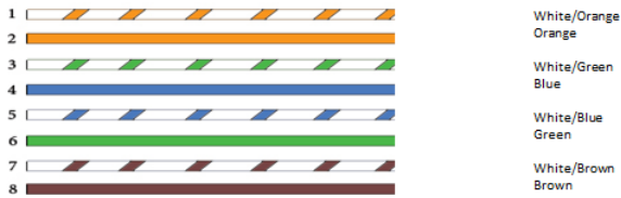
T568B Standard
