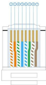
T568B Standard
