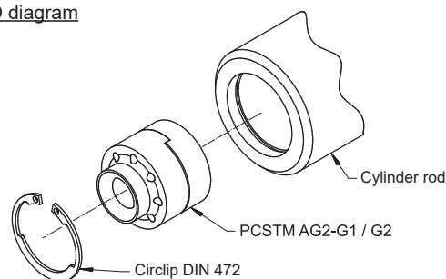
ISO diagram
