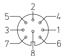
CONN-D8-8M
