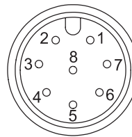
CONN-M12-8M
