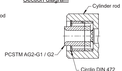
Section diagram
