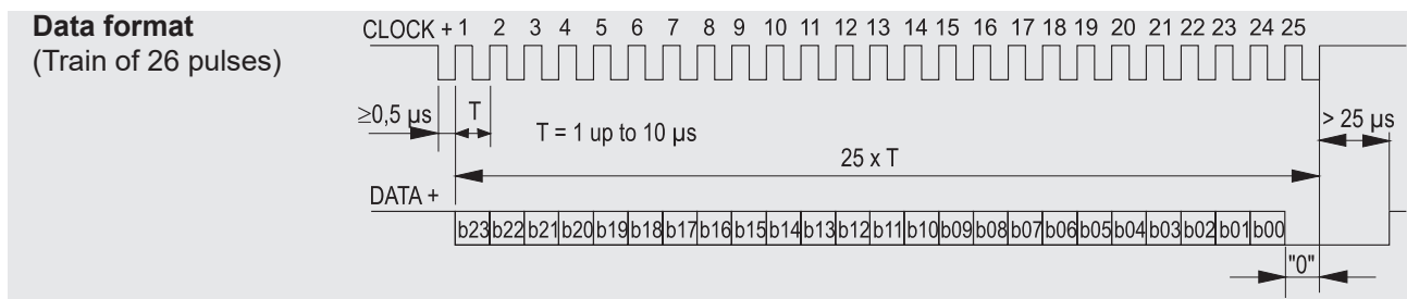
Signal diagram
