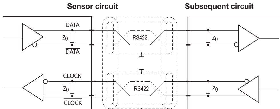
Signal diagram
