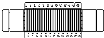
Blades (1.0mm x 10.0mm) CAT# MEE1-10-26 Mount, CAT# MEF26-10
