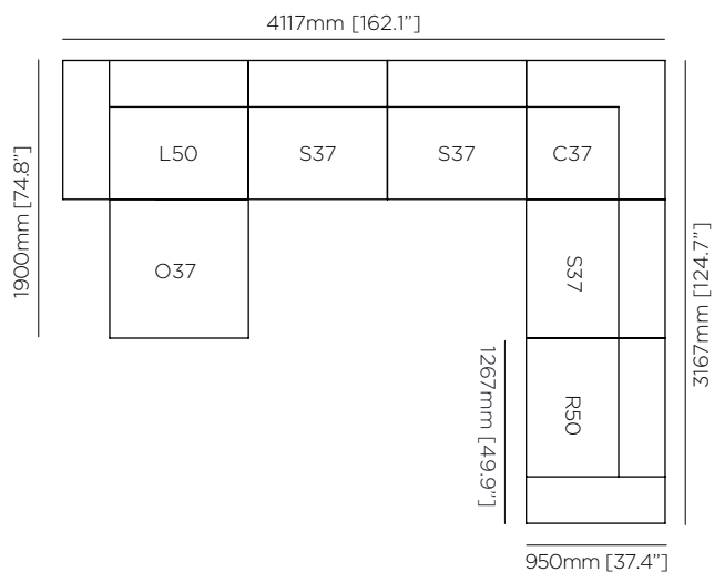
Modular 7 U-Sofa Chaise Sectional BLD.MS.CON.USC7
