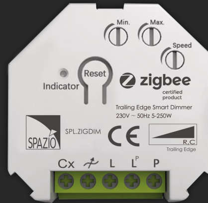
ZIGBEE DIMMER INCLUDES TOUCHLINK
