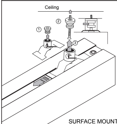
SURFACE MOUNT (NEW EXTRUSION)
