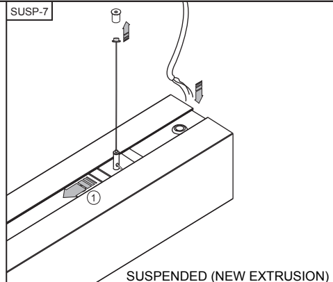
SUSPENDED (NEW EXTRUSION)
