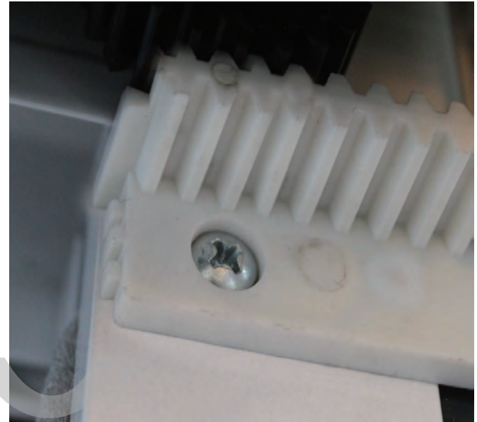
Installation of Mecahnism 2 (Top mounting)
