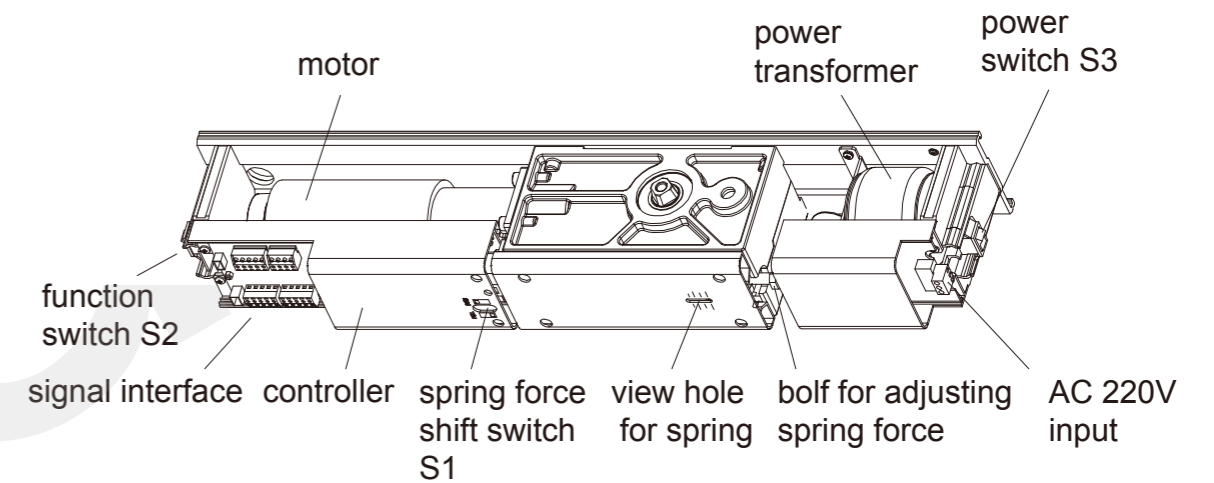
Drive device
