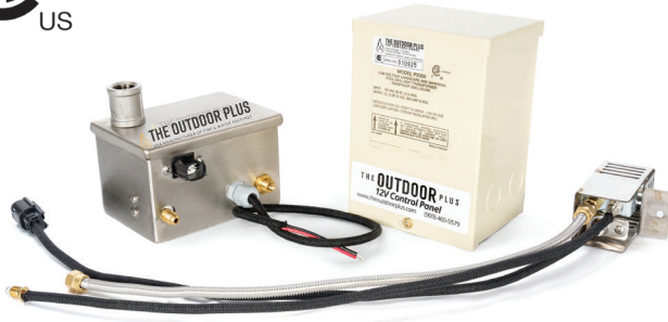
12V ELECTRONIC IGNITION SYSTEM
