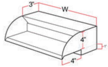
Smooth Flow Radius Scupper
