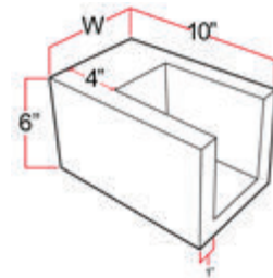
U-Shaped Scupper
