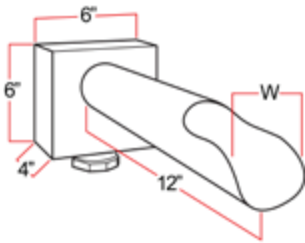
Cannon Scupper
