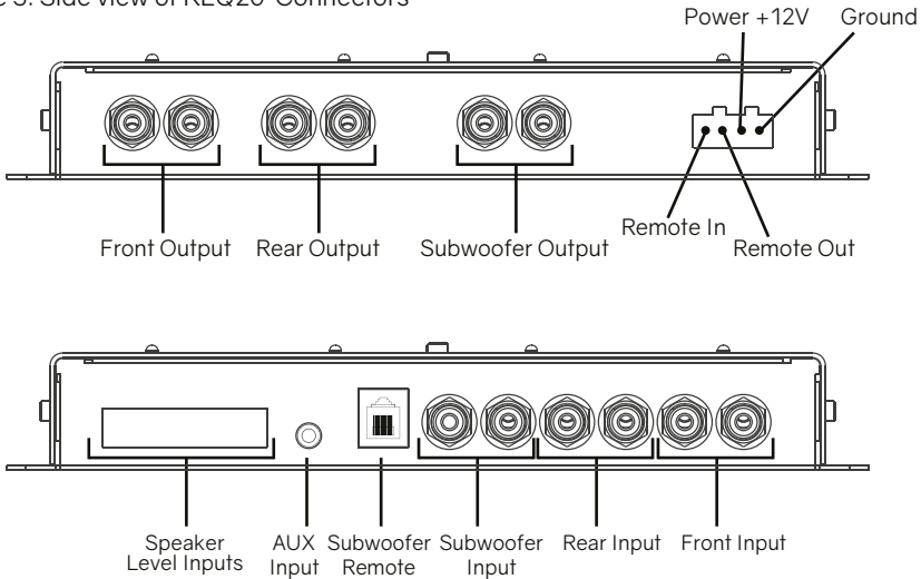
Figure 3: Side view of KEQ20 Connectors
